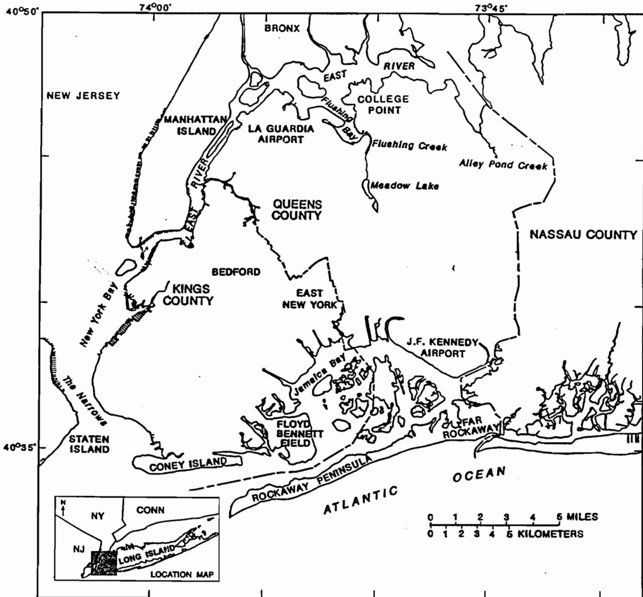
Figure 1. Location of Kings, Queens, and western Nassau County study area, Long Island, N.Y.
