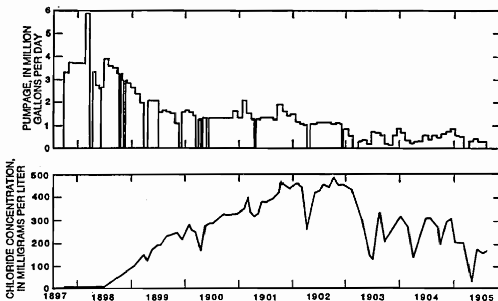
Figure 7. Average chloride concentration and total pumpage from eight driven wells at the Shetucket pumping station, 1897-1905. (From Spear, 1912, sheet 12.)
