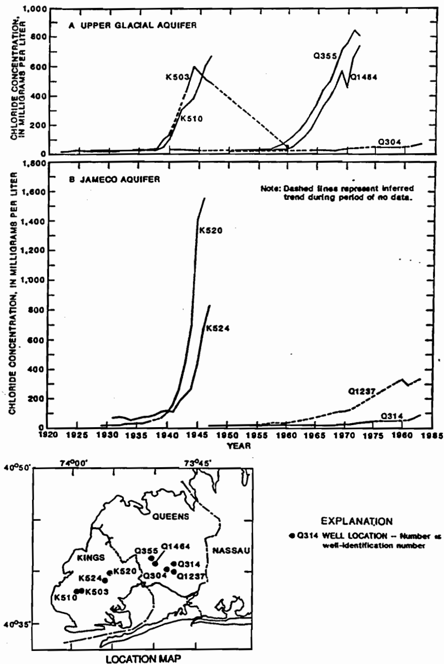
Figure 8. Chloride concentration in water from selected wells in Kings and Queens Counties: (A) Wells screened in the upper glacial aquifer. (B) Wells screened in the Jameco aquifer. (Data from U.S. Geological Survey files, Lusczynski, 1952, and selected annual reports of the Bureau of Water Supply, City of New York.)
