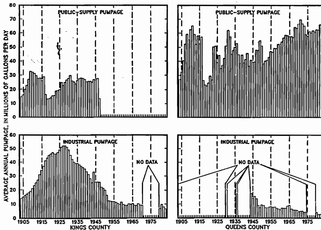
Figure 4. Annual average pumpage for industrial and public supply in Kings and Queens Counties, 1904-83. (Compiled from Johnson and Waterman, 1952; Thompson and Leggette, 1936, Suter, 1937, and New York State Department of Environmental Conservation.)
