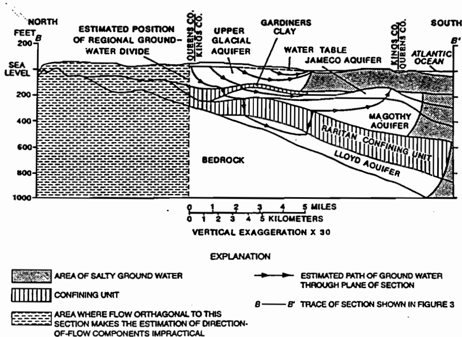
Figure 2. Estimated flow patterns along Section B-B' under predevelopment conditions. (Location is shown in fig. 3.)
