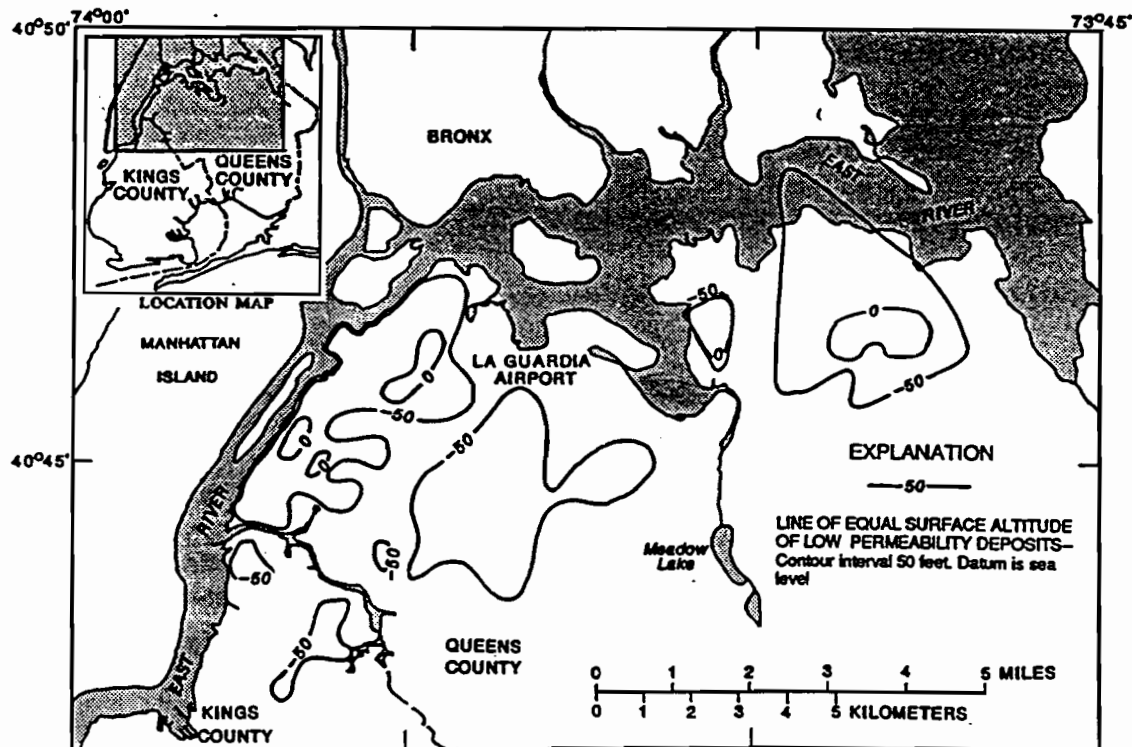
Figure 10. Upper surface altitude of deposits with low permeability at base of water-table aquifer in northern Kings and Queens Counties.
