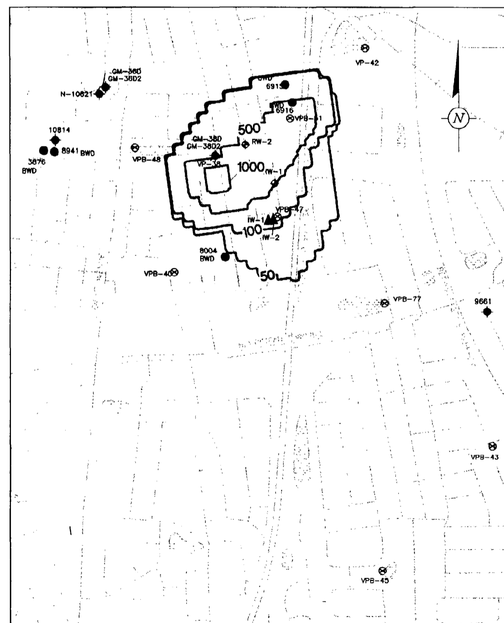
FIGURE 4: PRESENT DAY TVOC CONCENTRATIONS IN MODEL LAYER 5 PROPOSED 2-WELL REMEDIAL SYSTEM AT THE GM38 AREA SCALE: 1" = 80'
