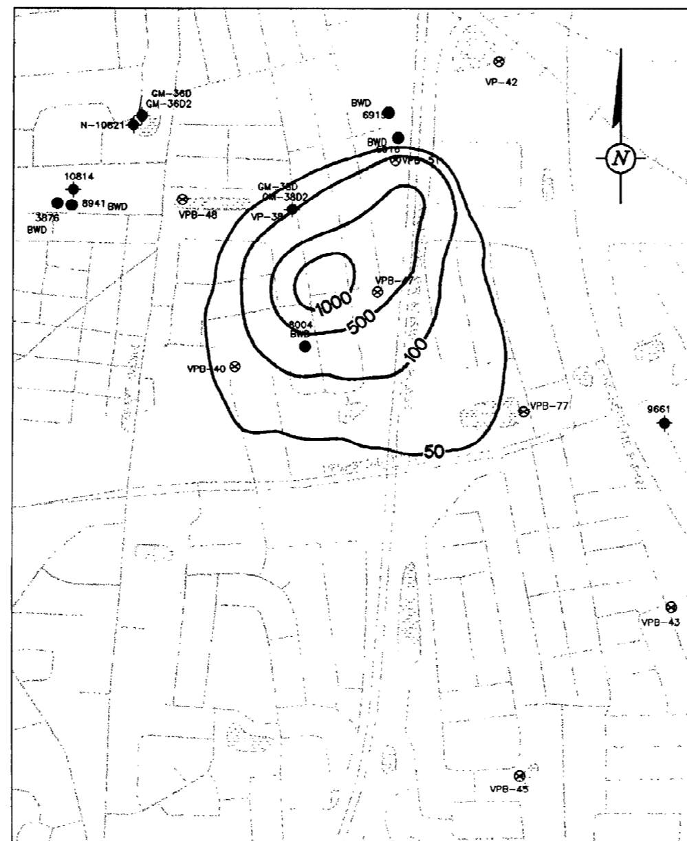
FIGURE 14: TVOC CONCENTRATIONS IN MODEL LAYER 6 AFTER 10 YEARS WITH NO REMEDIAL ACTION AT THE GM38 AREA SCALE: 1" = 80'
