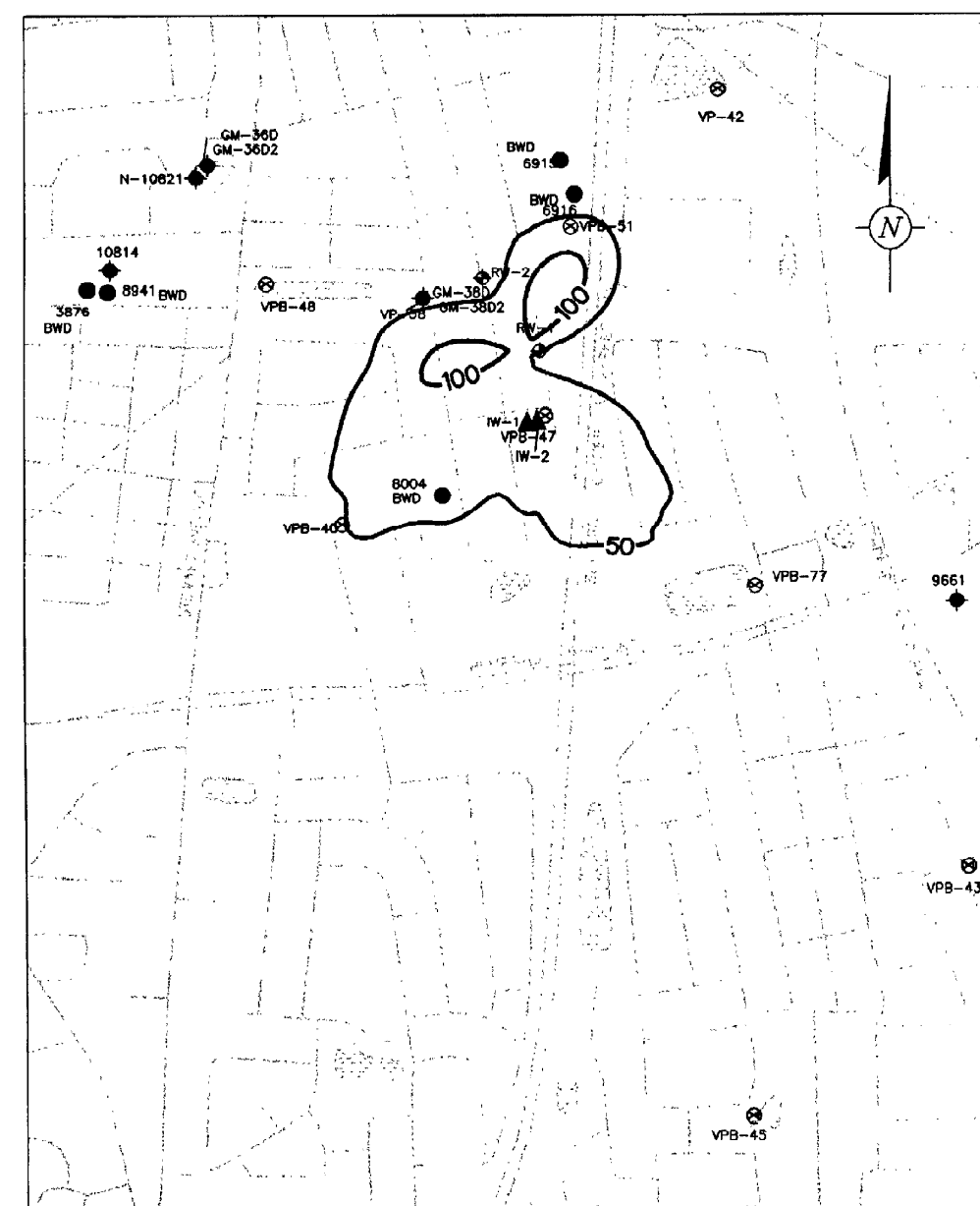
FIGURE 11: TVOC CONCENTRATIONS IN MODEL LAYER 6 AT THE GM38 AREA WITH THE PROPOSED 2-WELL REMEDIAL SYSTEM PUMPING FOR 5 YEARS SCALE: 1" = 80'
