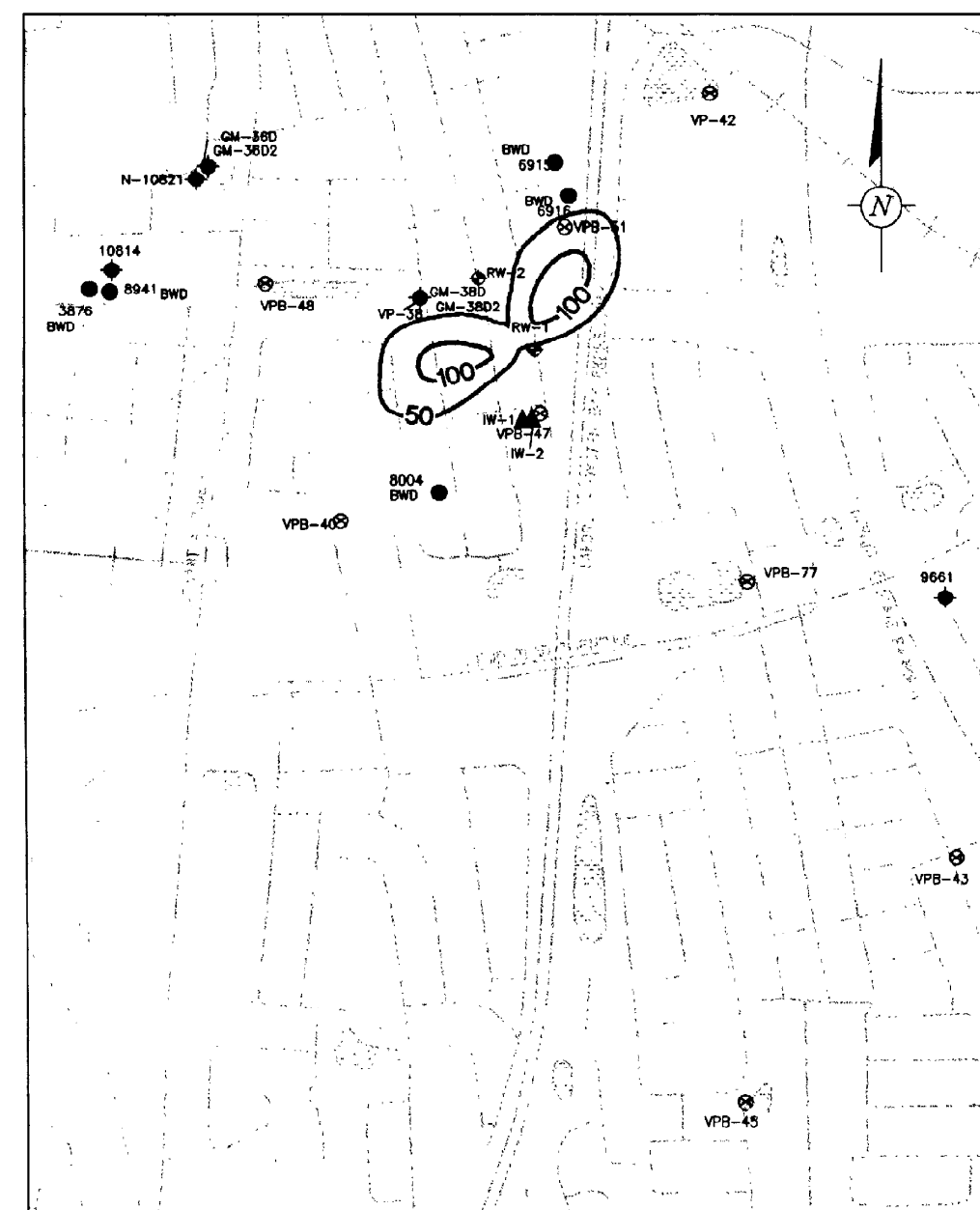
FIGURE 10: TVOC CONCENTRATIONS IN MODEL LAYER 5 AT THE GM38 AREA WITH THE PROPOSED 2-WELL REMEDIAL SYSTEM PUMPING FOR 5 YEARS SCALE: 1" = 80'
