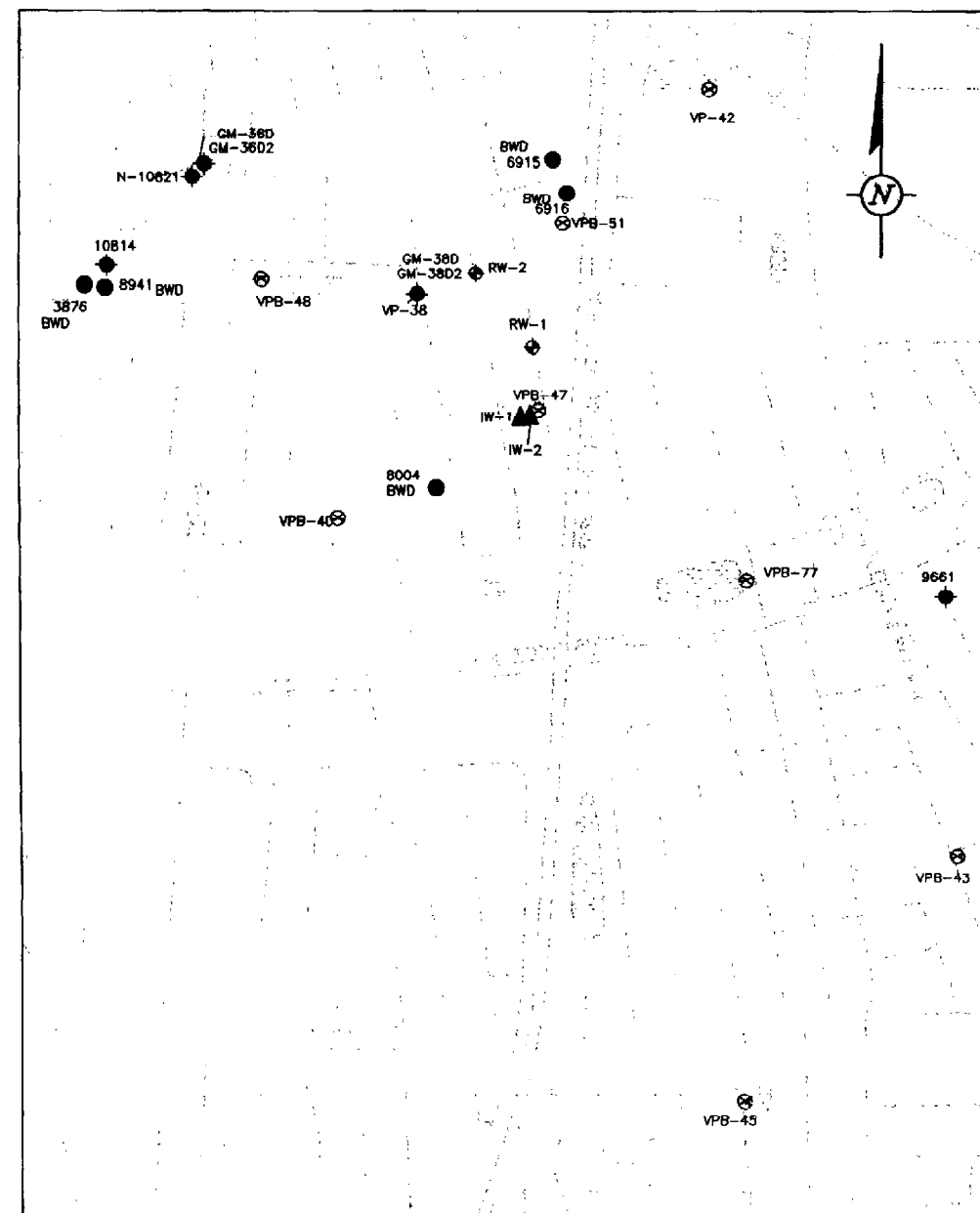
FIGURE 22: TVOC CONCENTRATIONS IN MODEL LAYER 5 AFTER 30 YEARS (PROPOSED 2-WELL REMEDIAL SYSTEM OPERATED FOR 10 YEARS AT THE START OF THE SIMULATION) SCALE: 1" = 80'
