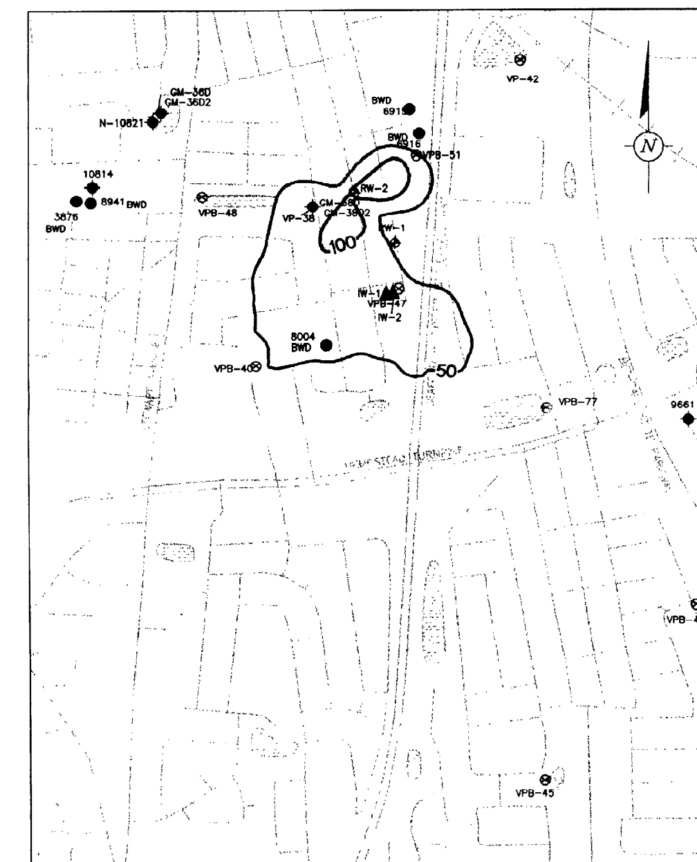
FIGURE 12: TVOC CONCENTRATIONS IN MODEL LAYER 7 AT THE GM38 AREA WITH THE PROPOSED 2-WELL REMEDIAL SYSTEM PUMPING FOR 5 YEARS SCALE: 1" = 80'
