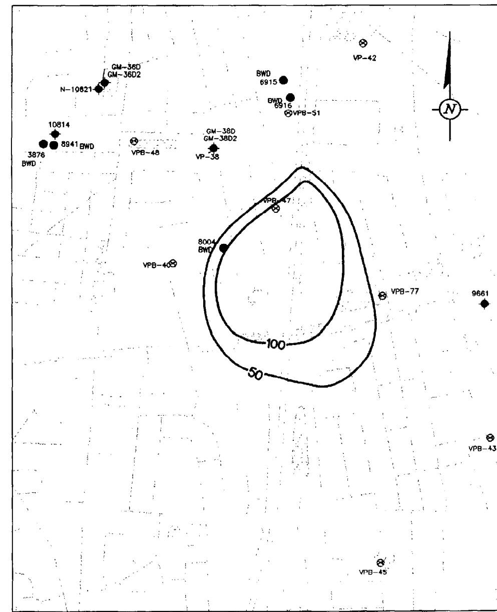
FIGURE 20: TVOC CONCENTRATIONS IN MODEL LAYER 6 AFTER 30 YEARS WITH NO REMEDIAL ACTION AT THE GM38 AREA SCALE: 1" = 80'
