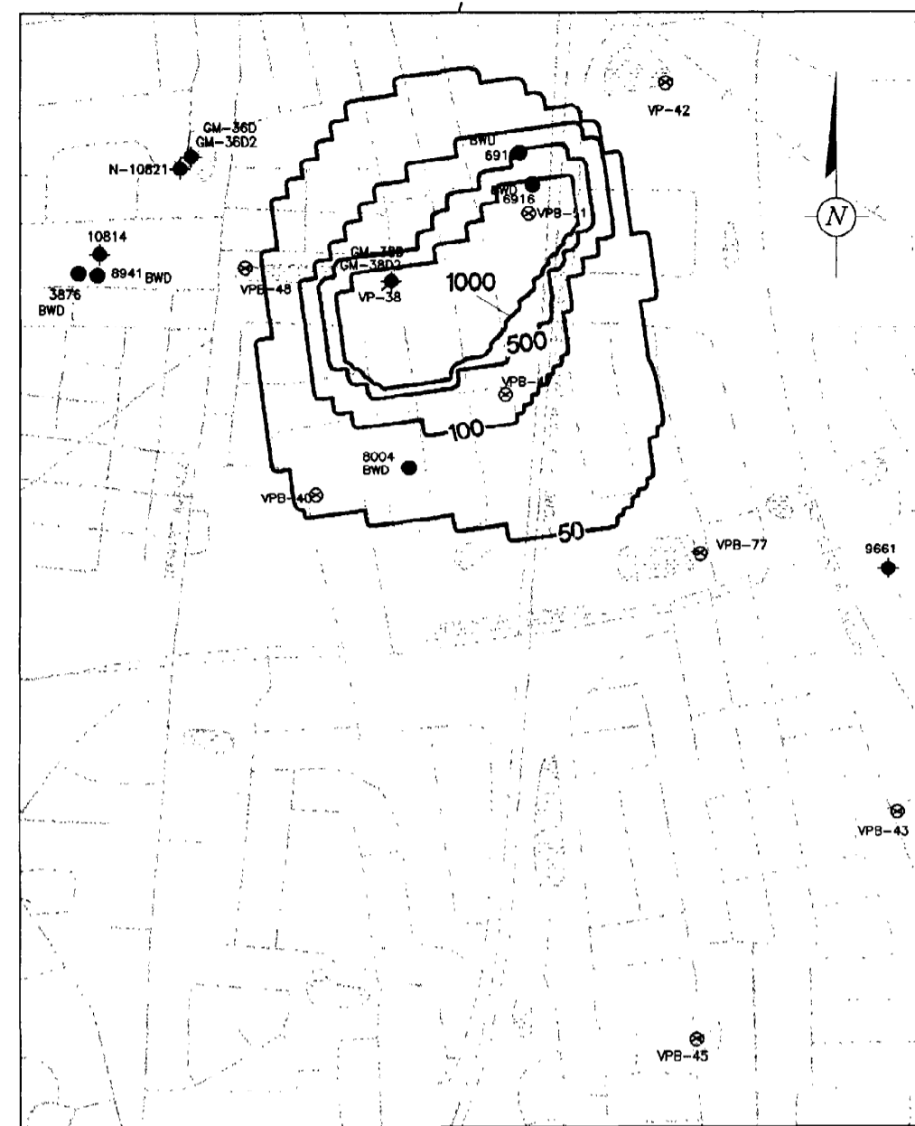
FIGURE 2: PRESENT DAY TVOC CONCENTRATIONS IN MODEL LAYER 6 NO REMEDIAL ACTION AT THE GM38 AREA SCALE: 1" = 80'
