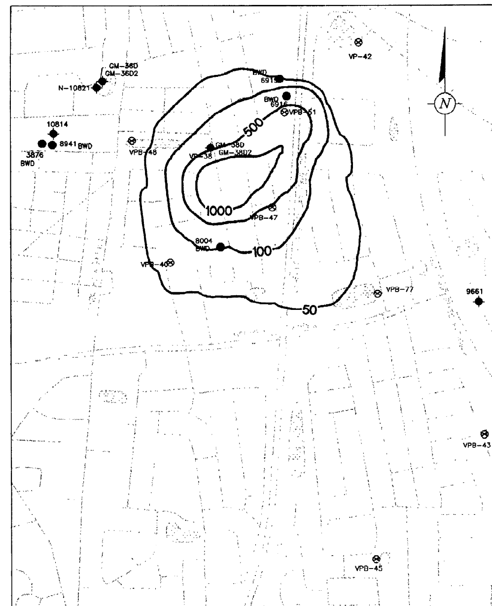
FIGURE 8: TVOC CONCENTRATIONS IN MODEL LAYER 6 AFTER 5 YEARS WITH NO REMEDIAL ACTION AT THE GM38 AREA SCALE: 1" = 80'
