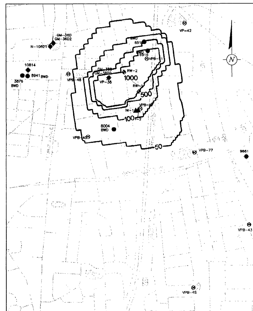
FIGURE 5: PRESENT DAY TVOC CONCENTRATIONS IN MODEL LAYER 6 PROPOSED 2-WELL REMEDIAL SYSTEM AT THE GM38 AREA SCALE: 1" = 80'
