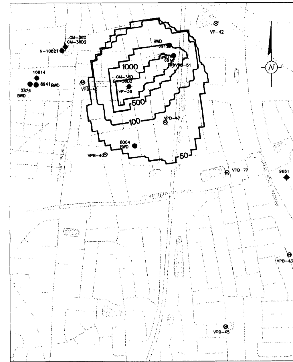
FIGURE 3: PRESENT DAY TVOC CONCENTRATIONS IN MODEL LAYER 7 NO REMEDIAL ACTION AT THE GM38 AREA SCALE: 1" = 80'
