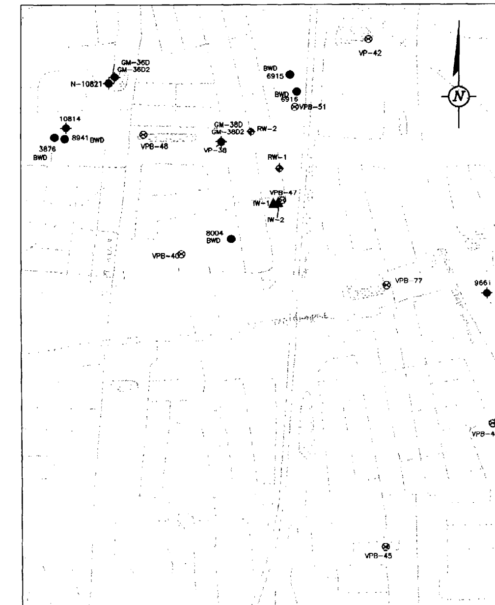
FIGURE 24: TVOC CONCENTRATIONS IN MODEL LAYER 7 AFTER 30 YEARS (PROPOSED 2-WELL REMEDIAL SYSTEM OPERATED FOR 10 YEARS AT THE START OF THE SIMULATION) SCALE: 1" = 80'
