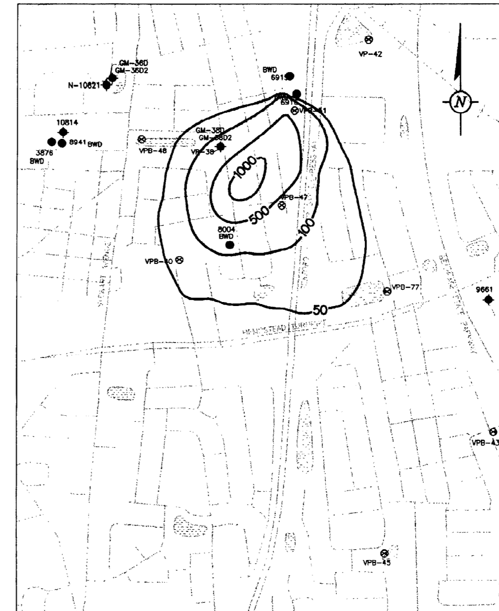
FIGURE 15: TVOC CONCENTRATIONS IN MODEL LAYER 7 AFTER 10 YEARS WITH NO REMEDIAL ACTION AT THE GM38 AREA SCALE: 1" = 80'
