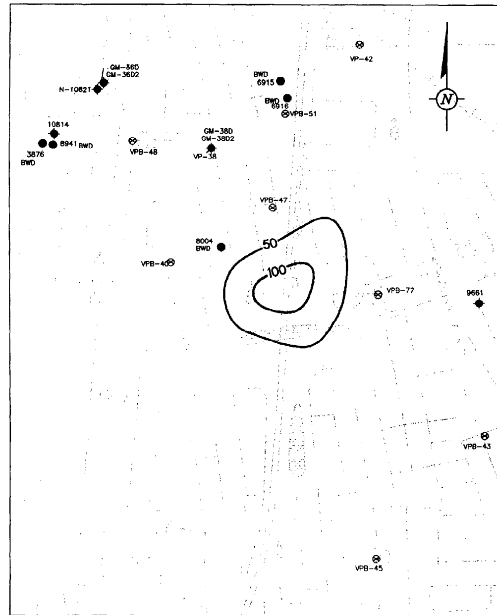
FIGURE 19: TVOC CONCENTRATIONS IN MODEL LAYER 5 AFTER 30 YEARS WITH NO REMEDIAL ACTION AT THE GM38 AREA SCALE: 1" = 80'
