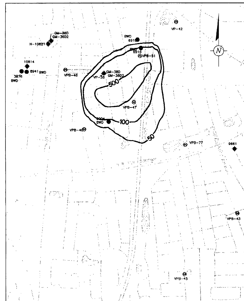
FIGURE 7: TVOC CONCENTRATIONS IN MODEL LAYER 5 AFTER 5 YEARS WITH NO REMEDIAL ACTION AT THE GM38 AREA SCALE: 1" = 80'
