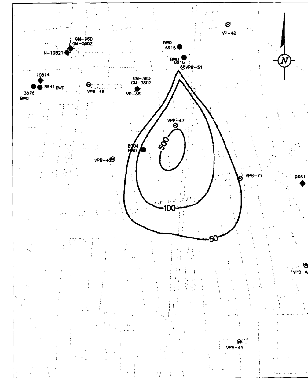
FIGURE 21: TVOC CONCENTRATIONS IN MODEL LAYER 7 AFTER 30 YEARS WITH NO REMEDIAL ACTION AT THE GM38 AREA SCALE: 1" = 80'
