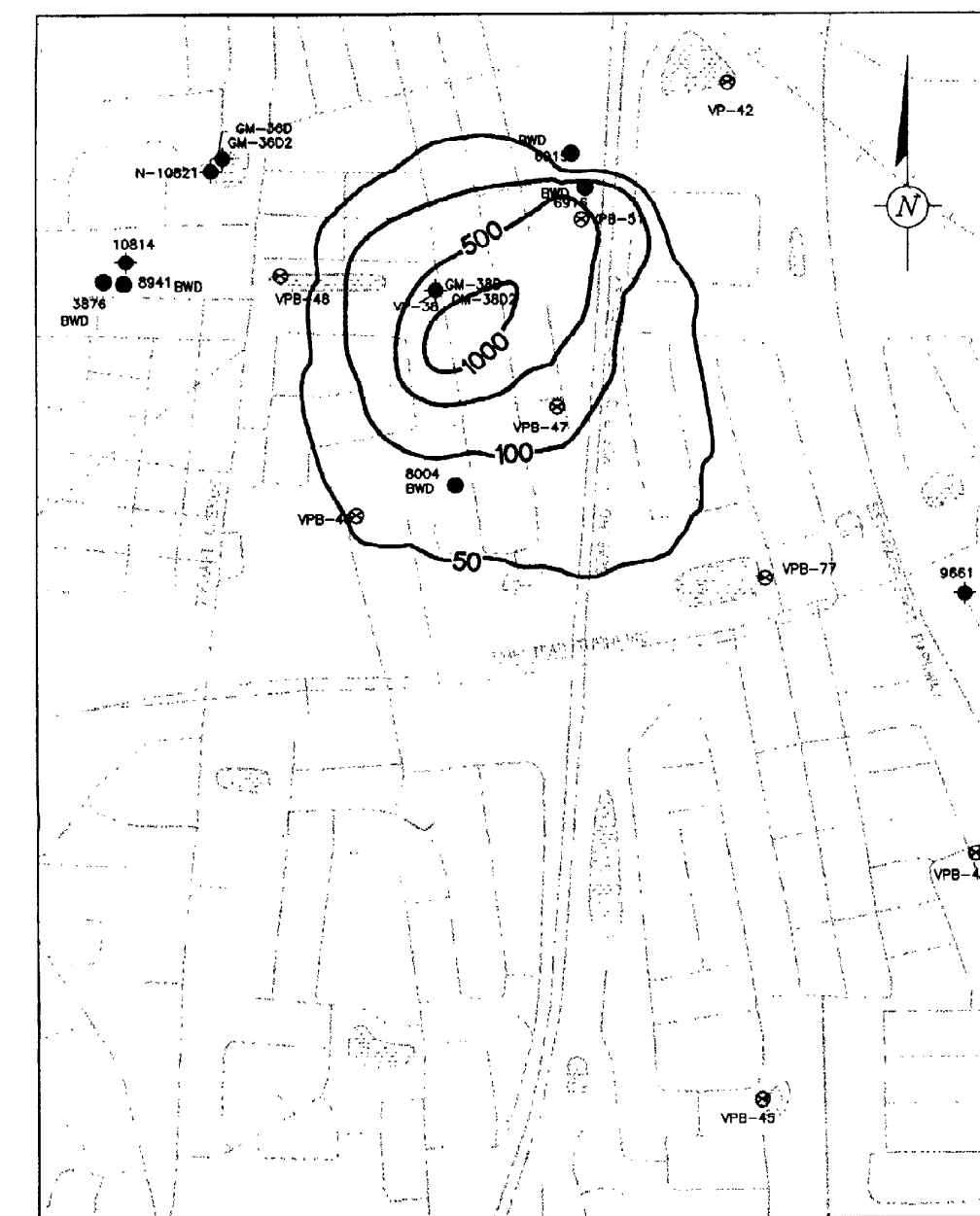
FIGURE 9: TVOC CONCENTRATIONS IN MODEL LAYER 7 AFTER 5 YEARS WITH NO REMEDIAL ACTION AT THE GM38 AREA SCALE: 1" = 80'
