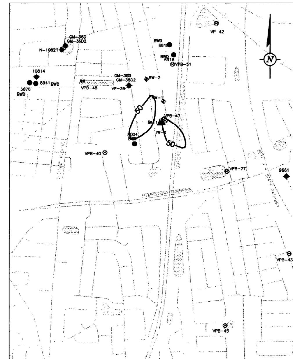
FIGURE 18: TVOC CONCENTRATIONS IN MODEL LAYER 7 AT THE GM38 AREA WITH THE PROPOSED 2-WELL REMEDIAL SYSTEM PUMPING FOR 10 YEARS SCALE: 1" = 80'
