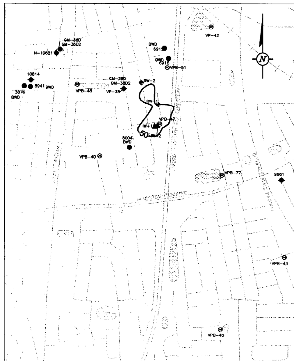
FIGURE 16: TVOC CONCENTRATIONS IN MODEL LAYER 5 AT THE GM38 AREA WITH THE PROPOSED 2-WELL REMEDIAL SYSTEM PUMPING FOR 10 YEARS SCALE: 1" = 80'
