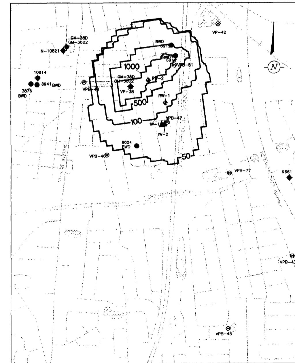
FIGURE 6: PRESENT DAY TVOC CONCENTRATIONS IN MODEL LAYER 7 PROPOSED 2-WELL REMEDIAL SYSTEM AT THE GM38 AREA SCALE: 1" = 80'
