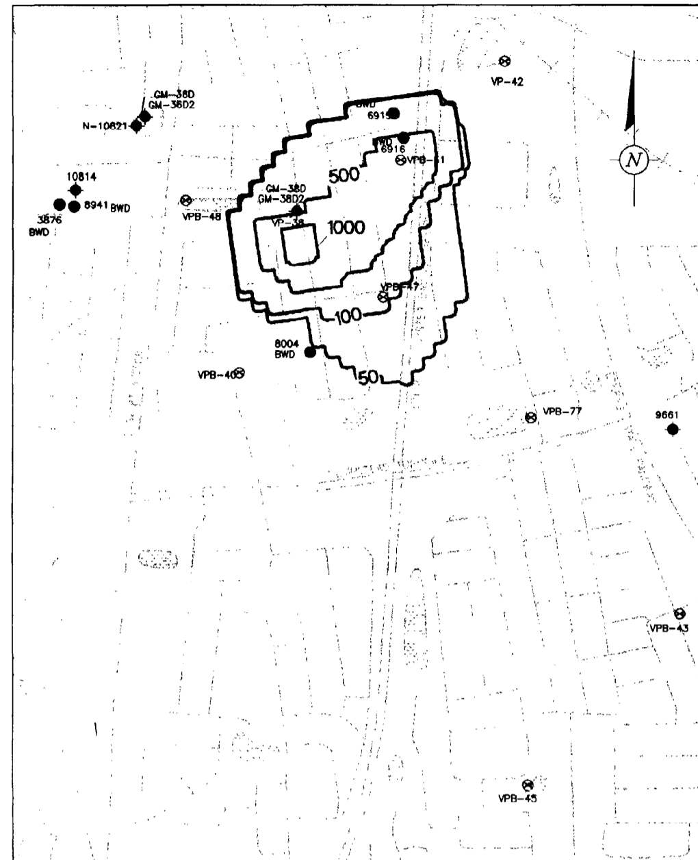
FIGURE 1: PRESENT DAY TVOC CONCENTRATIONS IN MODEL LAYER 5 NO REMEDIAL ACTION AT THE GM38 AREA SCALE: 1" = 80'
