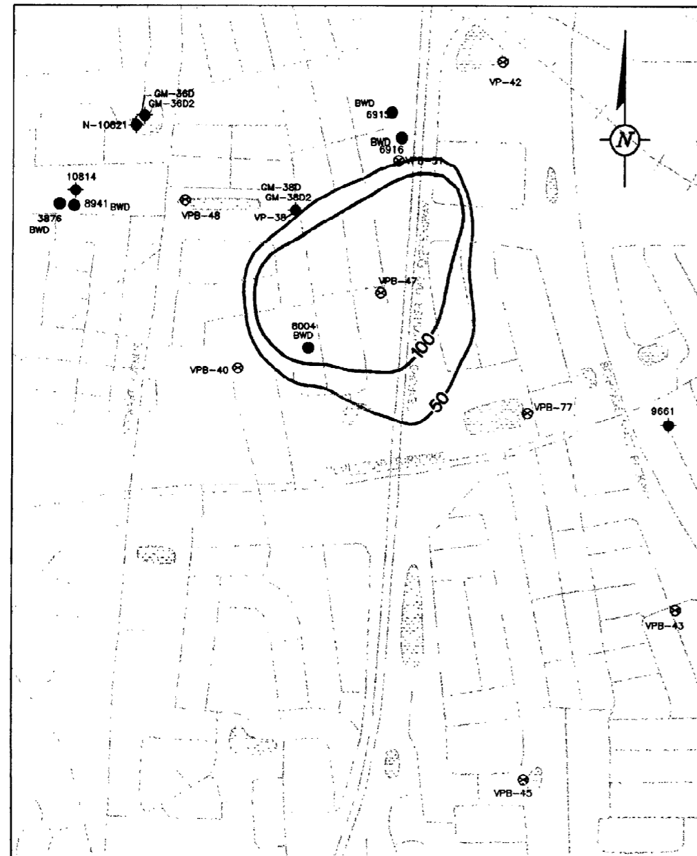
FIGURE 13: TVOC CONCENTRATIONS IN MODEL LAYER 5 AFTER 10 YEARS WITH NO REMEDIAL ACTION AT THE GM38 AREA SCALE: 1" = 80'
