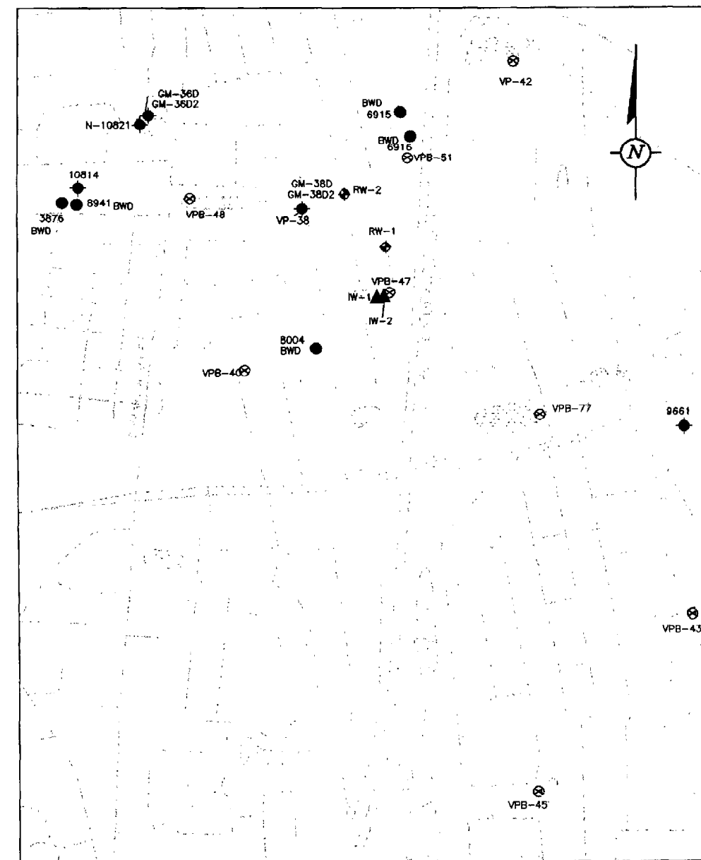
FIGURE 23: TVOC CONCENTRATIONS IN MODEL LAYER 6 AFTER 30 YEARS (PROPOSED 2-WELL REMEDIAL SYSTEM OPERATED FOR 10 YEARS AT THE START OF THE SIMULATION) SCALE: 1" = 80'
