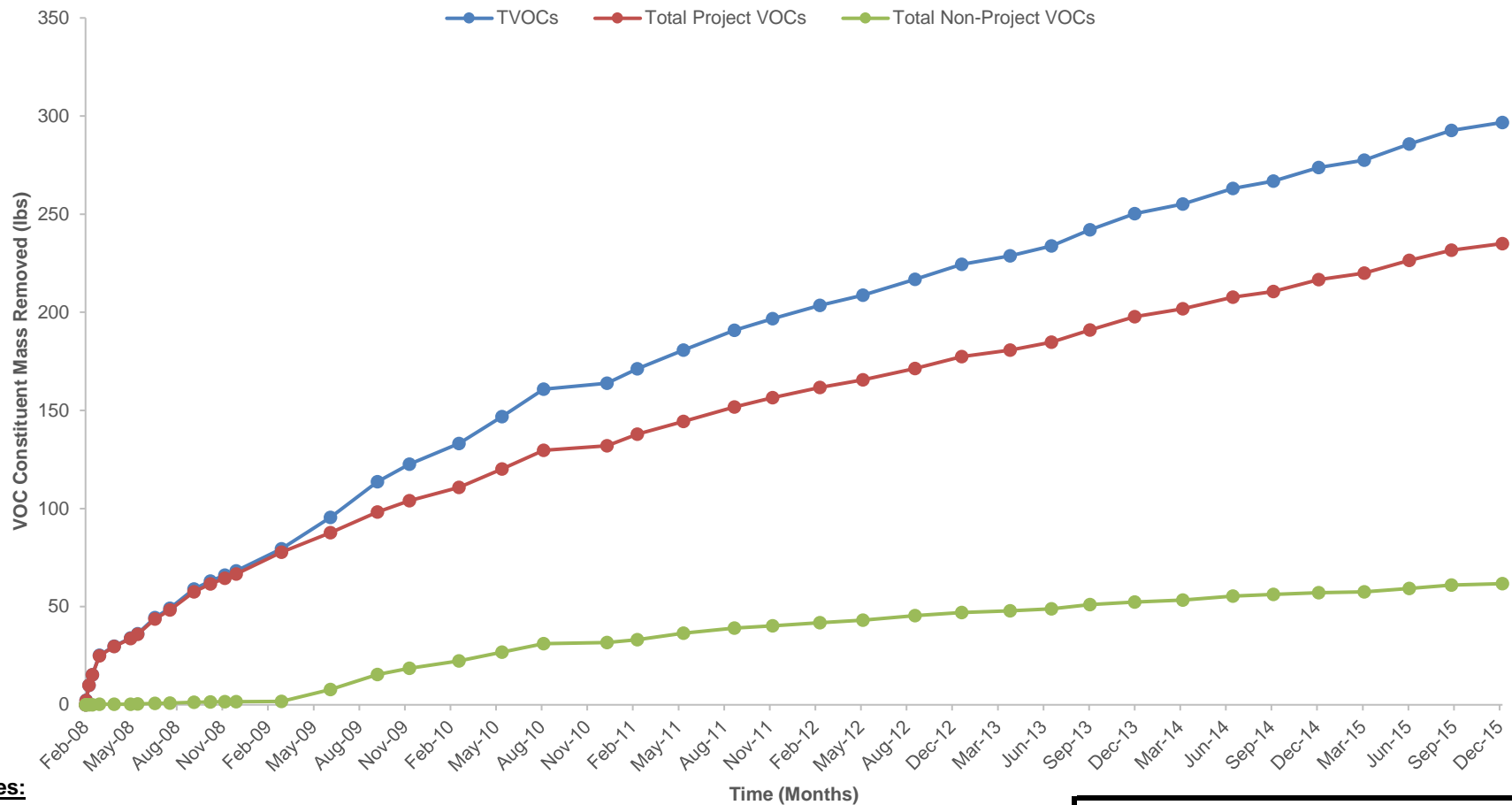
BETHPAGE PARK SOIL GAS CONTAINMENT SYSTEM, OPERABLE UNIT 3 (FORMER GRUMMAN SETTLING PONDS) BETHPAGE, NEW YORK CUMULATIVE TOTAL, PROJECT, AND NON-PROJECT VOC MASS REMOVED THROUGH DECEMBER 2015
