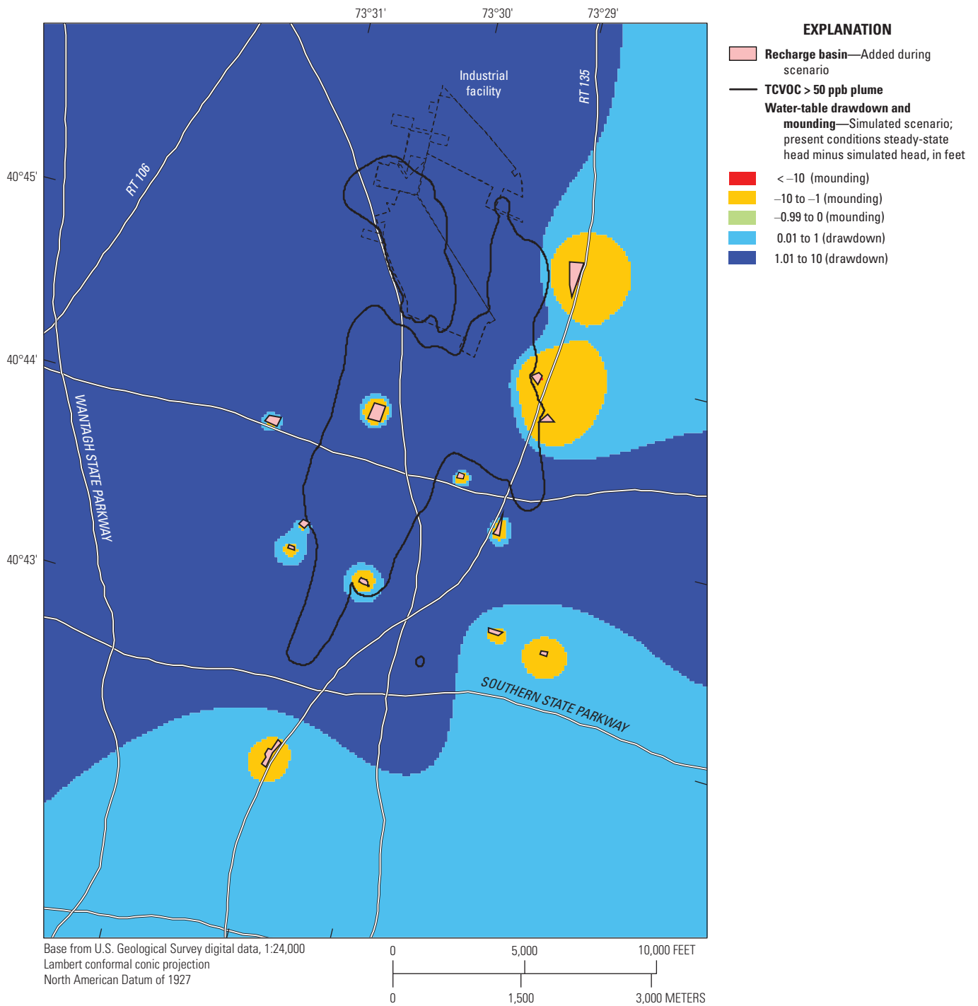
Figure 21. Maps showing locations in scenarios A, 3A and B, 3B of treated-water return and simulated water-table change from scenario 1, southeastern Nassau County, New York. TCVOC, total chlorinated volatile organic compound; ppb, part per billion; >, greater than; <, less than.
