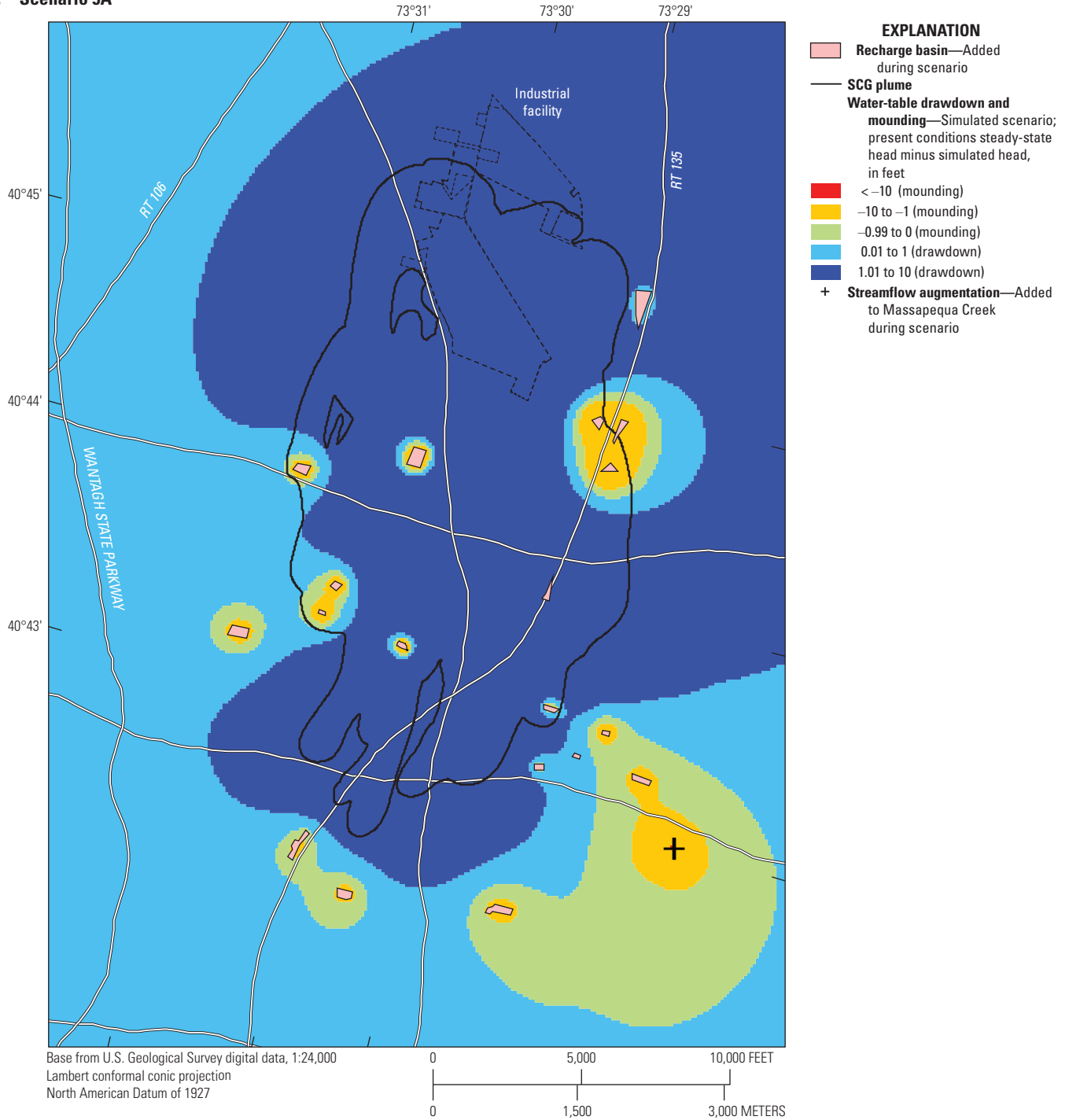
Figure 25. Maps showing changes in the locations of treated-water return and the simulated water table in scenarios A, 5A and B, 5B from scenario 1, southeastern Nassau County, New York.
