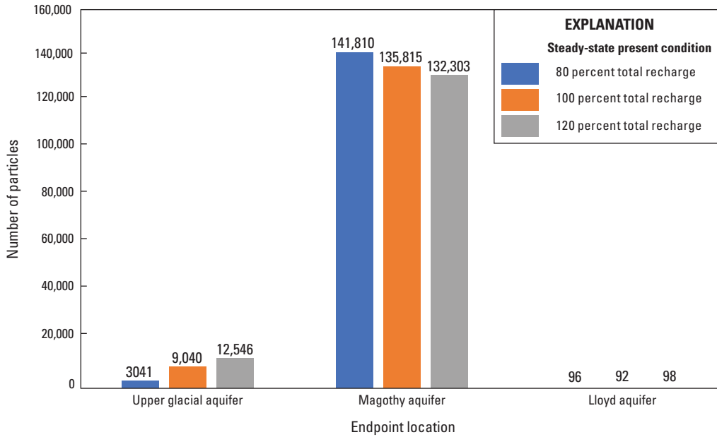
Figure 27. Graph showing effects of variation in total natural recharge on the present-conditions steady-state endpoint locations for the New York State Department of Environmental Conservation (NYSED) standards, criteria, and guidance (SCG) plume (HDR, 2019) in southeastern Nassau County, New York.
