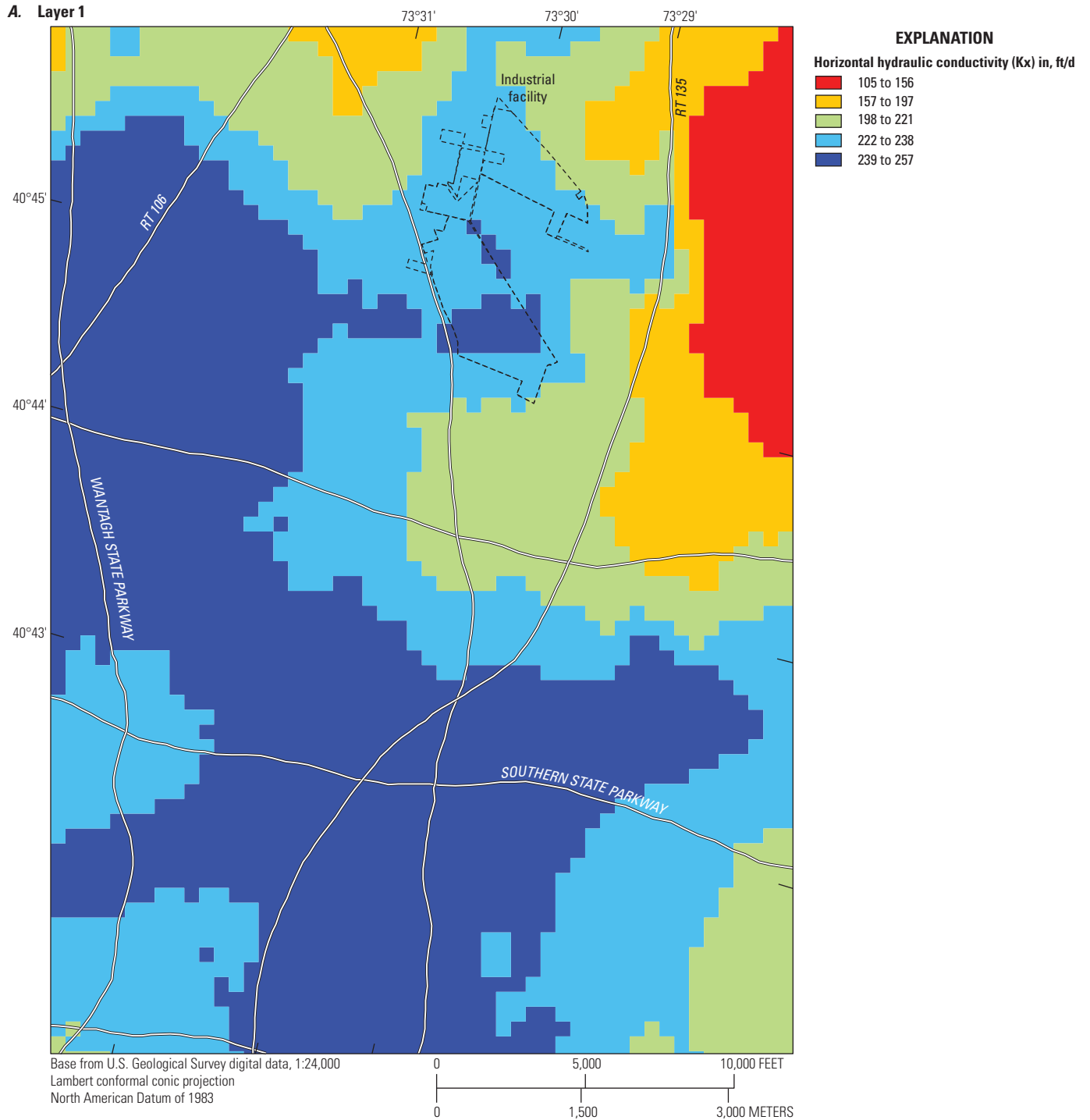
Figure 12. Maps showing hydraulic conductivity and the New York State Department of Environmental Conservation (NYSED) standards, criteria, and guidance (SCG) plume (HDR, 2019) for model layers 1 and 19, southeastern Nassau County, New York. A , Horizontal hydraulic conductivity in layer 1; B , ratio of horizontal to vertical hydraulic conductivity in layer 1; C , horizontal hydraulic conductivity in layer 19; and D , ratio of horizontal to vertical hydraulic conductivity in layer 1. K , hydraulic conductivity; K_x , horizontal hydraulic conductivity; K_v , vertical hydraulic conductivity; K_x/K_v , ratio of horizontal to vertical hydraulic conductivity; ft/d, foot per day.
