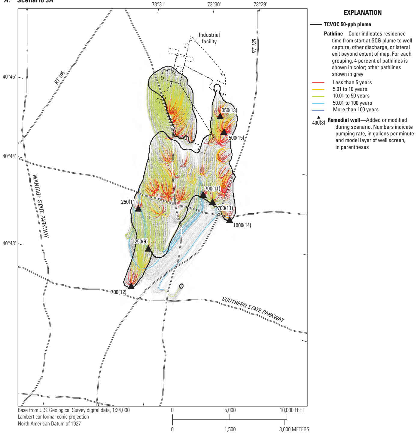
Figure 20. Maps showing scenarios A, 3A and B, 3B, pumping wells, the total chlorinated volatile organic compound (TCVOC) greater than (>) 50-part-per-billion (ppb) plume shell (HDR, 2019), and particle pathlines started at the plume shell, southeastern Nassau County, New York. A high-resolution version of this figure is available for download at https://doi.org/10.3133/sir20205090 .
