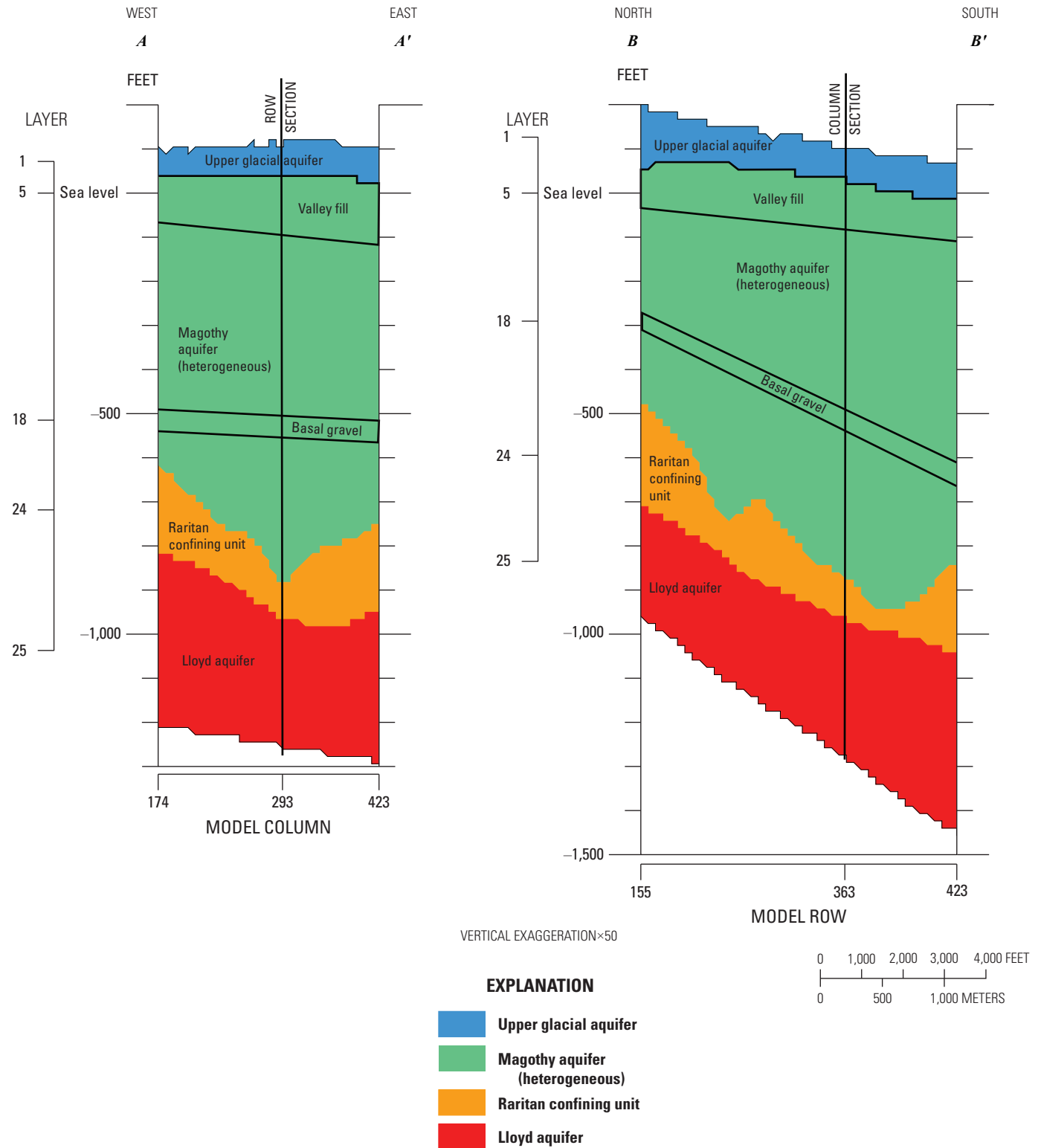
Figure 2. Model row and column sections in Nassau County, Long Island, New York. Section locations shown on figure 1.
