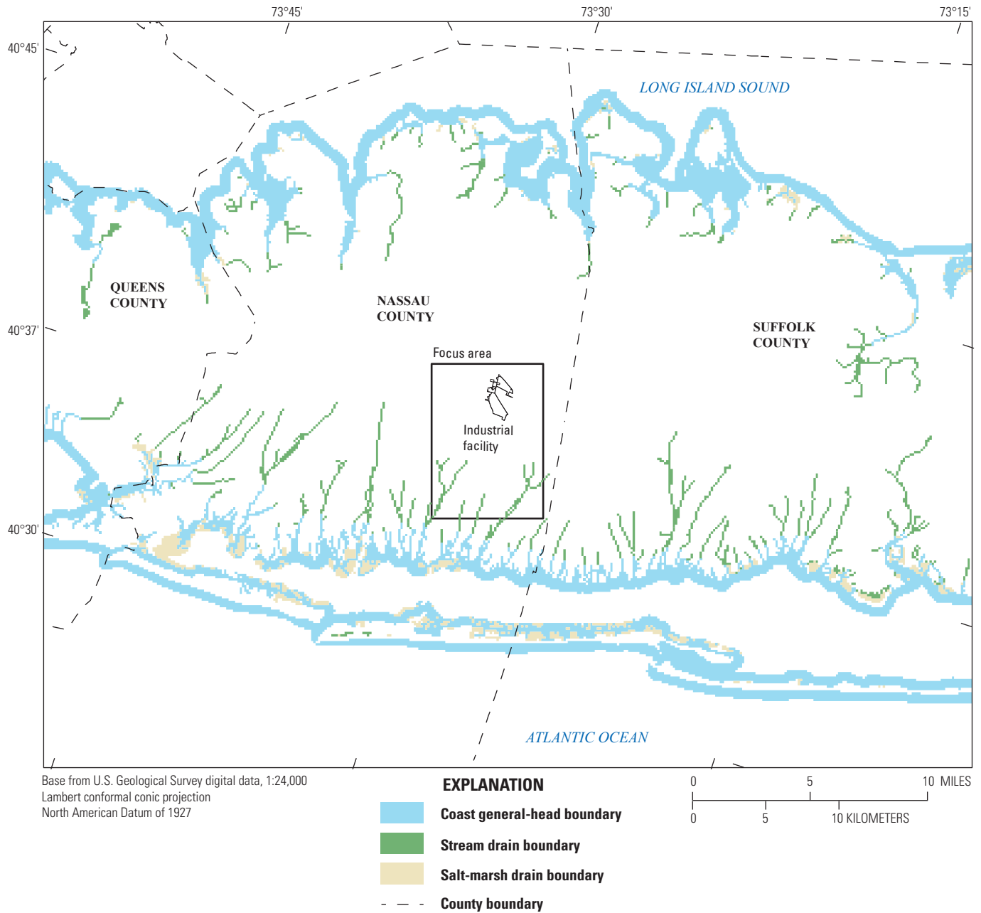
Figure 2.2. Map showing model top-layer boundaries, Long Island, New York.
