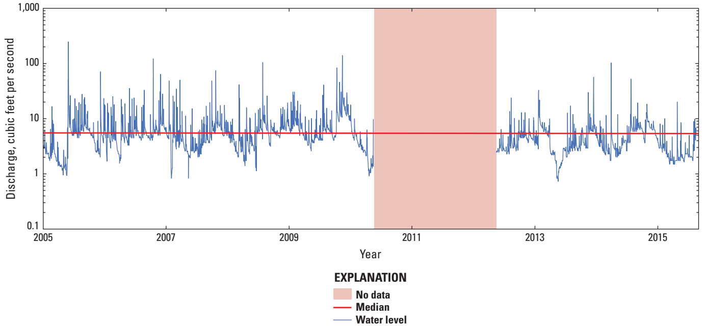
Figure 9. Graph showing daily mean discharge at U.S. Geological Survey streamgage 01309500, Massapequa Creek at Massapequa, New York, from 2005 to 2015 and the median during this period, southeastern Nassau County, New York. Location of streamgage shown on figure 6.
