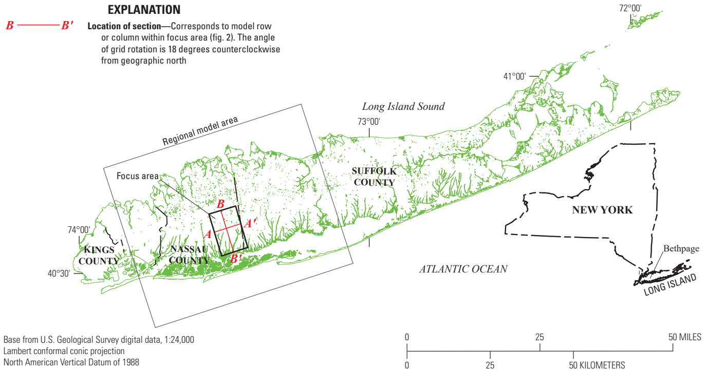
Figure 1. Model-grid domain, sections, and other local features for southeastern Nassau County, New York.
