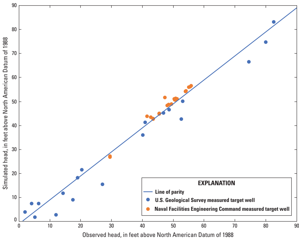
Figure 11. Graph showing the relation between observed and simulated hydraulic heads calculated for present steady-state conditions by a groundwater-flow model, southeastern Nassau County, New York.
