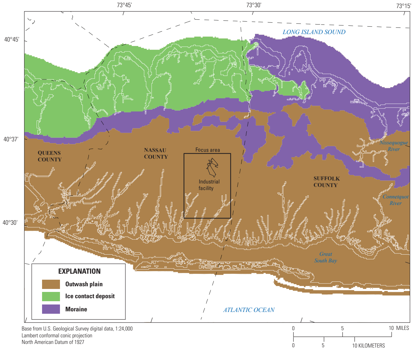
Figure 2.8. Map showing model moraine, ice-contact deposit, and outwash zones, Long Island, New York. Zone parameter values are listed in table 6 of this report.
