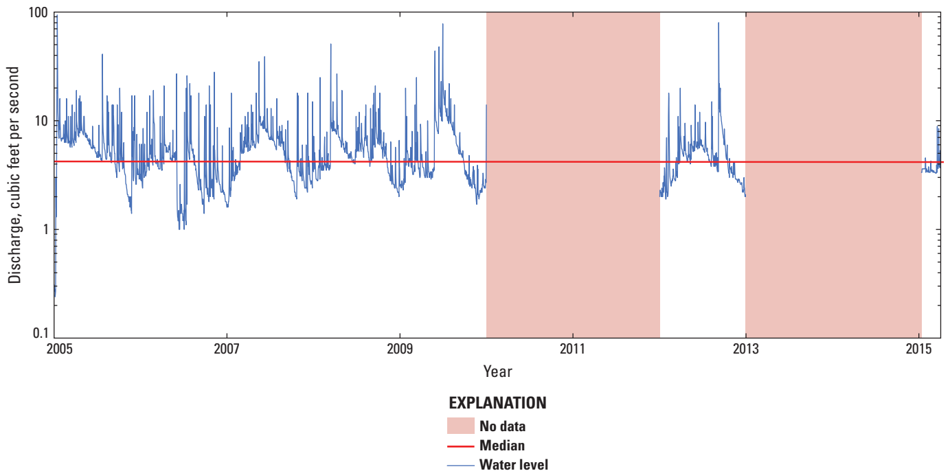
Figure 10. Graph showing daily mean discharge at U.S. Geological Survey streamgage 0309950, Bellmore Creek at Bellmore, New York, from 2005 to 2015 and the median during this period, southeastern Nassau County, New York. Location of streamgage shown on figure 6.
