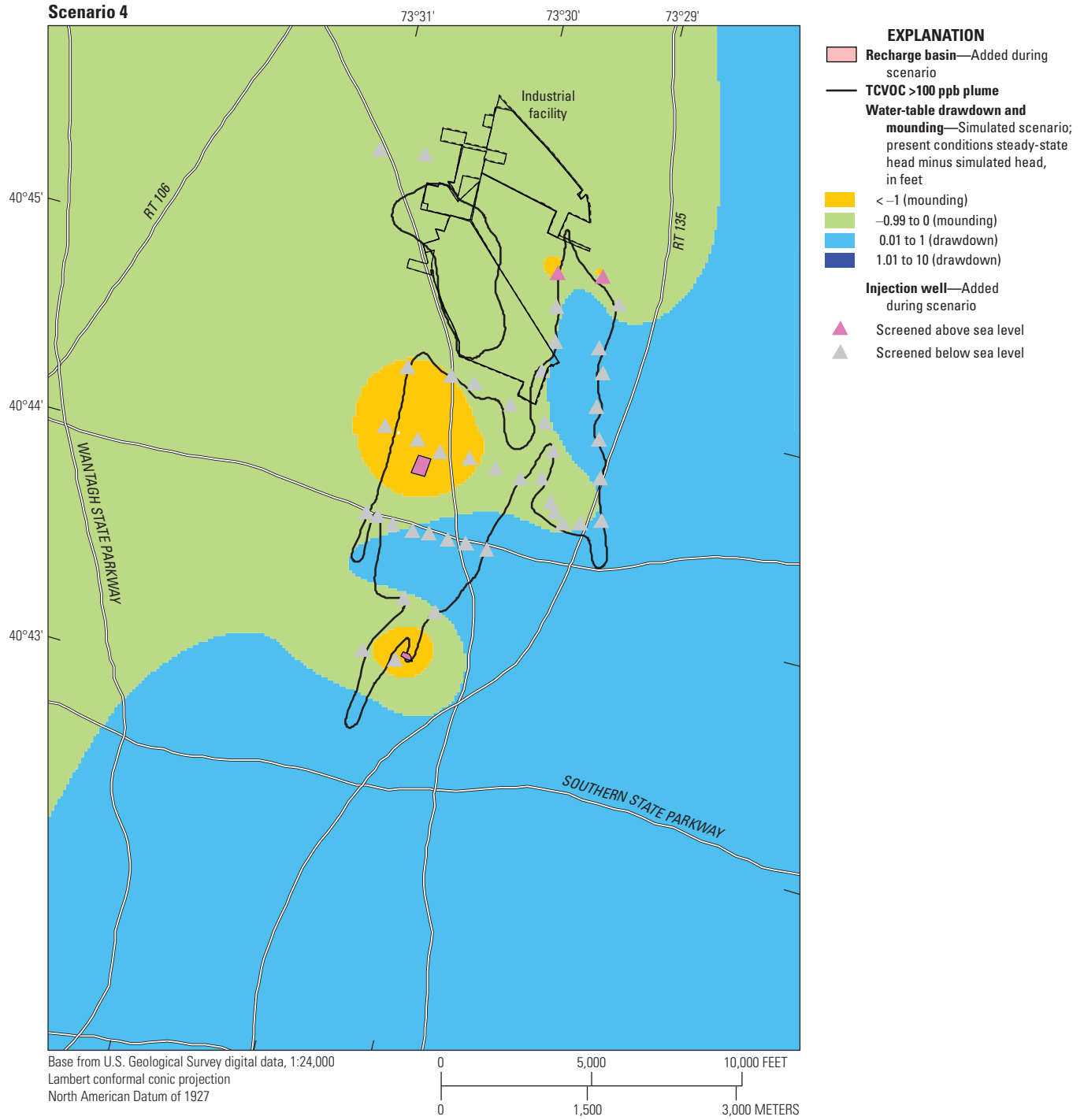
Figure 23. Map showing scenario 4 locations of treated-water return and simulated water-table change from scenario 1, southeastern Nassau County, New York. TCVOC, total chlorinated volatile organic compound; ppb, part per billion; >, greater than; <, less than.
