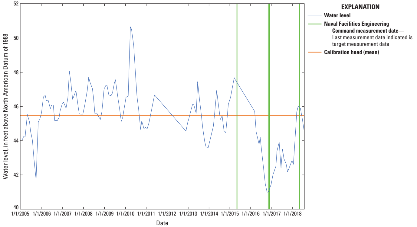
Figure 7. Graph showing water-level elevations in well N12250 measured by the U.S. Geological Survey from 2005 to 2018, the mean water level during this period, and dates of water-level measurement by the Naval Facilities Engineering Command at nearby wells from 2015 to 2018, southeastern Nassau County, New York. Location of well shown on figure 6.
