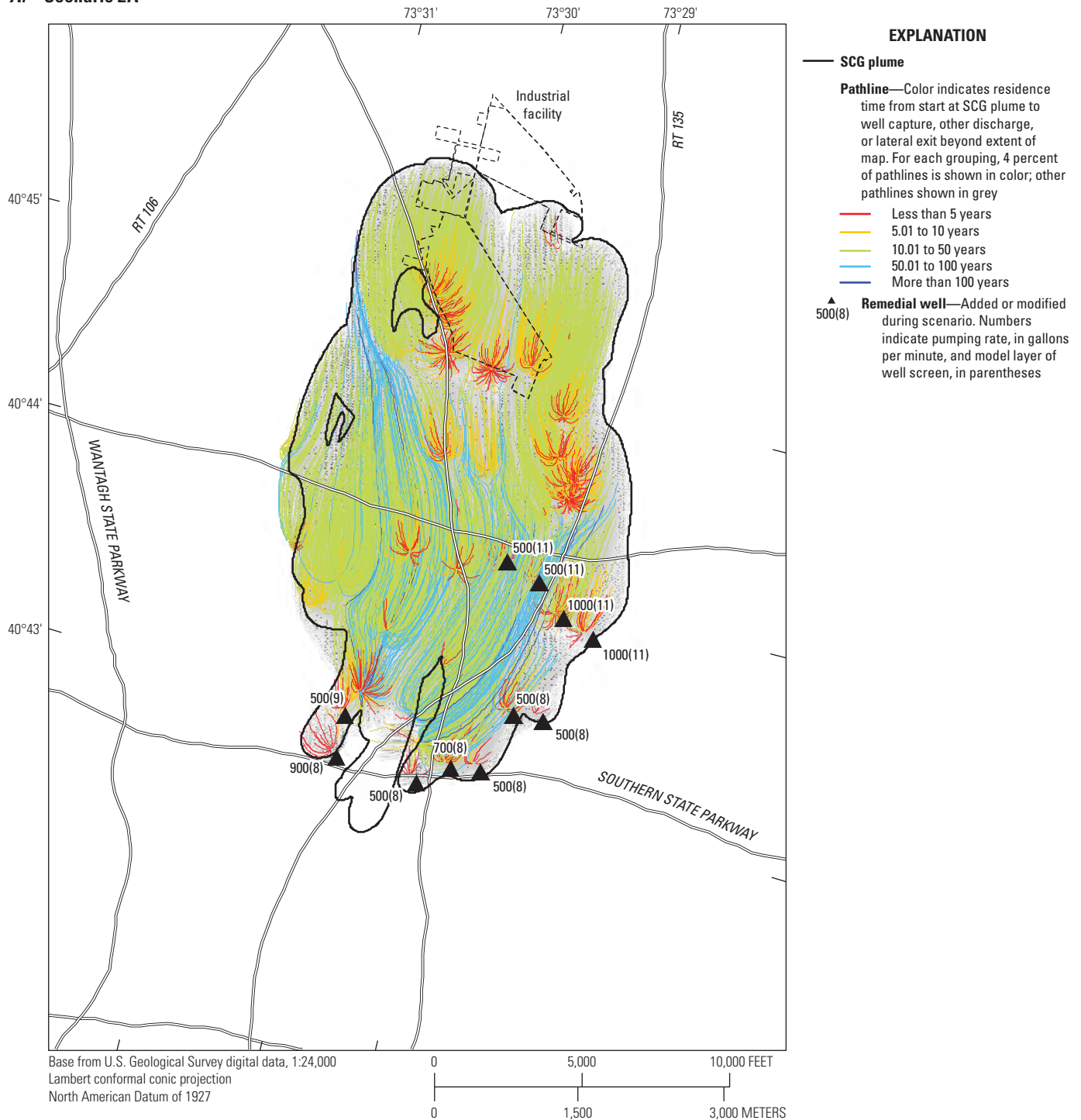
Figure 18. Maps showing remedial pumping wells, layers 6 through 15 of the New York State Department of Environmental Conservation (NYSED) standards, criteria, and guidance (SCG) plume shell (HDR, 2019) and particle pathlines started at the plume shell for A, scenario 2A, and B, scenario 2B, southeastern Nassau County, New York. A high-resolution version of this figure is available for download at https://doi.org/10.3133/sir20205090 .
