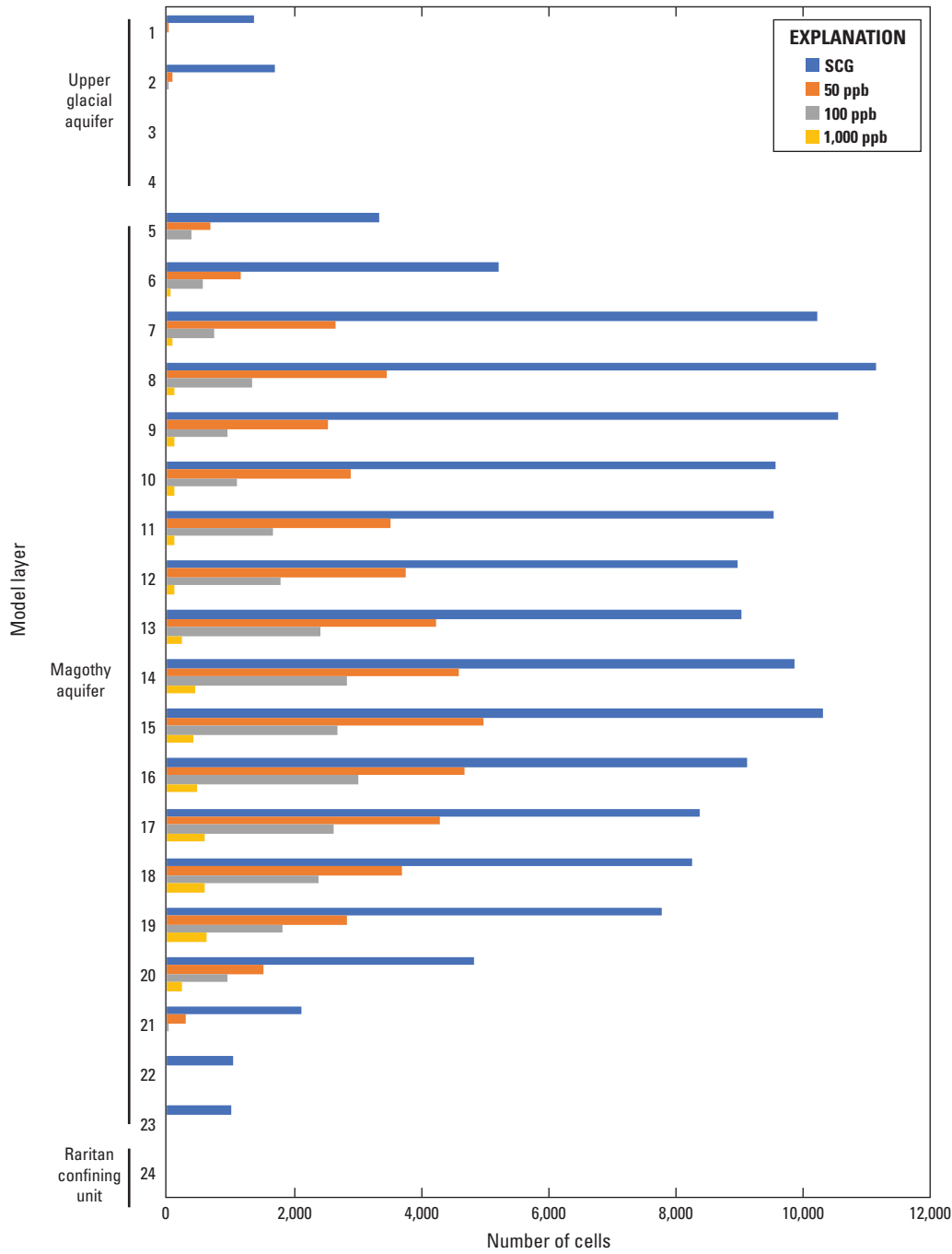
Figure 14. Graph showing number of model cells per layer that intersect the standards, criteria, and guidance (SCG), total chlorinated volatile organic compound (TCVOC) greater than (>) 50-part-per-billion (ppb), TCVOC >100-ppb, and TCVOC >1,000-ppb plumes (HDR, 2019) in southeastern Nassau County, New York.
