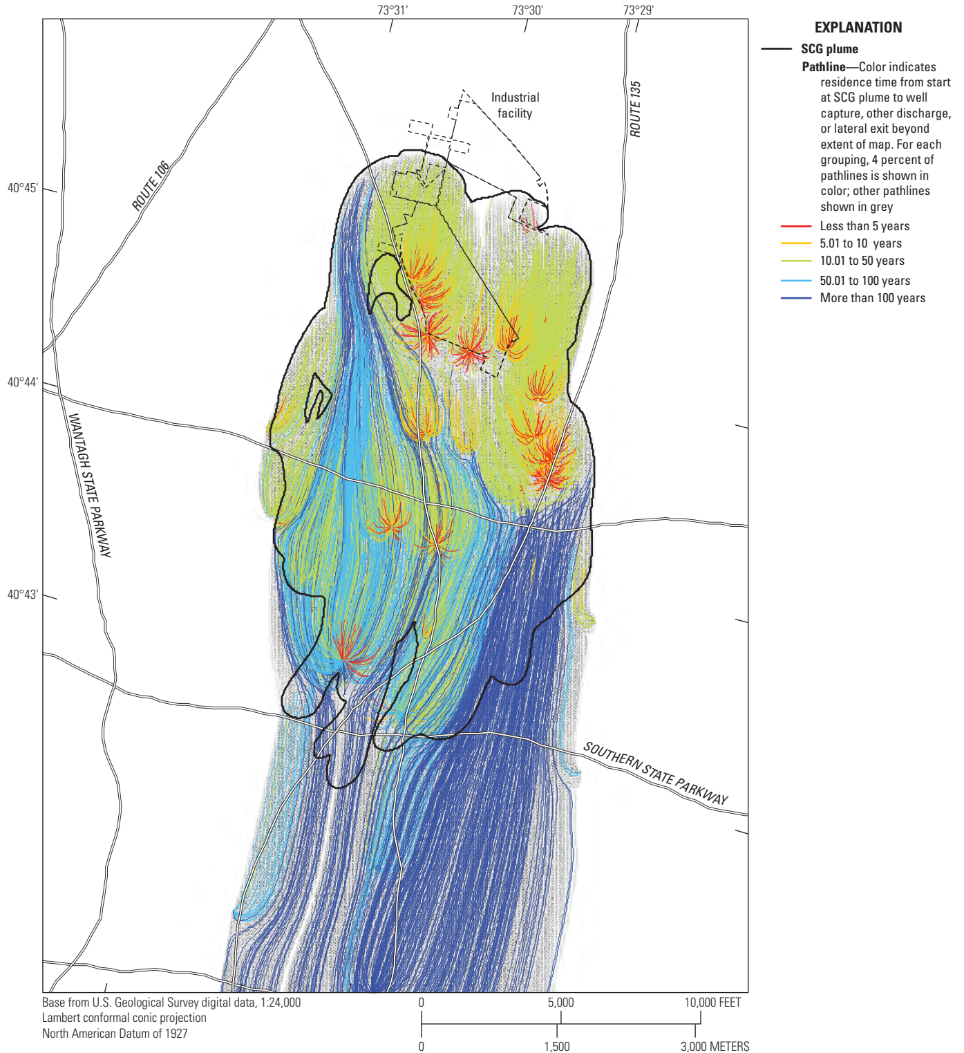
Figure 16. Map showing the New York State Department of Environmental Conservation (NYSED) standards, criteria, and guidance (SCG) plume shell (HDR, 2019) and scenario 1 particle pathlines started at the plume shell, southeastern Nassau County, New York. A high-resolution version of this figure is available for download at https://doi.org/10.3133/sir20205090 .
