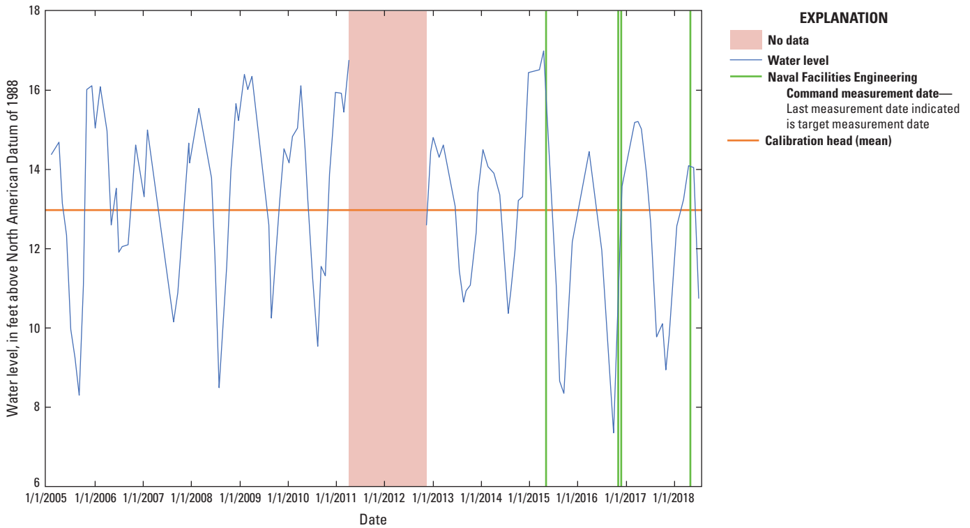
Figure 8. Graph showing water-level elevation in well N180 measured by the U.S. Geological Survey from 2005 to 2018, the mean water level during this period, and dates of measurement by the Naval Engineering Facilities Command from 2005 to 2018, southeastern Nassau County, New York. Location of well shown on figure 6.
