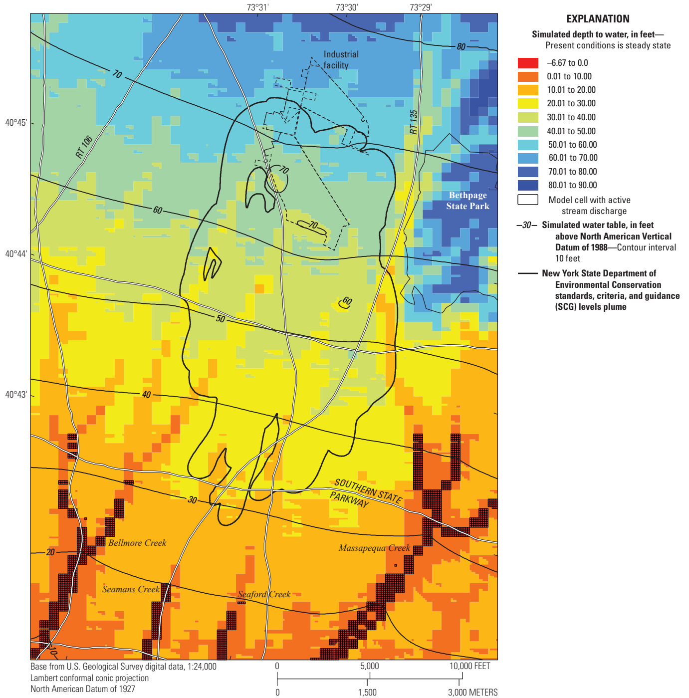
Figure 13. Map showing the water table, depth to water, and New York State Department of Environmental Conservation (NYSED) standards, criteria, and guidance (SCG) plume under present steady-state conditions (HDR, 2019), southeastern Nassau County, New York.
