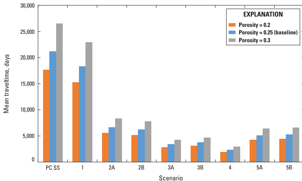
Figure 28. Graph showing sensitivities of mean travel times in the New York State Department of Environmental Conservation (NYSED) standards, criteria, and guidance (SCG) plume (HDR, 2019) of scenario particles to porosity, southeastern Nassau County, New York. Baseline value is listed in table 5. PC SS, present-condition steady-state.
