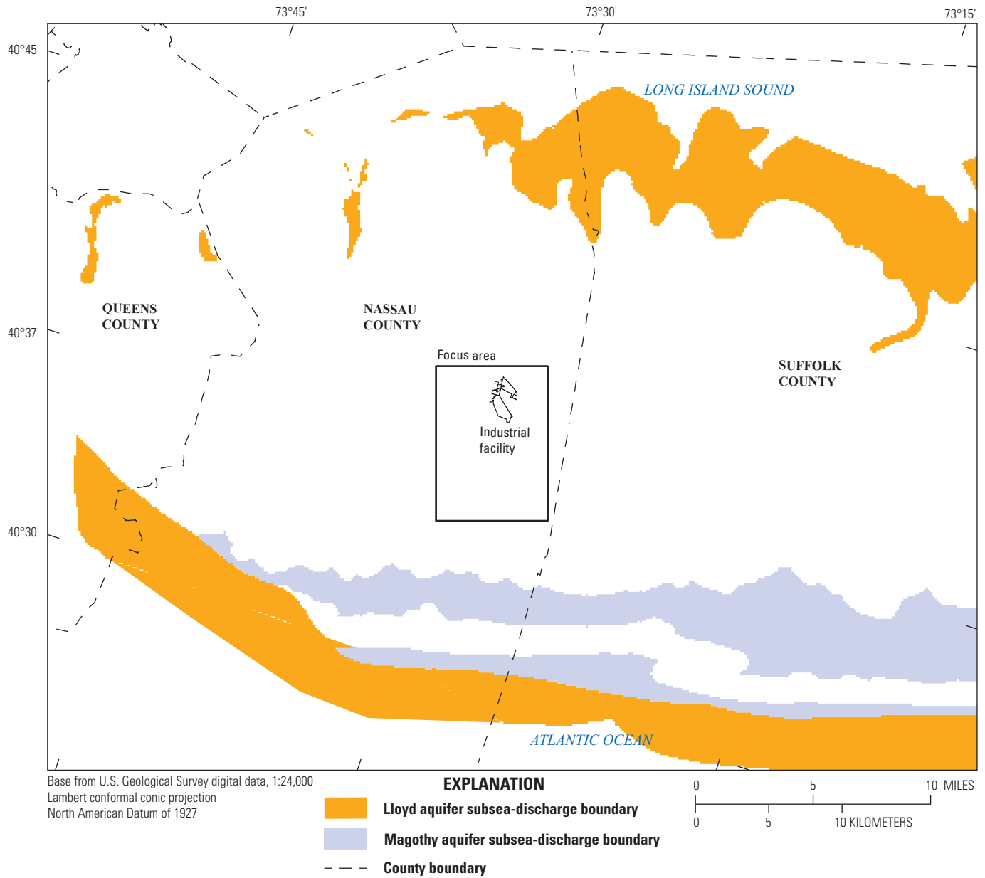
Figure 2.3. Maps showing model subsea discharge zones, Long Island, New York.
