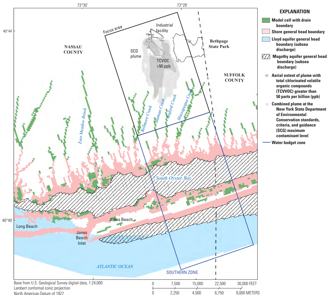
Figure 4. Map showing zones used to calculate simulated water-budget terms, representation of boundary conditions, plumes of both New York State Department of Environmental Conservation (NYSDEC) standards, criteria, and guidance (SCG) levels and total chlorinated volatile organic compounds (TCVOCs), the area in which concentrations of TCVOCs are greater than (>) 50 parts per billion (ppb; HDR, 2019), and other local features in southeastern Nassau County, New York.
