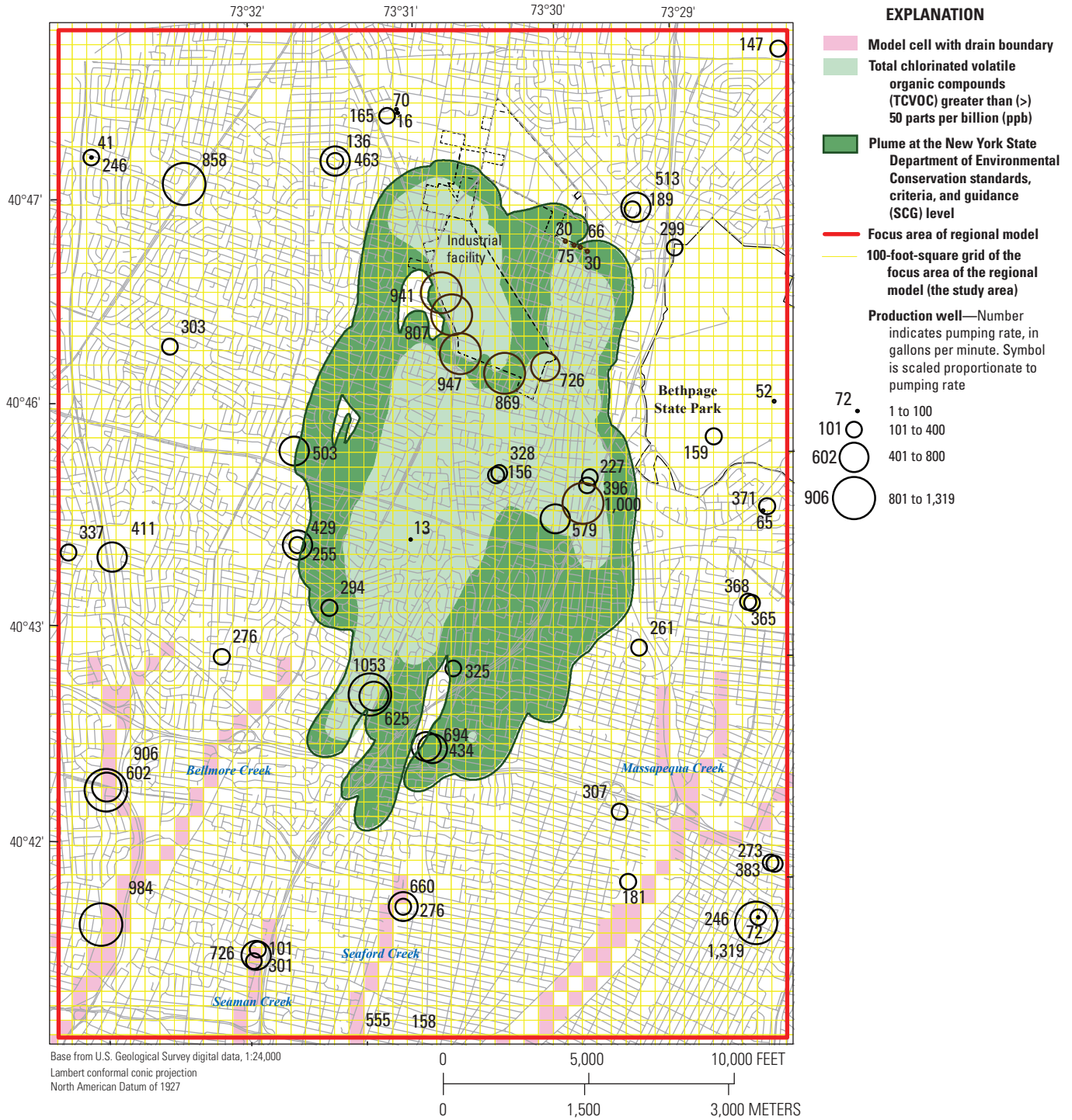
Figure 5. Map showing production wells and drain cells within focus area; plumes at New York State Department of Environmental Conservation (NYSED) standards, criteria, and guidance (SCG) levels; and plumes with concentrations of total chlorinated volatile organic compounds (TCVOC) greater than (>) 50 parts per billion (HDR, 2019), southeastern Nassau County, New York.
