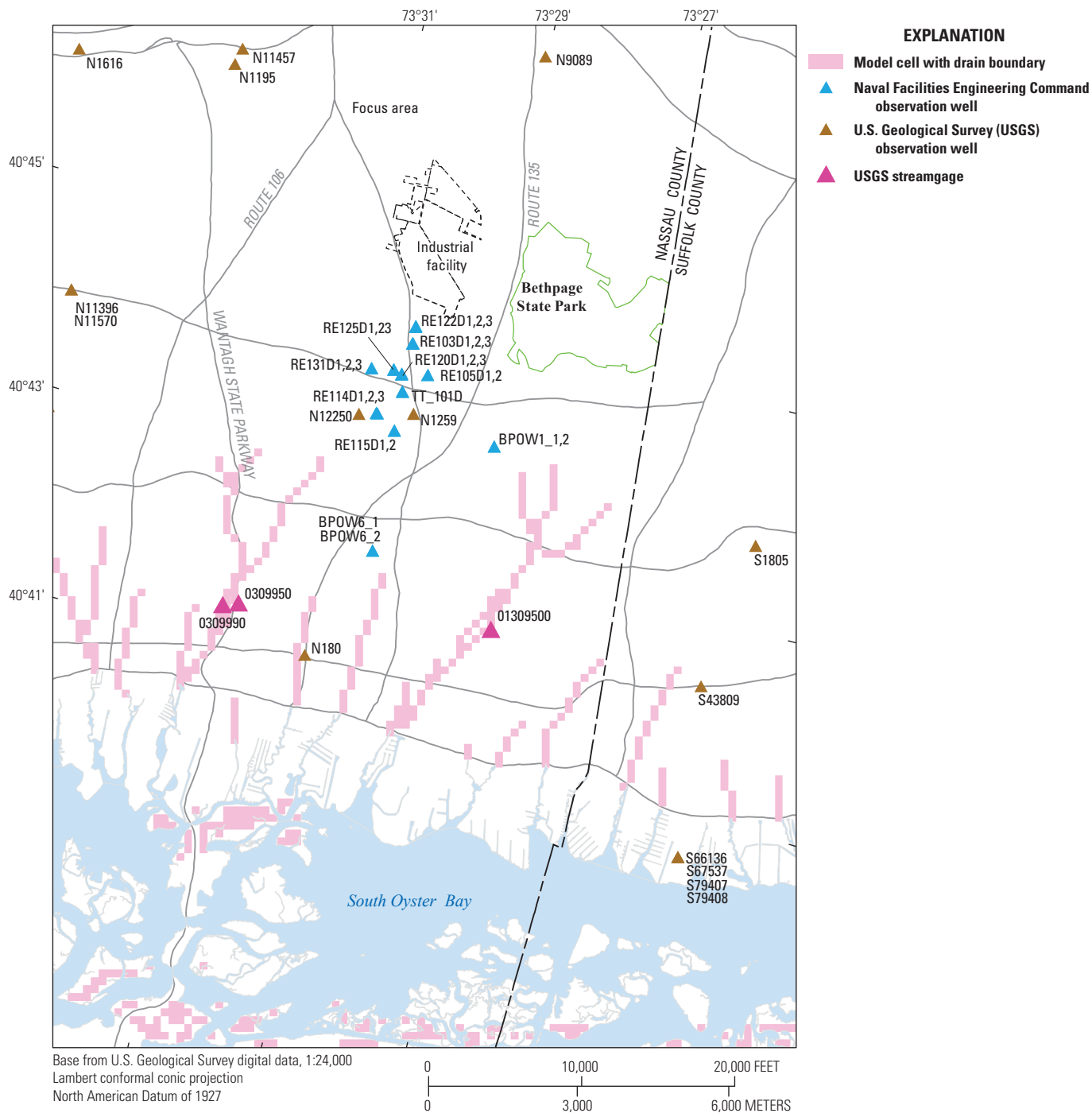
Figure 6. Map showing locations of selected observation wells and streamgages in southeastern Nassau County, New York.
