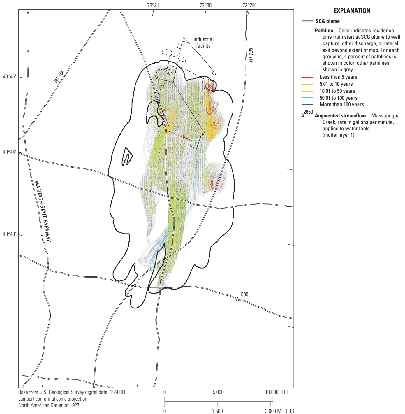
Figure 24. Maps showing remedial wells, the New York State Department of Environmental Conservation (NYSED) standards, criteria, and guidance (SCG) plume shell (HDR, 2019), and particle pathlines started at plume shell for scenarios 5A and 5B, southeastern Nassau County, New York; plume shell and particle pathlines for A, layers 1 to 5 for scenario 5A; B, layers 1 to 5 for scenario 5B; C, layers 6 to 15 for scenario 5A; D, layers 6 to 15 for scenario 5B; E, layers 16 to 23 for scenario 5A; and F, layers 16 to 23 for scenario 5B. A high-resolution version of this figure is available for download at https://doi.org/10.3133/sir20205090 .
