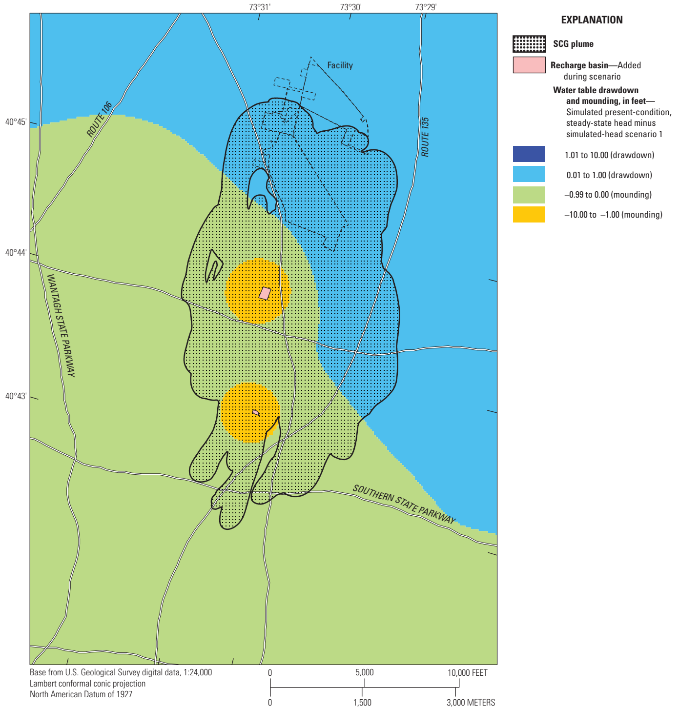
Figure 17. Map showing scenario 1 locations of treated-water return and simulated water-table change from present conditions, southeastern Nassau County, New York. SCG, New York State Department of Environmental Conservation (NYSED) standards, criteria, and guidance (SCG).
