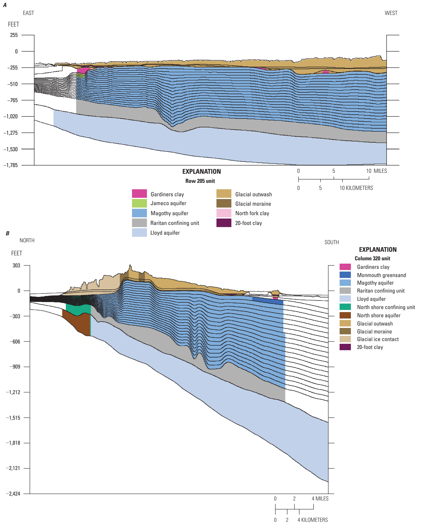
Figure 2.6. A, Row and B, column sections of a regional model showing hydrogeologic units on Long Island, New York. Locations of sections are shown on figure 2.1.
