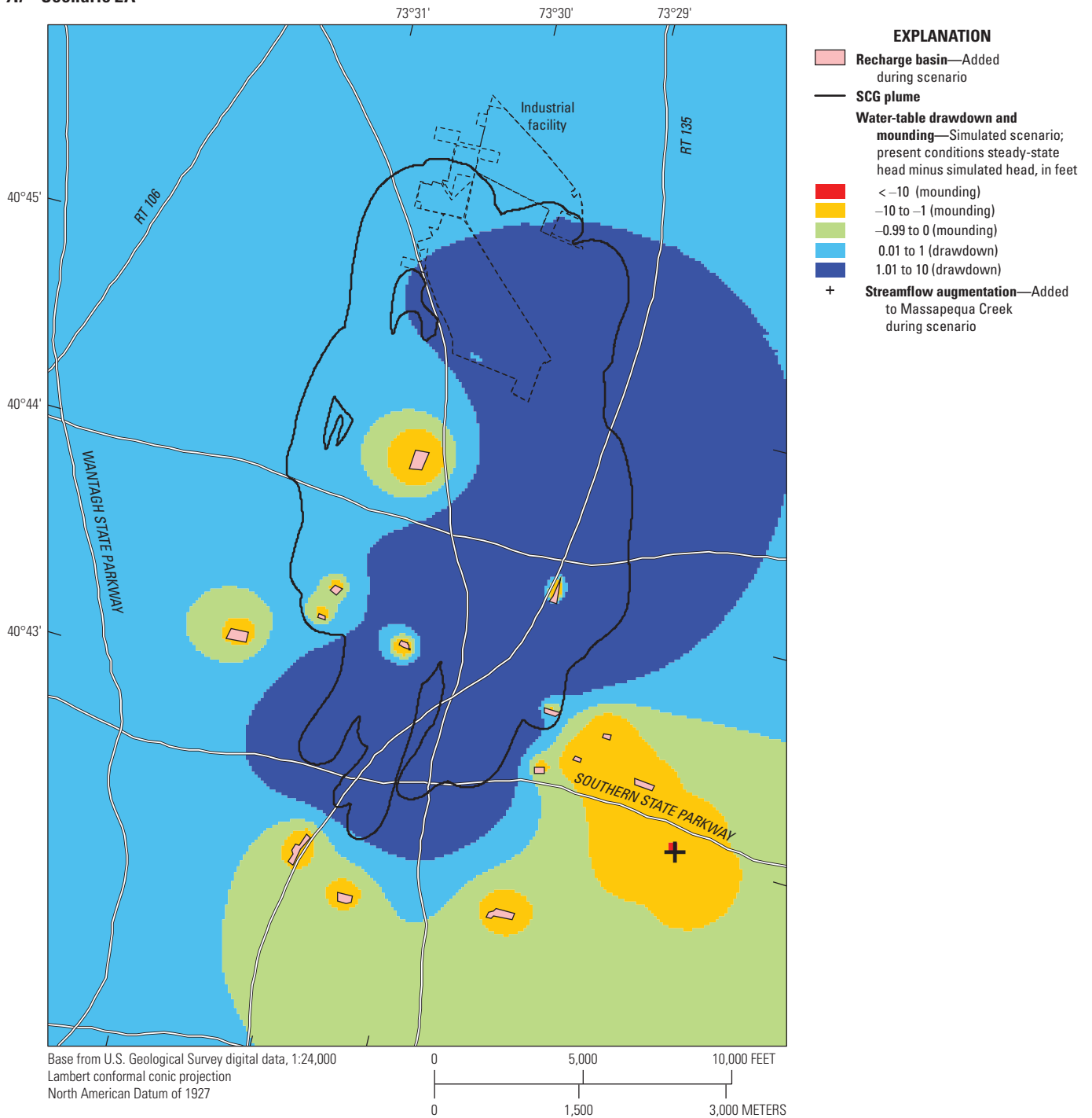
Figure 19. Maps showing locations of treated water return and simulated water-table change in scenarios A, 2A and B, 2B, southeastern Nassau County, New York. SCG, New York State Department of Environmental Conservation (NYSED) standards, criteria, and guidance; <, less than.
