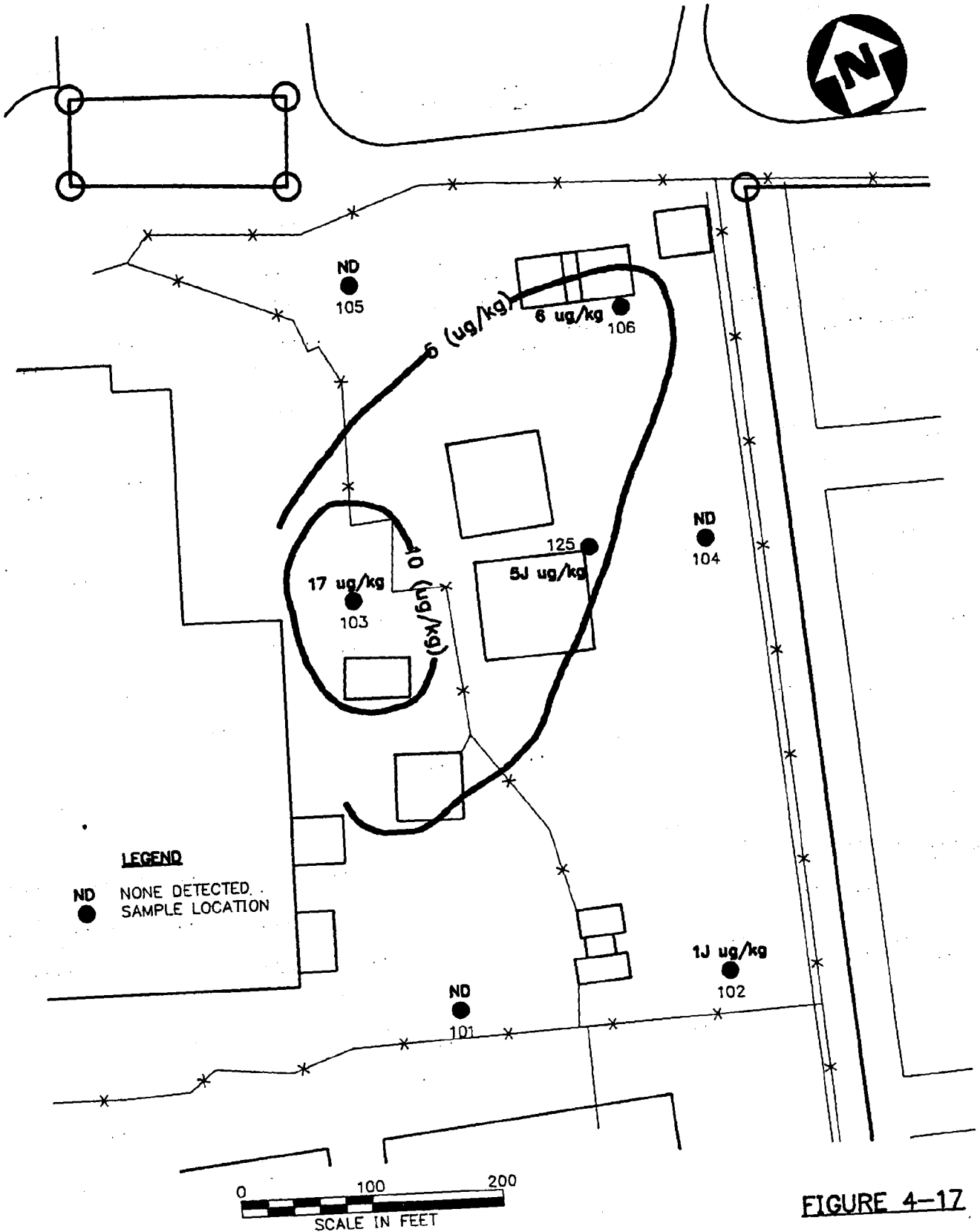
SITE 1 - SURFACE SOIL RESULTS - ICE REMEDIAL INVESTIGATION NWIRP, BETHPAGE, NY
