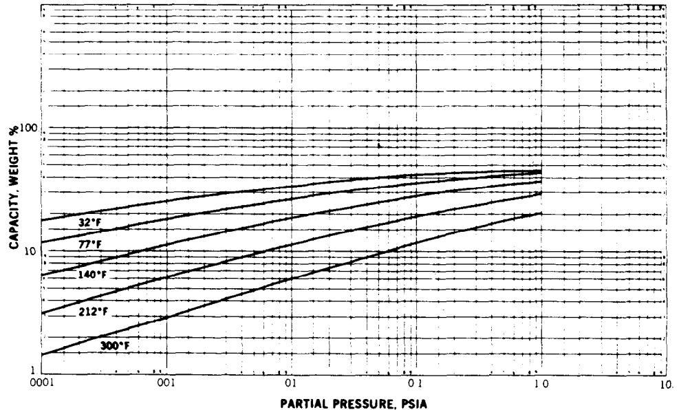
Theoretical Carbon Capacities of BPL Carbon at Atmospheric Pressure and 70° F
