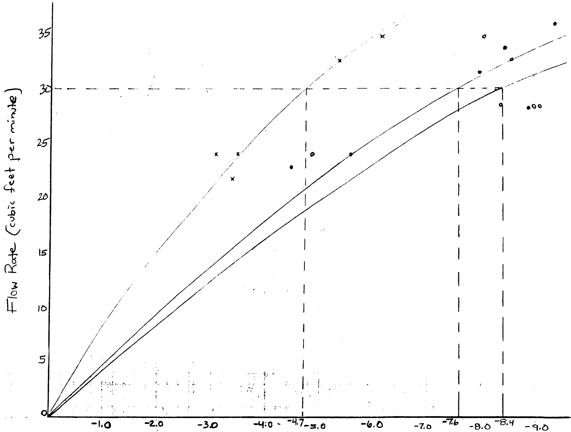
Figure 2. Flow Rate vs. Vacuum
