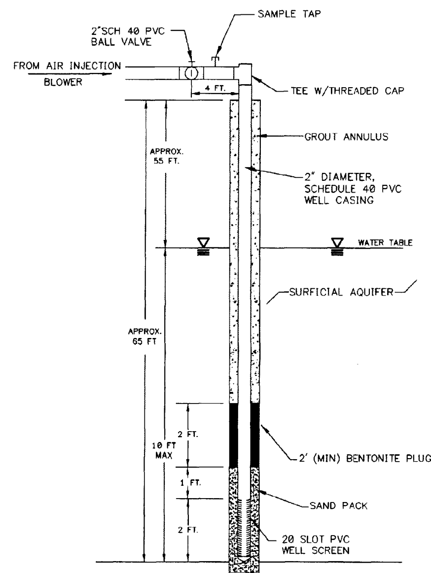
INJECTION WELL DETAIL (TYPICAL) NOT TO SCALE
