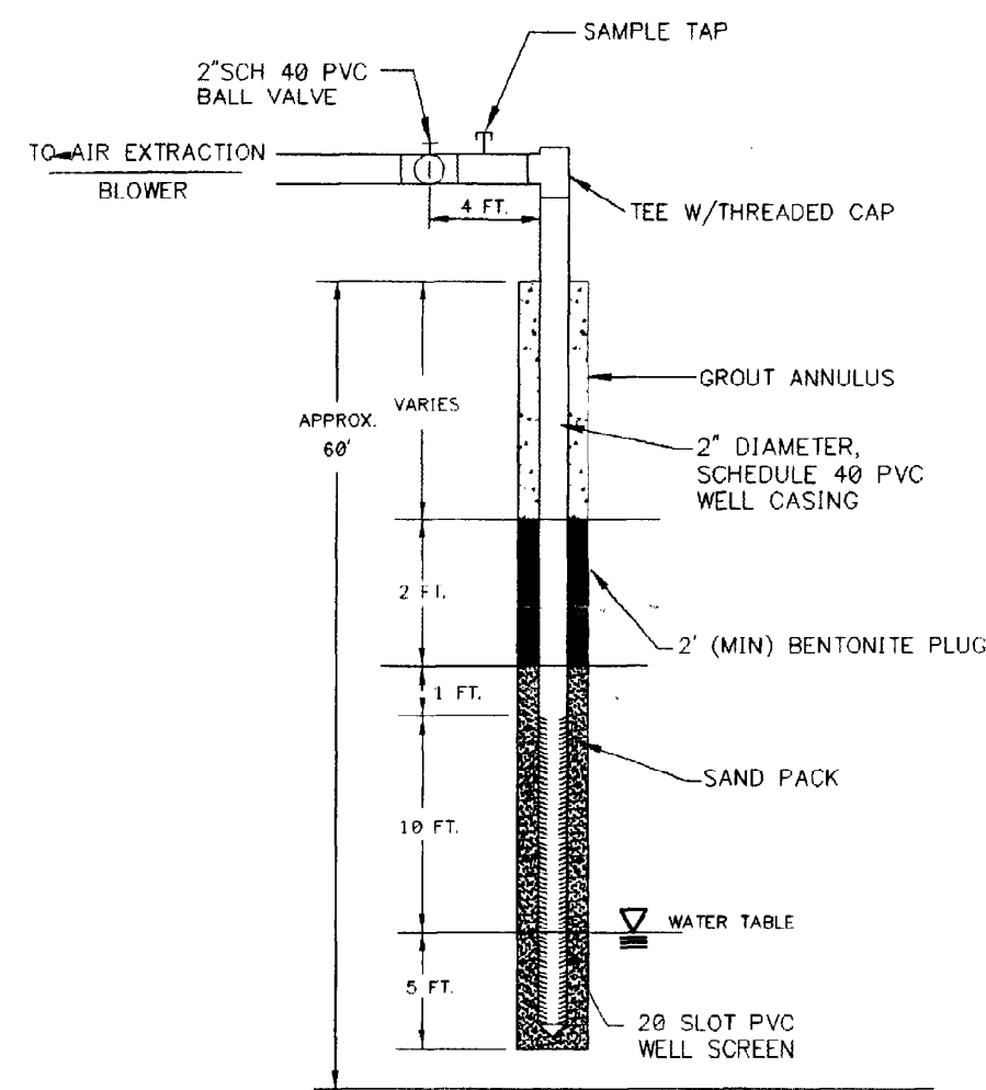
EXTRACTION WELL DETAIL (TYPICAL) NOT TO SCALE
