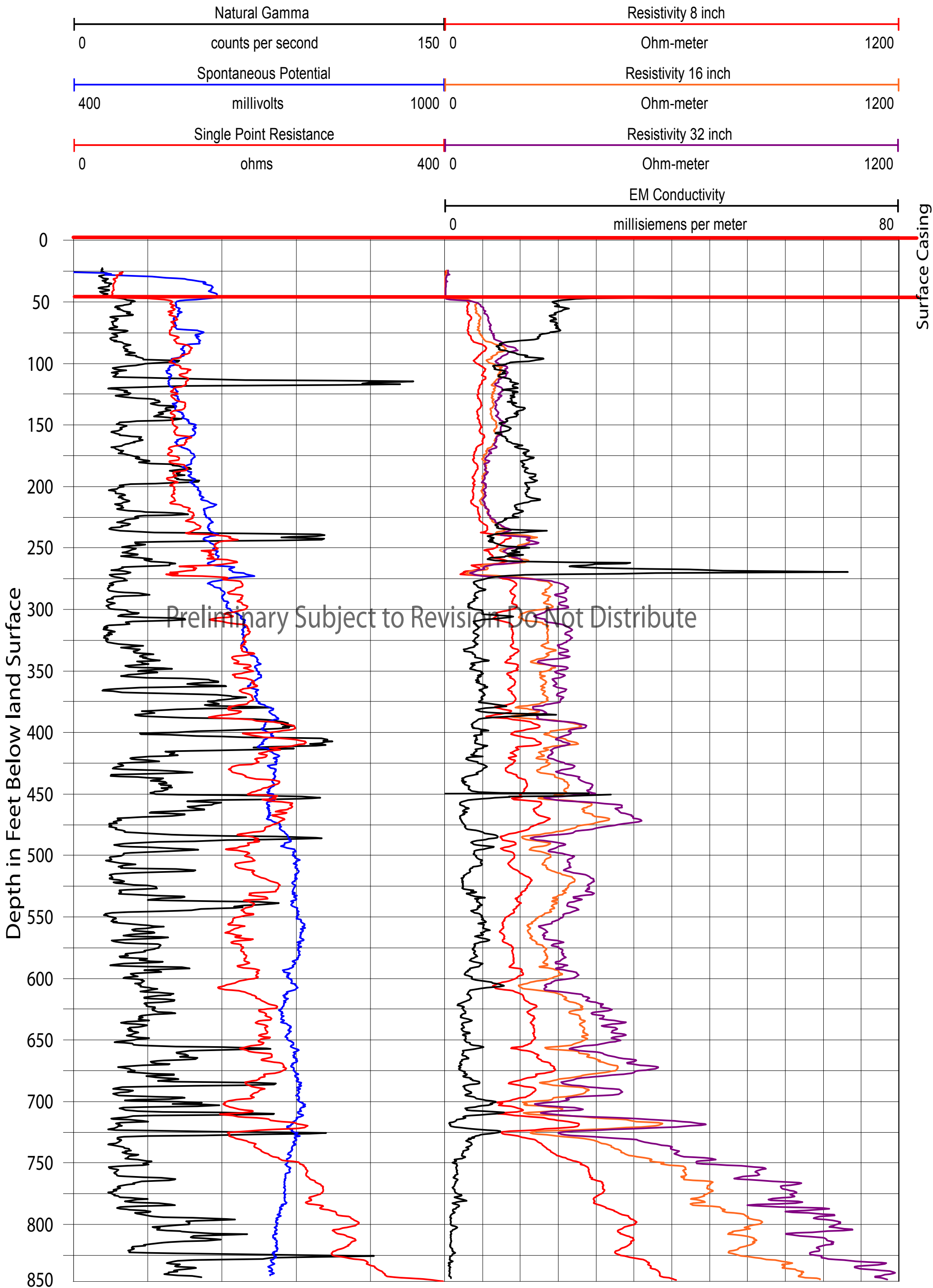
Suite of borehole geophysical logs of test boring VPB-129 Bethpage, NY.
