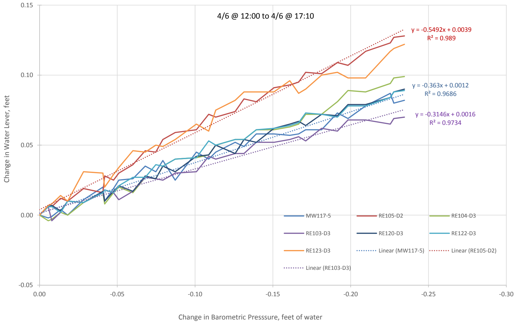
Figure A-17. Period C - Change in Barometric Pressure vs Change in WLS
