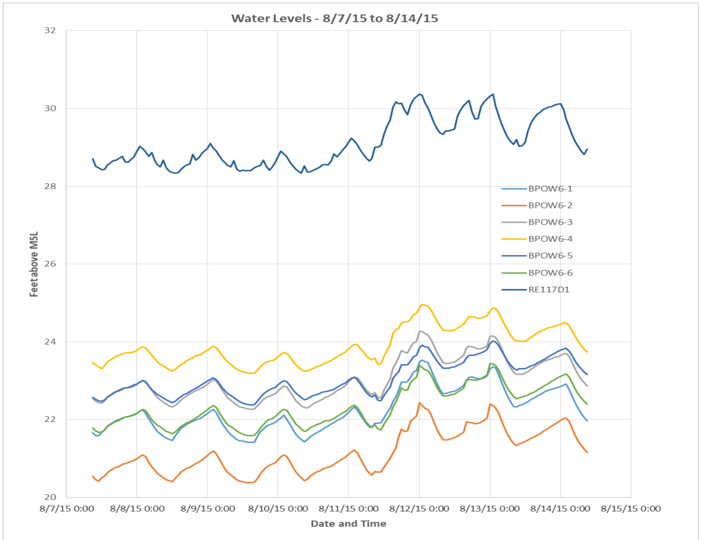
Figure 3. Time Series Hydrograph of Water Levels in RE117D1 and BPOW6 Wells – Focused Range
