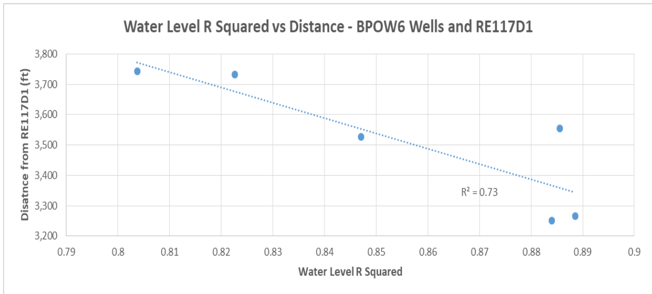
Figure 11. Relationship Between the Water Level R-Squared Values and Distance From RE117D1
