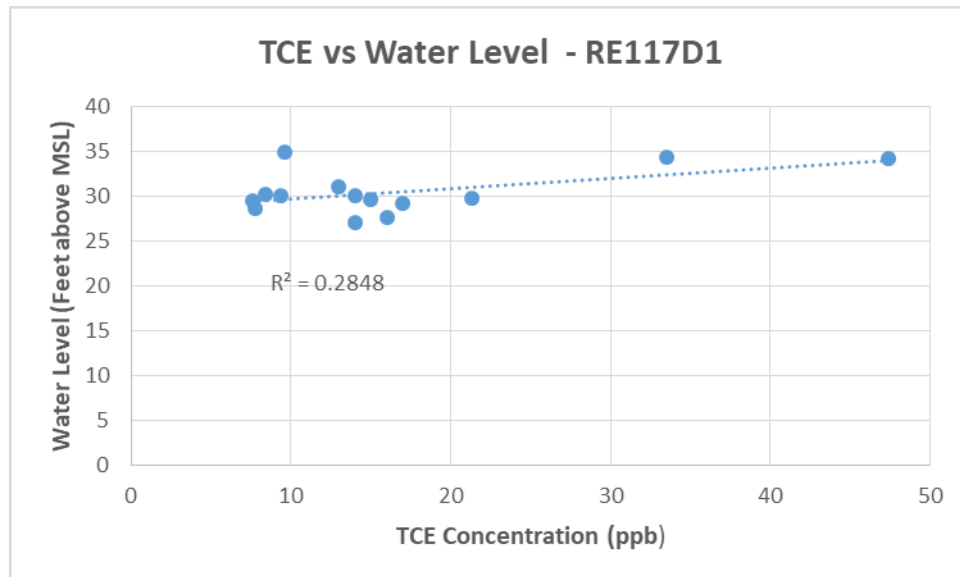
Figure 12. Relationship Between Water Level and TCE Concentration – RE117D1
