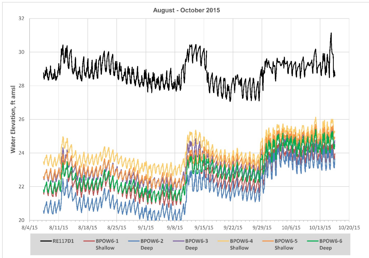
Figure 2. Time Series Hydrograph of Water Levels in the RE117D1 and BPOW6 Series Wells.
