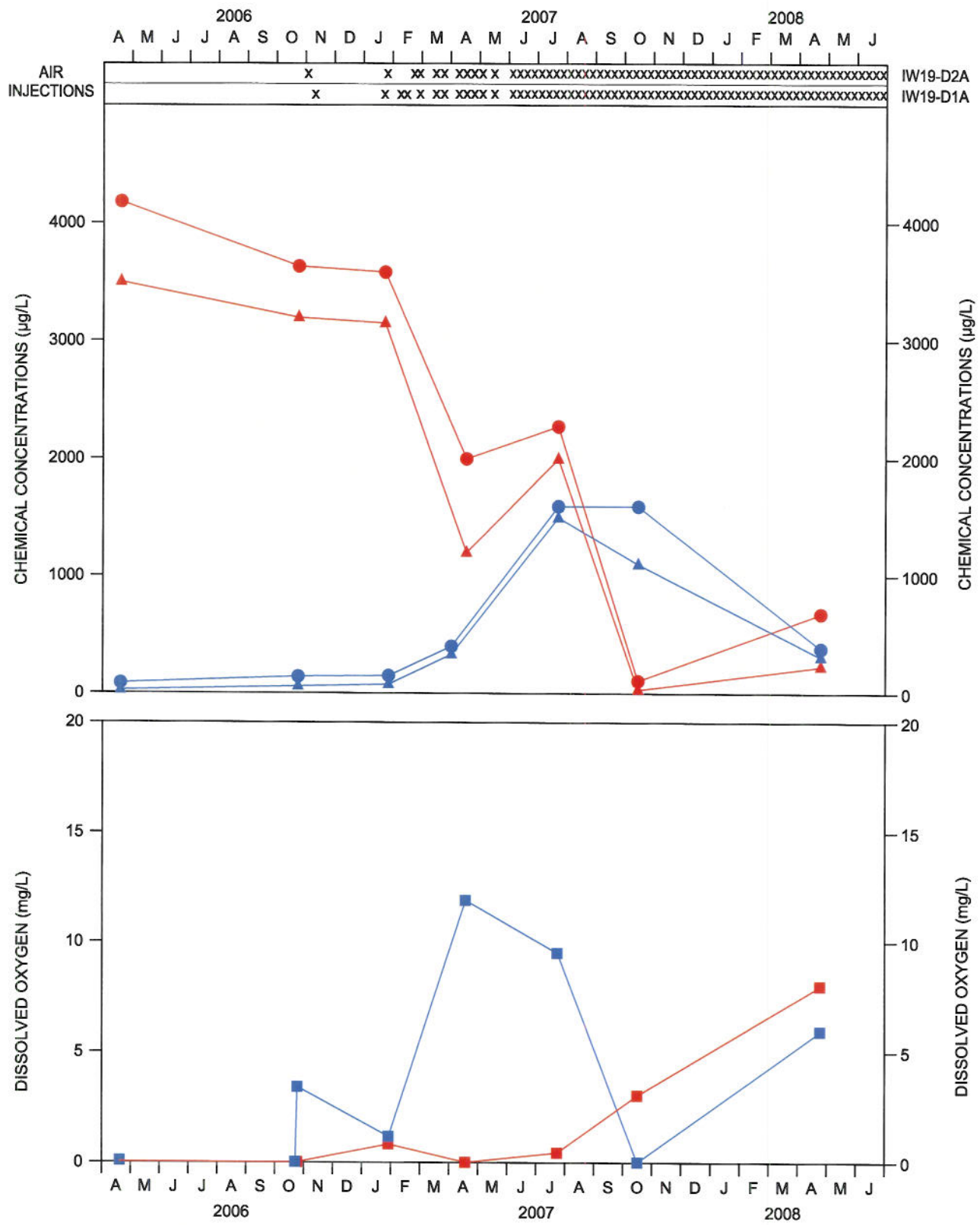
WELL NEST MW-88 CHEMICAL CONCENTRATION PLOTS MIDDLE INJECTION FENCELINE Hooker/Ruco Site, Hicksville, New York
