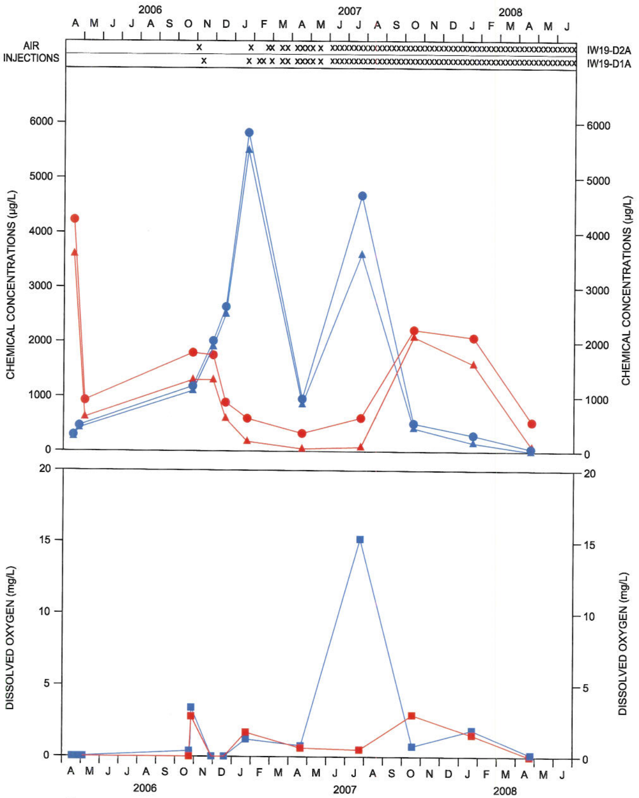
WELL NEST MW-82 CHEMICAL CONCENTRATION PLOTS MIDDLE INJECTION FENCELINE Hooker/Ruco Site, Hicksville, New York
