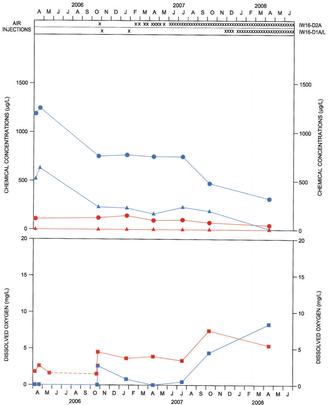
WELL NEST MW-87 CHEMICAL CONCENTRATION PLOTS MIDDLE INJECTION FENCELINE Hooker/Ruco Site, Hicksville, New York
