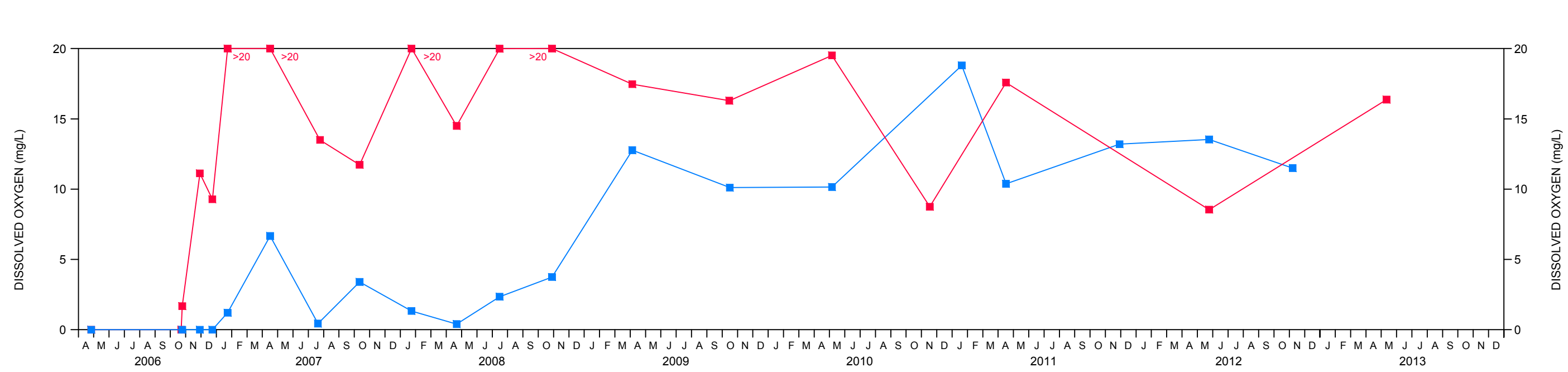
figure 5 WELL NEST MW-61 CHEMICAL CONCENTRATION PLOTS MIDDLE INJECTION FENCELINE Hooker/Ruco Site, Hicksville, New York
