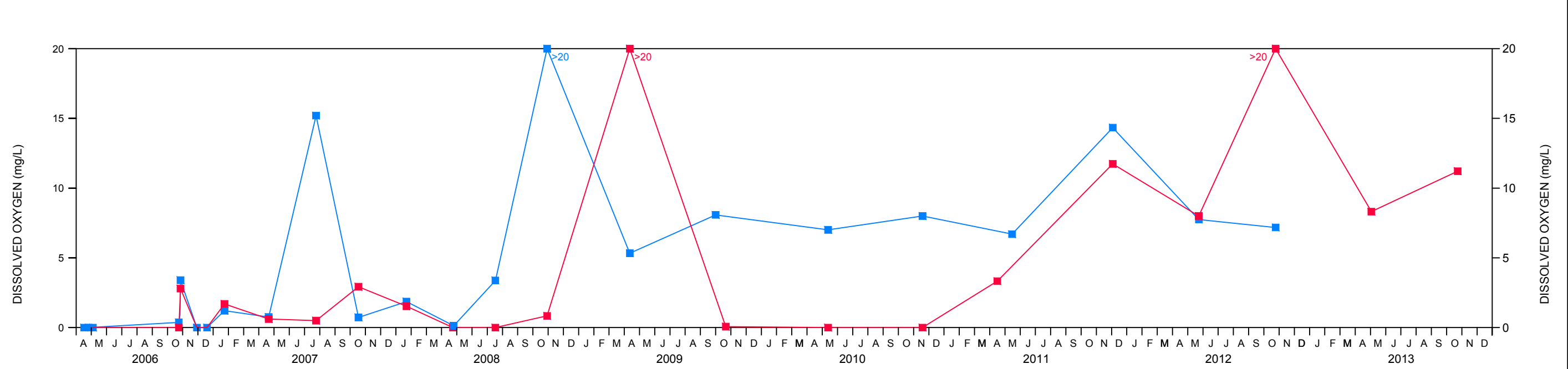
figure 7 WELL NEST MW-82 CHEMICAL CONCENTRATION PLOTS MIDDLE INJECTION FENCELINE Hooker/Ruco Site, Hicksville, New York
