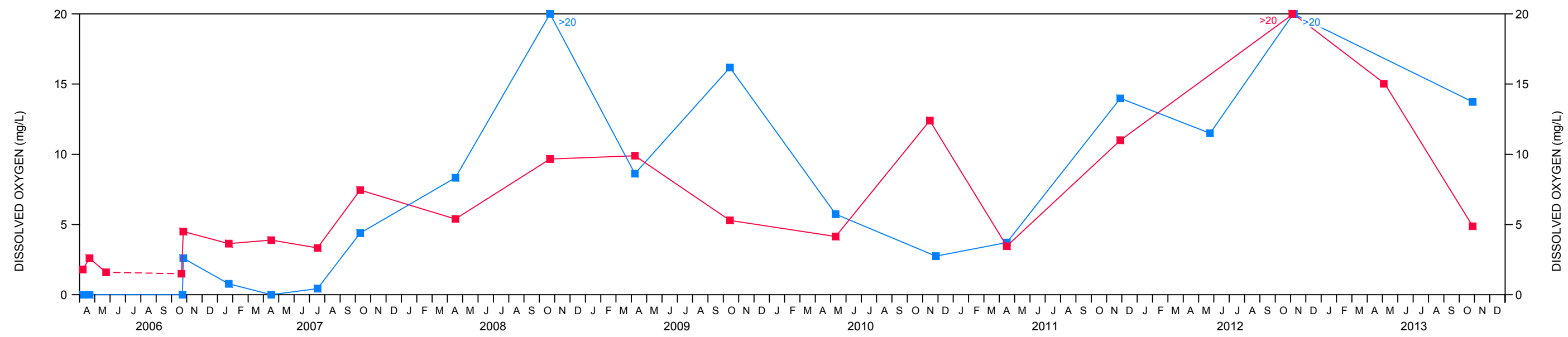
figure 10 WELL NEST MW-87 CHEMICAL CONCENTRATION PLOTS MIDDLE INJECTION FENCELINE Hooker/Ruco Site, Hicksville, New York
