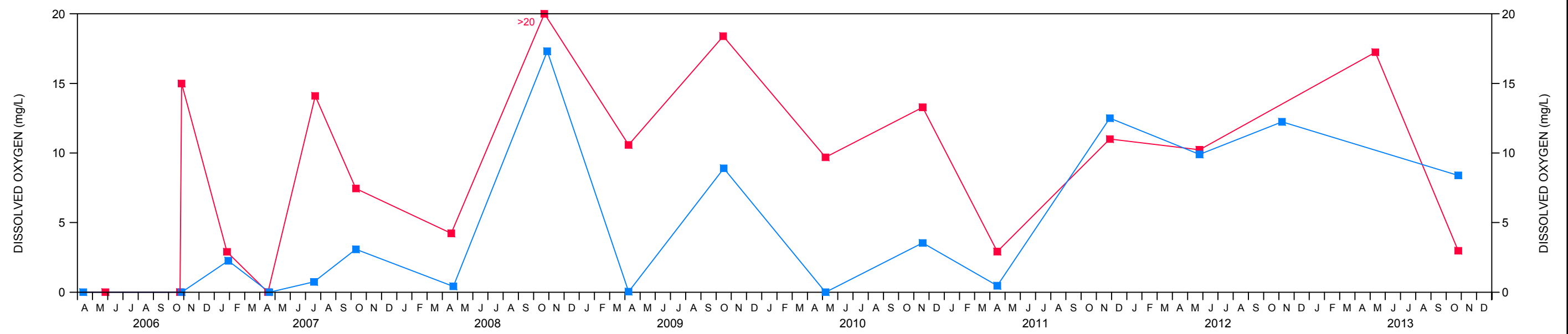
figure 6 WELL NEST MW-81 CHEMICAL CONCENTRATION PLOTS MIDDLE INJECTION FENCELINE Hooker/Ruco Site, Hicksville, New York
