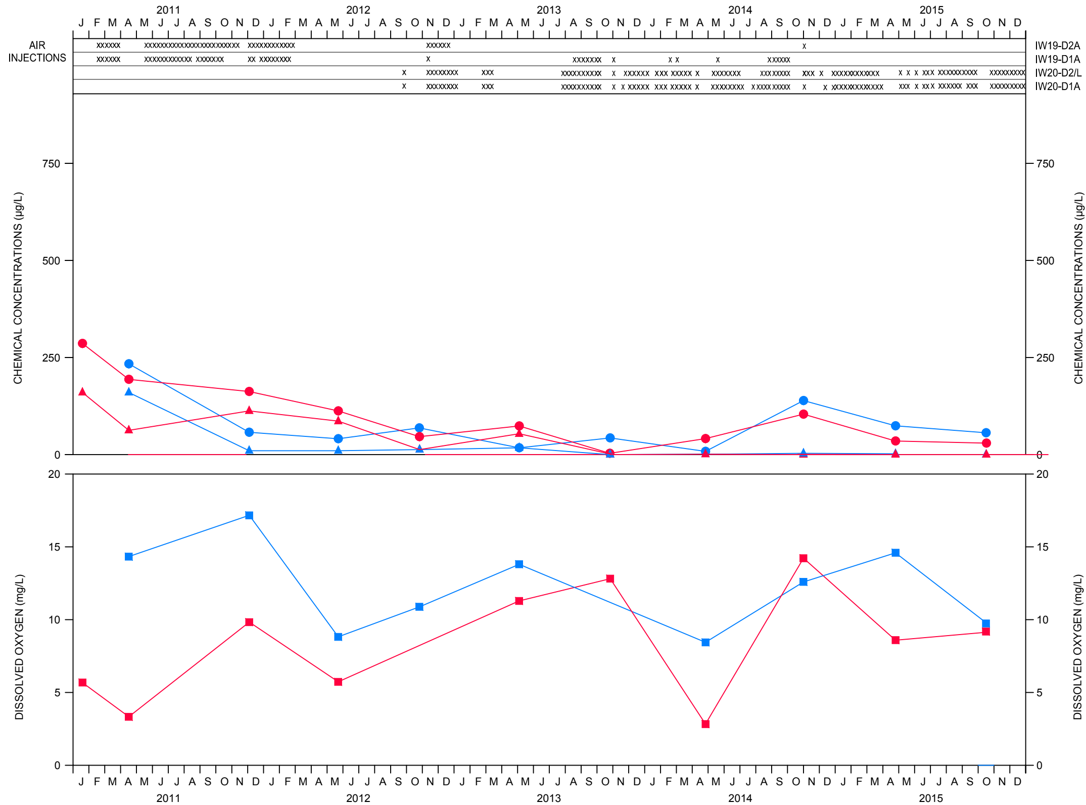
figure 11 WELL NEST MW-88 CHEMICAL CONCENTRATION PLOTS MIDDLE INJECTION FENCELINE Hooker/Ruco Site, Hicksville, New York
