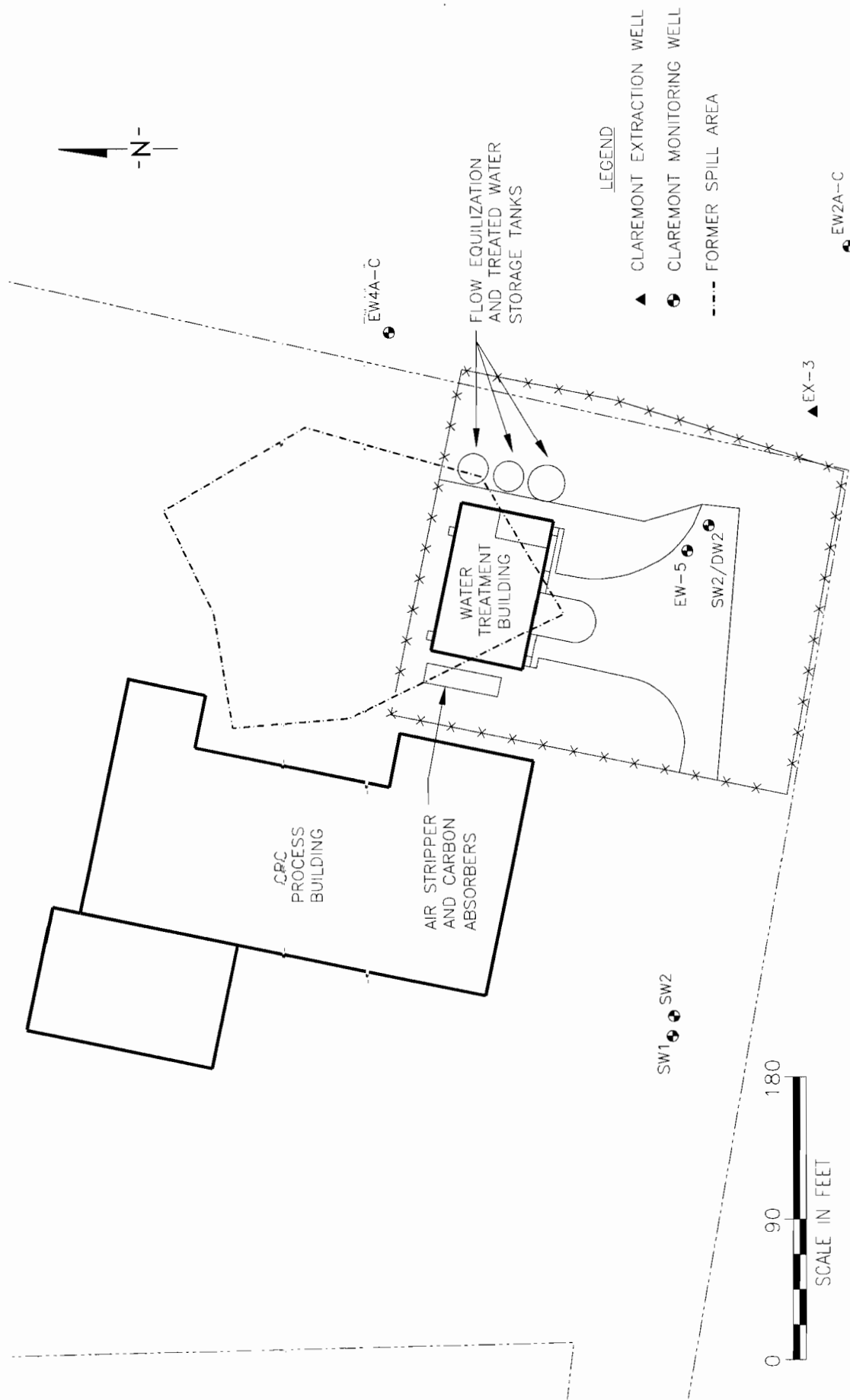
FIGURE 1-3. THE CLAREMONT POLYCHEMICAL SITE INCLUDING SELECT WELLS, SITE BUILDINGS, AND THE FORMER SPILL AREA.
