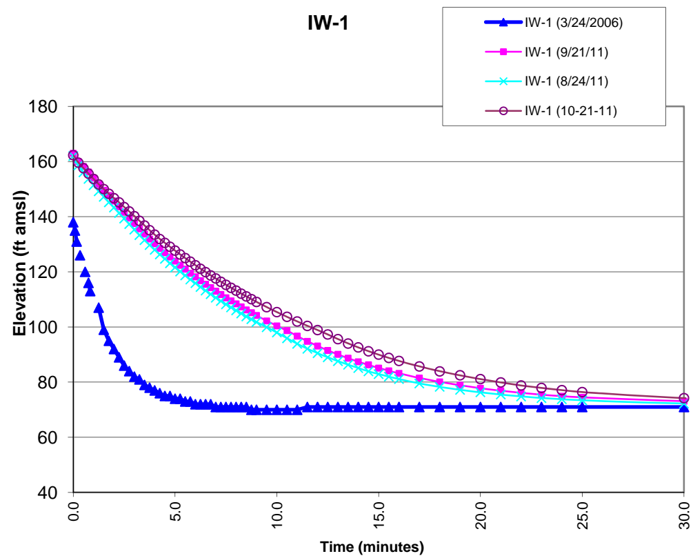
Figure 14-3 Comparison of Falling Head Tests
