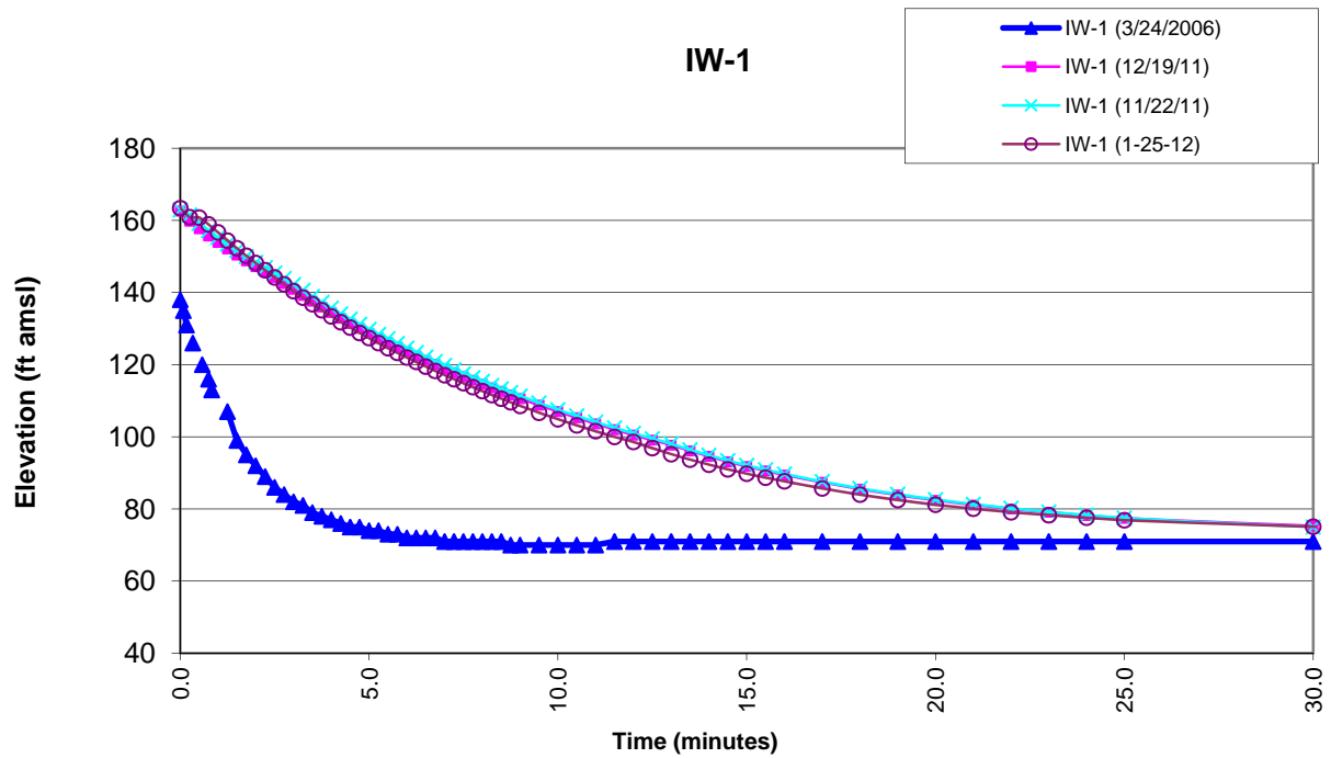
Figure 14-3 Comparison of Falling Head Tests
