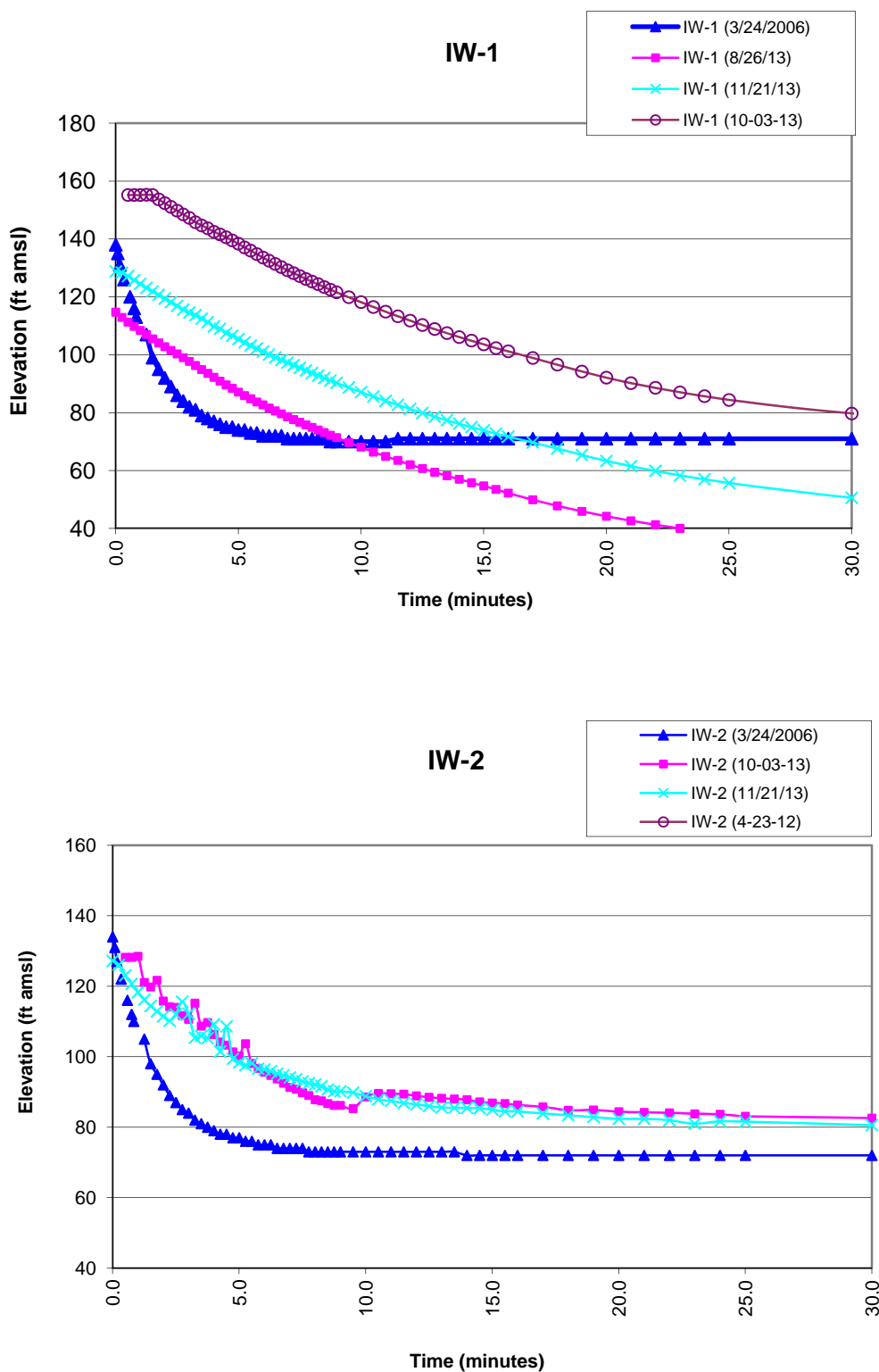
Figure 14-3 Comparison of Falling Head Tests
