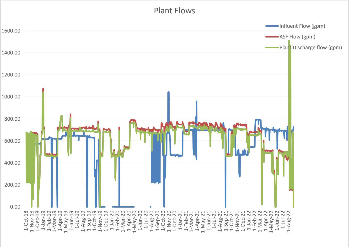
Figure 1 Plant Discharge Daily Flow
