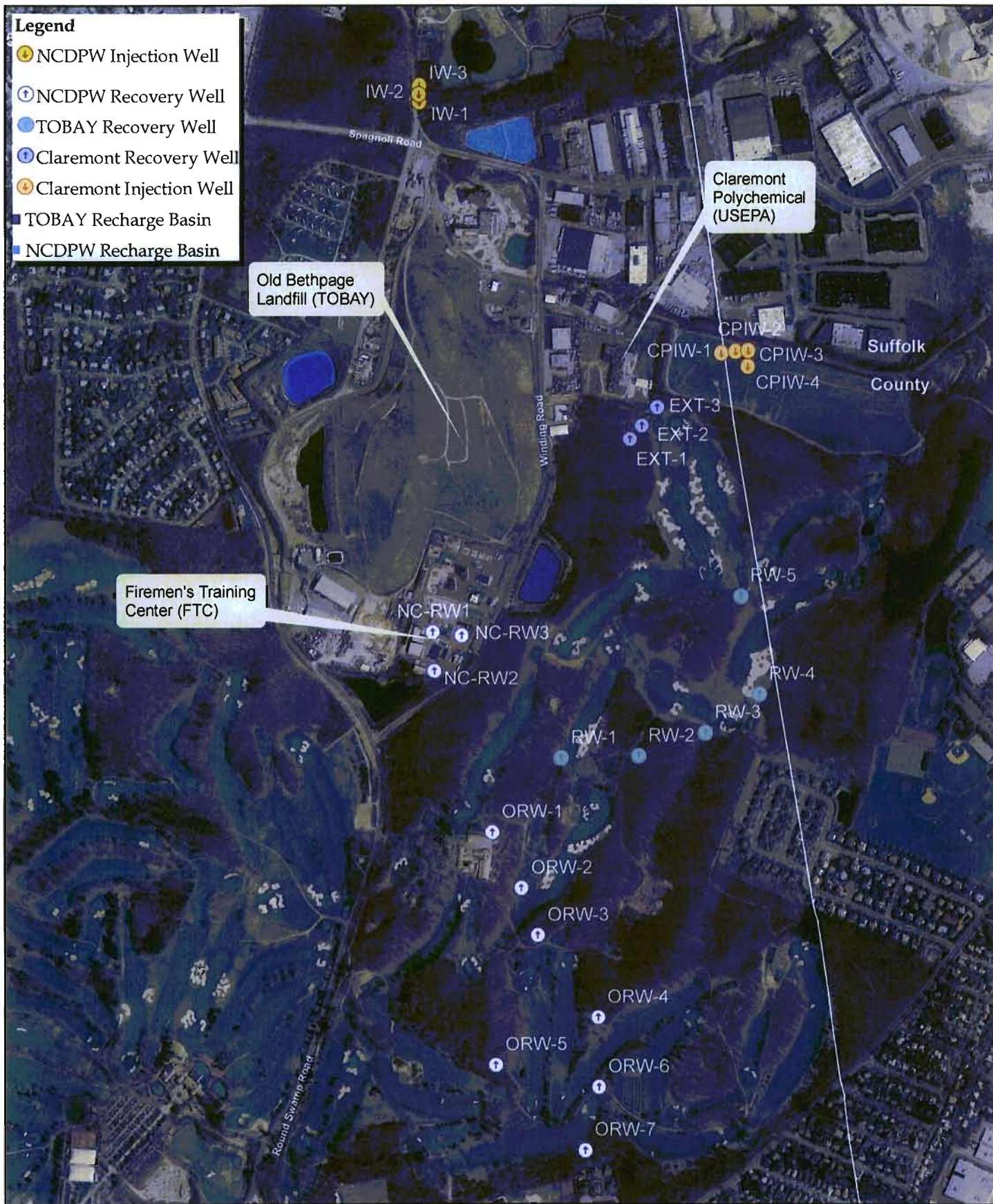
Figure 2-6 Firemen's Training Center Groundwater Model Groundwater Remediation Systems FTC, Old Bethpage Landfill, and Claremont Polychemical CDM
