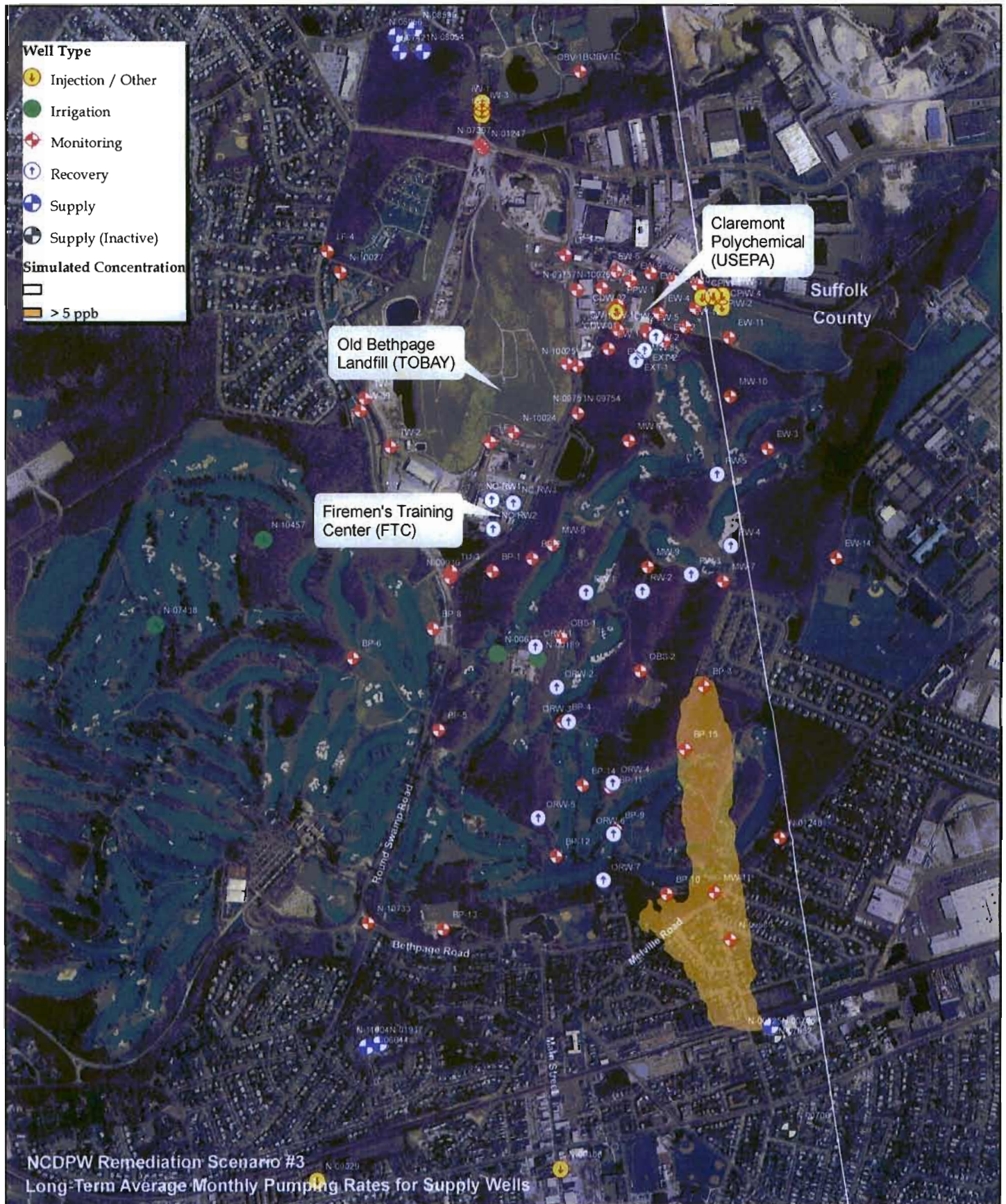
Figure 3-36 Firemen's Training Center Groundwater Model Simulated Contaminant Plume from BP-3C and BP-10C, 2050 Concentrations Fixed at Wells; R = 1.3
