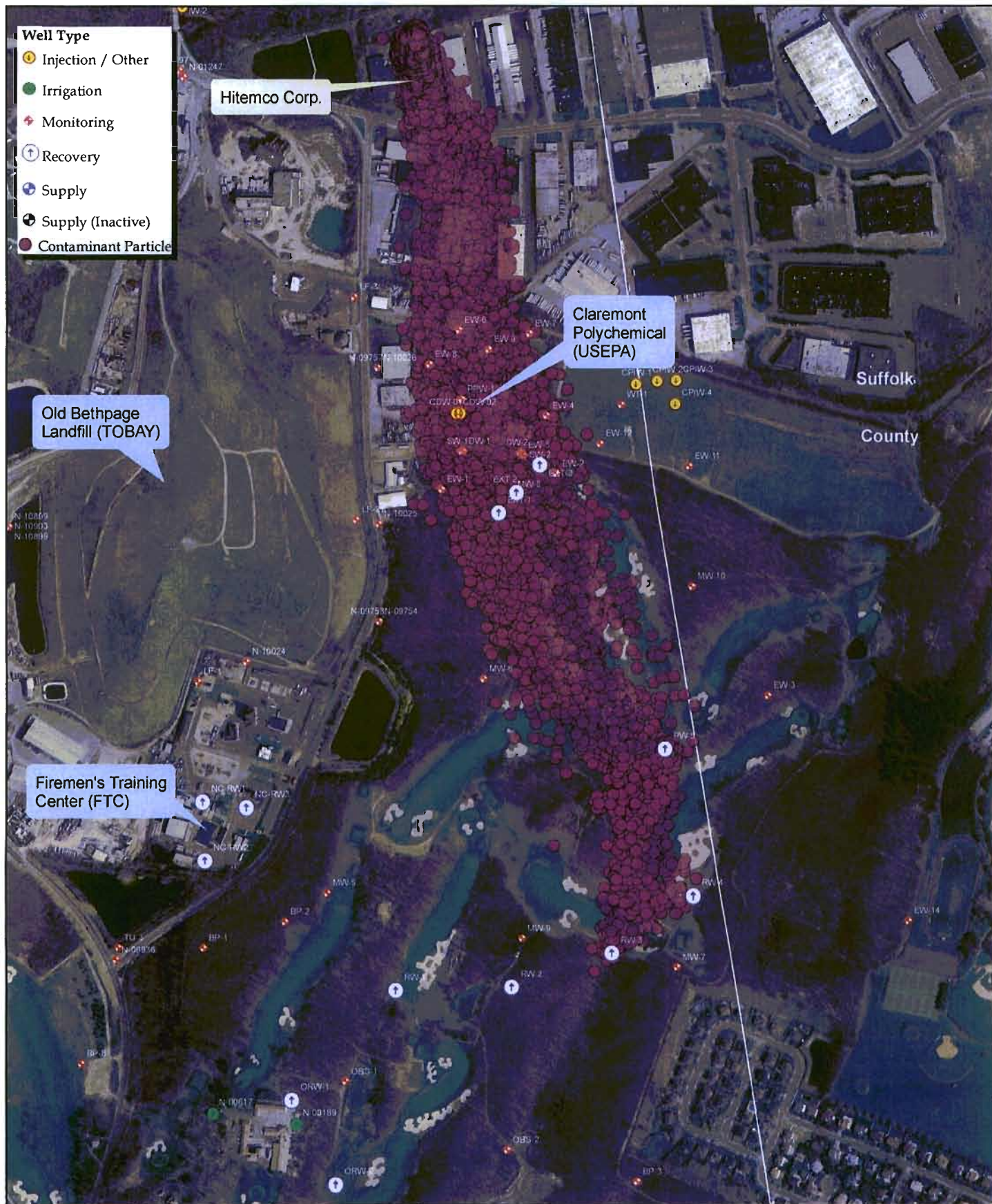
Figure 3-18b Firemen's Training Center Groundwater Model Simulated Plume from Hitemco Corporation Particles Released from Water Table 1981-Present; R = 1.5 CDM
