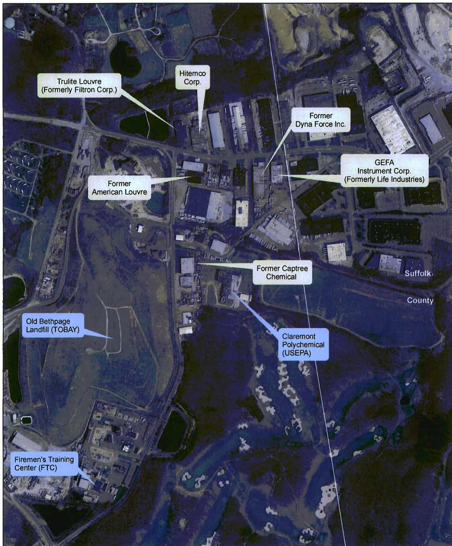
Figure 3-14 Firemen's Training Center Groundwater Model Potential Upgradient Sources from FTC Nassau County
