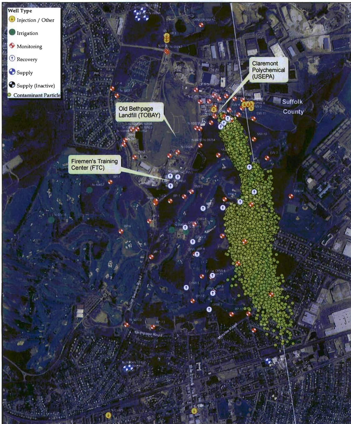
Figure 3-13b Firemen's Training Center Groundwater Model Simulated Plume from Water Table at Claremont Particles Released 1968-1997; Retardation = 1.5
