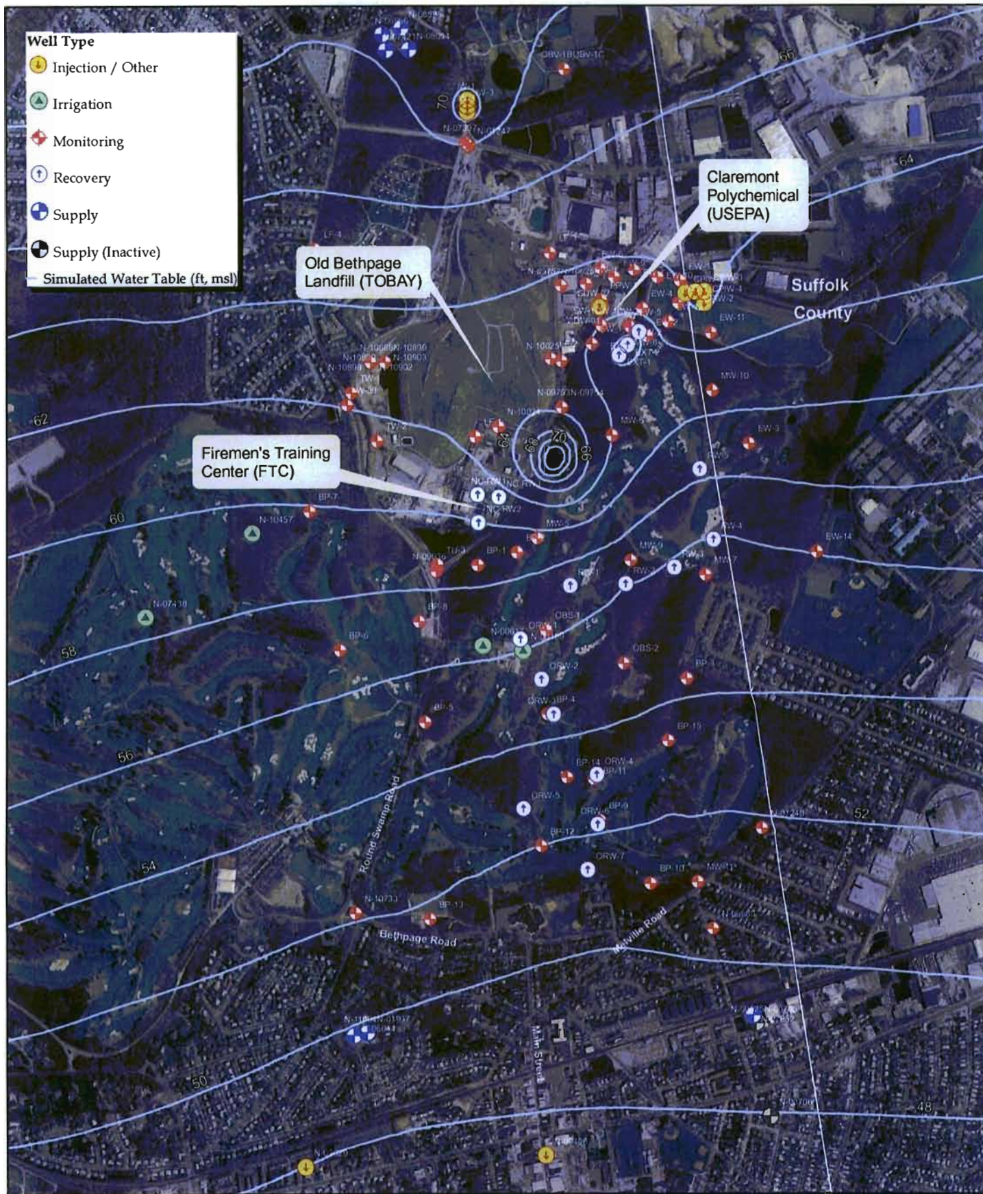
Figure 2-10 Firemen's Training Center Groundwater Model Simulated Water Table Transient Simulation: April 2003
