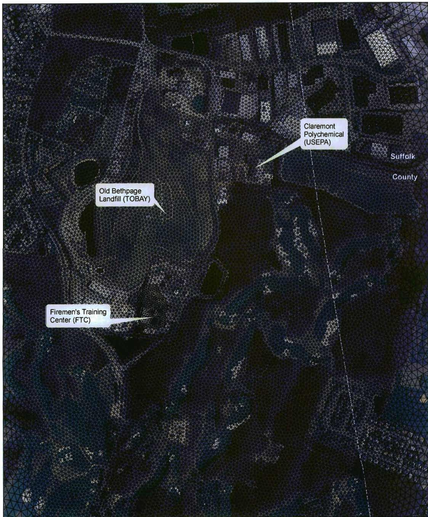
Figure 2-2 Firemen's Training Center Groundwater Model Finite Element Grid Fine Node Discretization within Study Area
