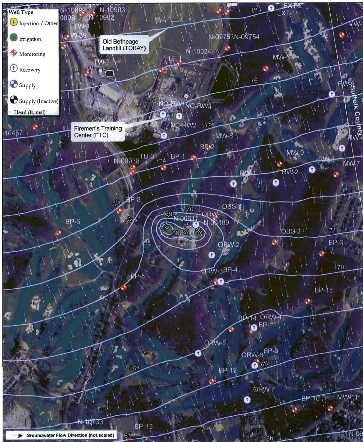
Figure 3-24 Firemen's Training Center Groundwater Model Influence of Bethpage Irrigation Wells Simulated Groundwater Head at Well Screens - July 1980
