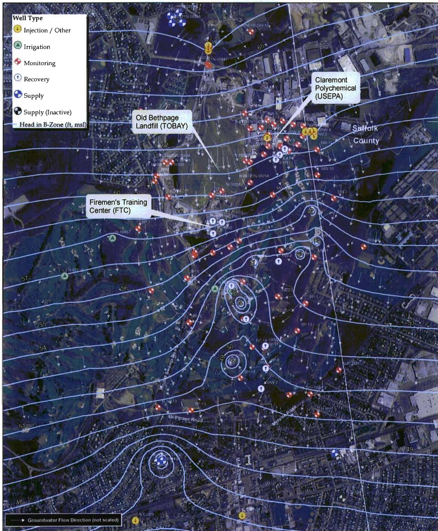
Figure 2-11 Firemen's Training Center Groundwater Model Simulated Head in B-Zone Transient Simulation: April 2003
