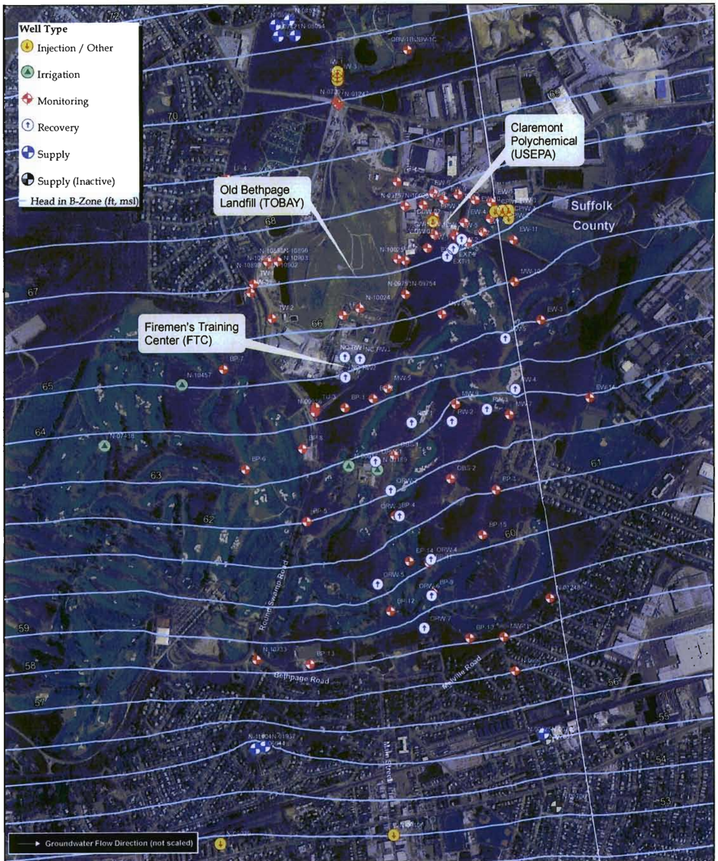
Figure 2-9 Firemen's Training Center Groundwater Model Simulated Head in B-Zone March 1992 Steady-State Simulation
