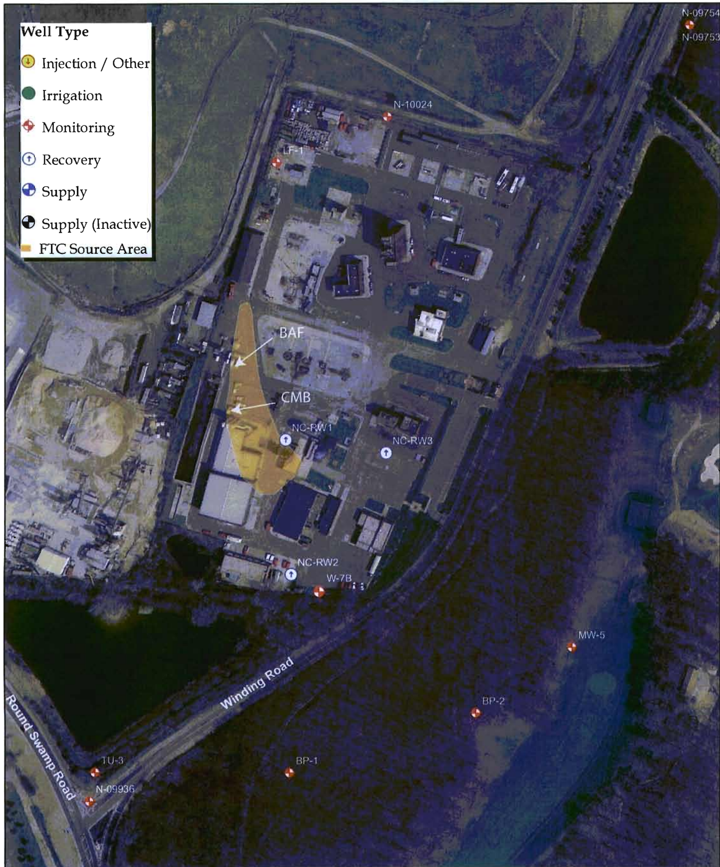
Figure 3-2 Firemen's Training Center Groundwater Model Source Area for Contamination at FTC Facility
