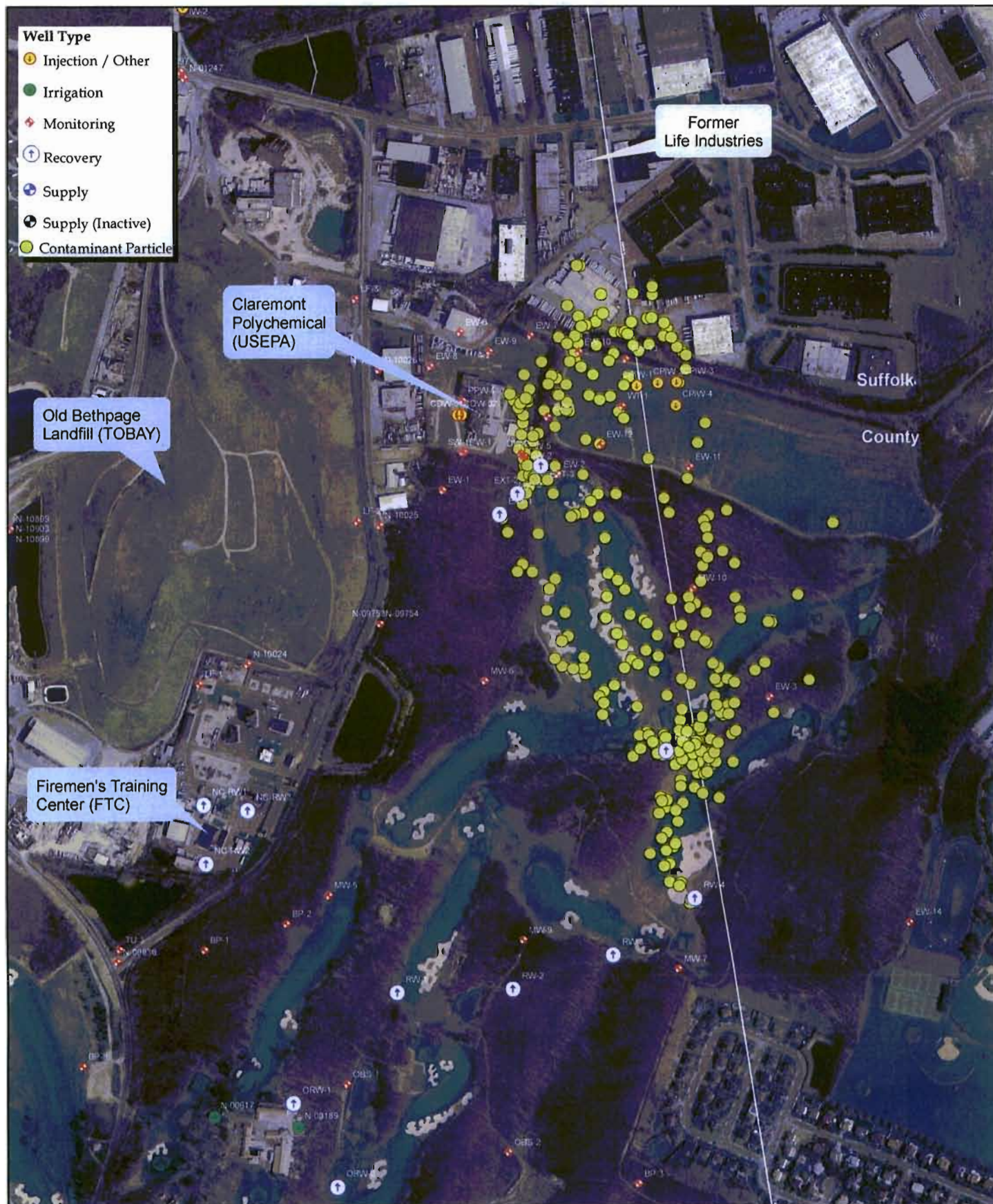
Figure 3-20 Firemen's Training Center Groundwater Model Simulated Plume from Former Life Industries Particles Released from Water Table 1983-1996; R = 1.5
