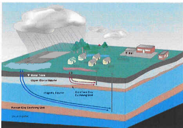
Figure 3-11 Example of well contributing areas (from Long Island Source Water Assessment Program, NYSDOH, 2003)
