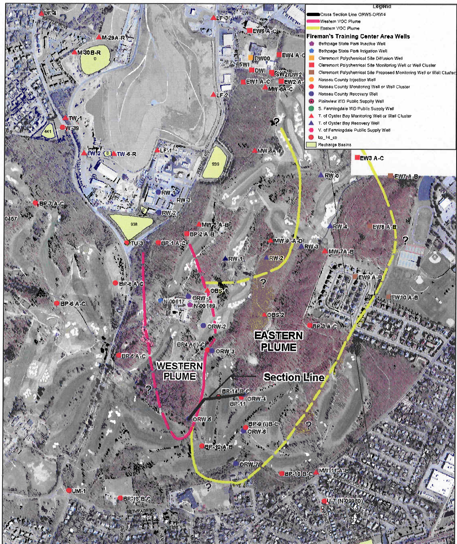
Figure 1-1 Firemen's Training Center Groundwater Model Eastern and Western Plume Extent Plume Extents Mapped by NCDPW (2004)
