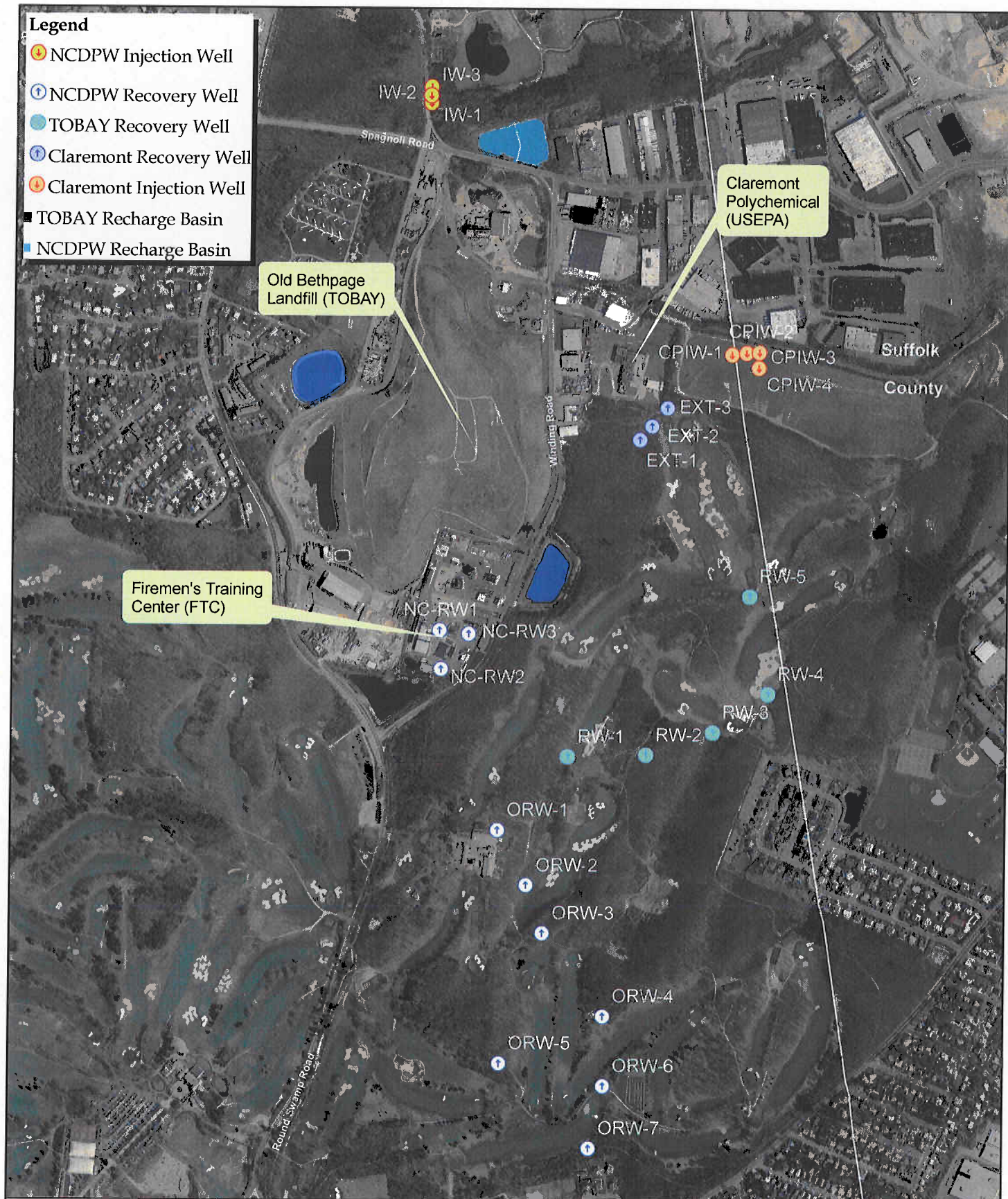
Figure 2-6 Firemen's Training Center Groundwater Model Groundwater Remediation Systems FTC, Old Bethpage Landfill, and Claremont Polychemical
