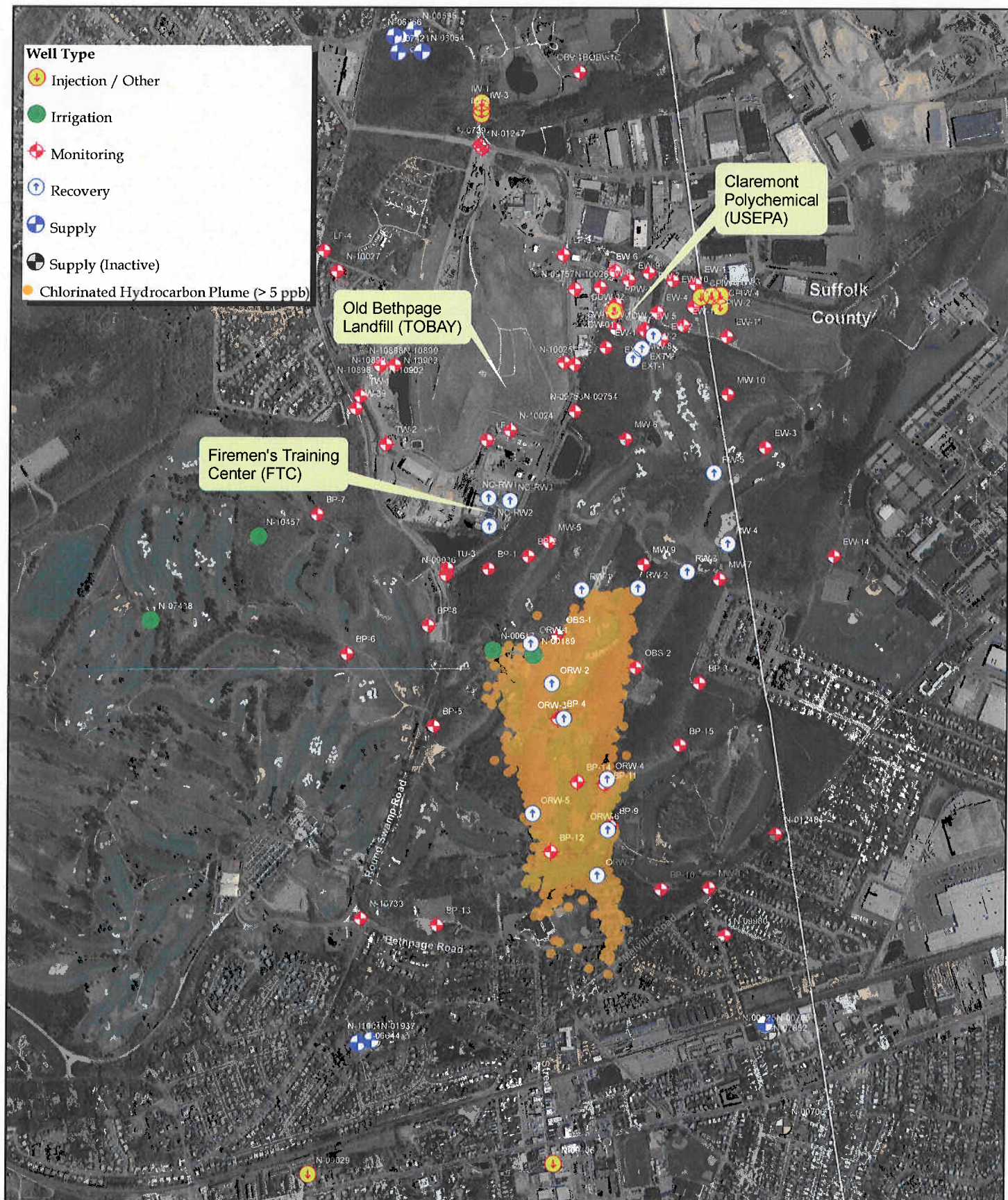
Figure 3-5 Firemen's Training Center Groundwater Model Simulated Chlorinated Hydrocarbon Plume from FTC, 2005 Continuous Source of 3,000 ppb, 1966-1985
