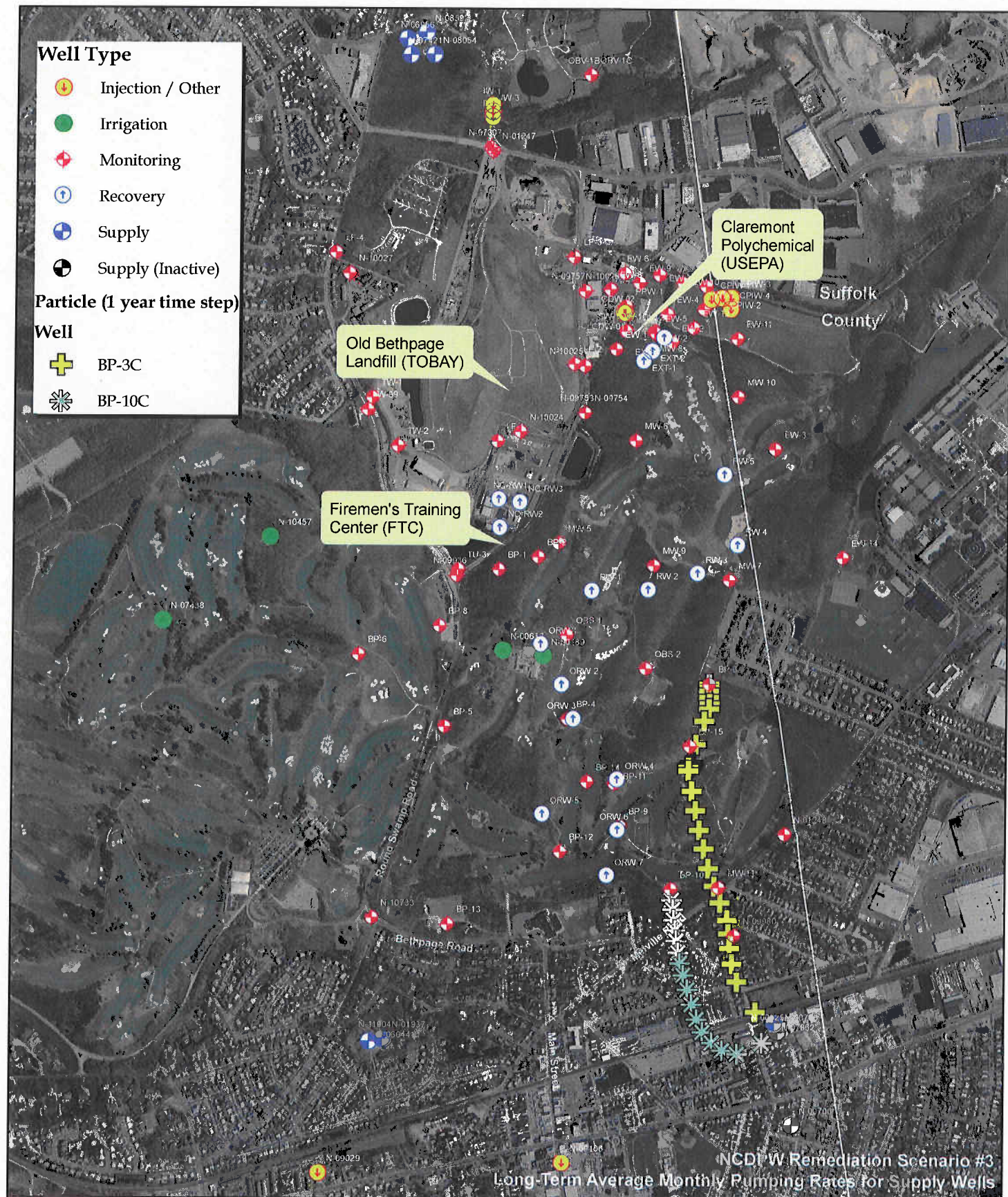
Figure 3-35a Firemen's Training Center Groundwater Model Forward Particle Tracks from C-Zone; No Retardation Particles Released from BP-3C (1996) & BP-10C (2005)
