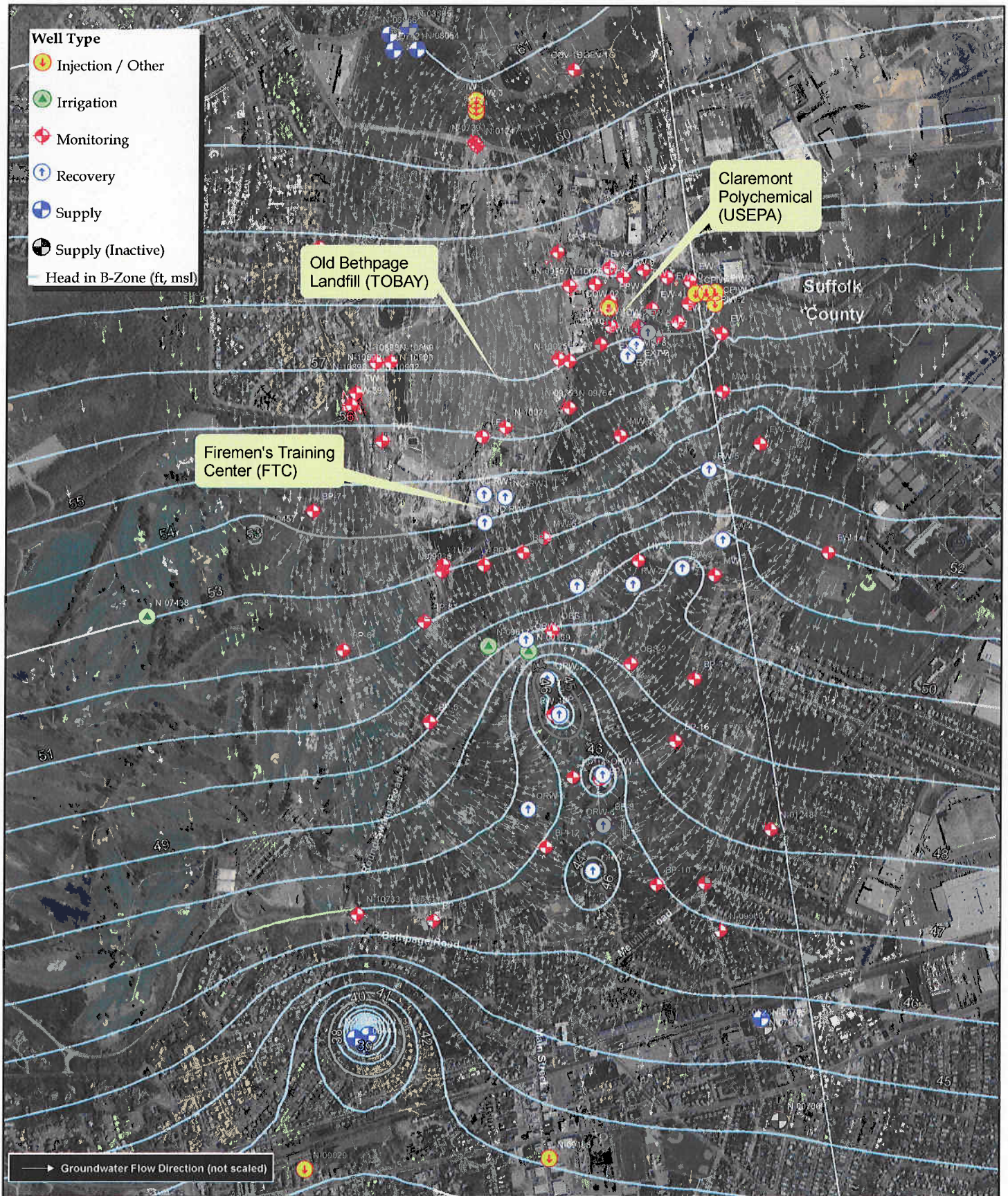
Figure 3-9a Firemen's Training Center Groundwater Model Simulated Head in B-Zone Transient Simulation: October 2002
