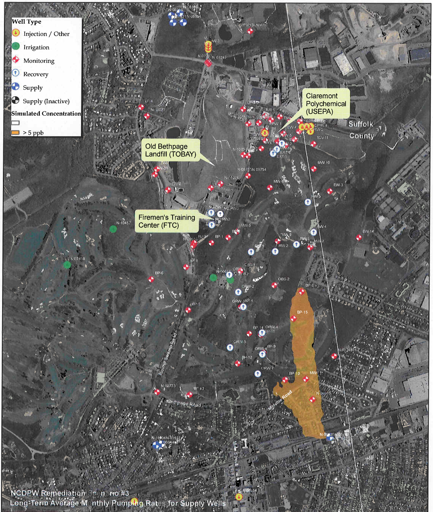
Figure 3-36 Firemen's Training Center Groundwater Model Simulated Contaminant Plume from BP-3C and BP-10C, 2050 Concentrations Fixed at Wells; R = 1.3 CDM
