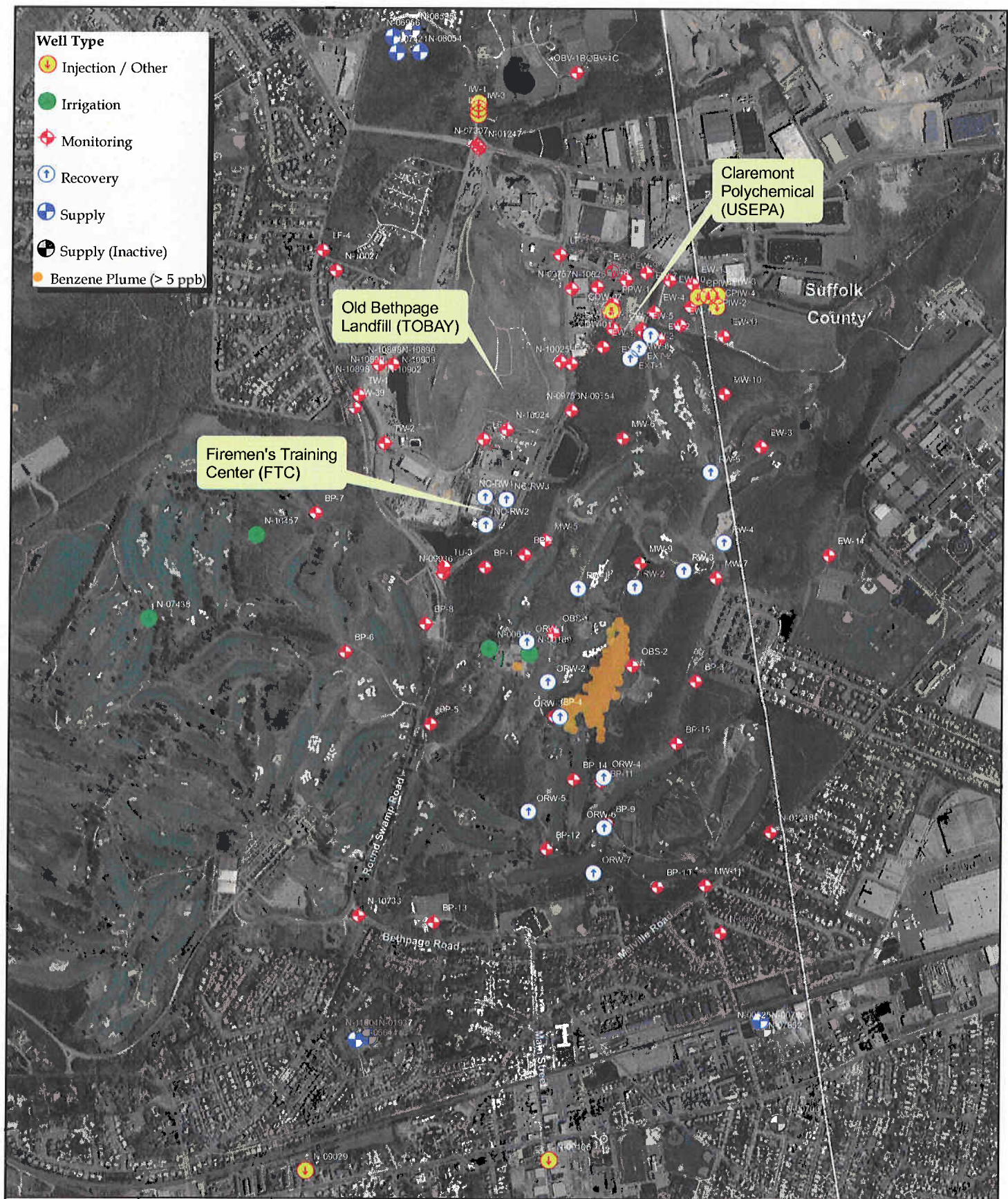
Figure 3-7 Firemen's Training Center Groundwater Model Simulated Benzene Plume from FTC, 2005 Continuous Source of 5,000 ppb, 1966-1992; 500 ppb 1992-2000 CDM
