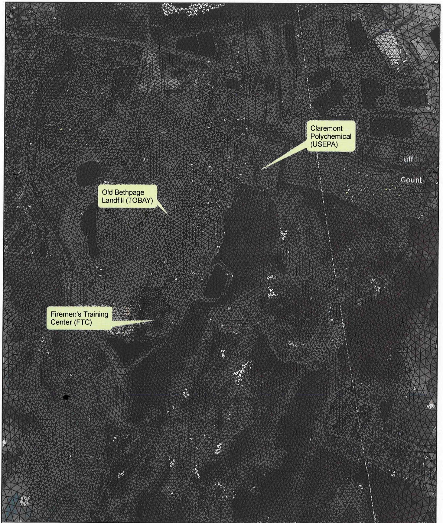
Figure 2-2 Firemen's Training Center Groundwater Model Finite Element Grid Fine Node Discretization within Study Area CDM
