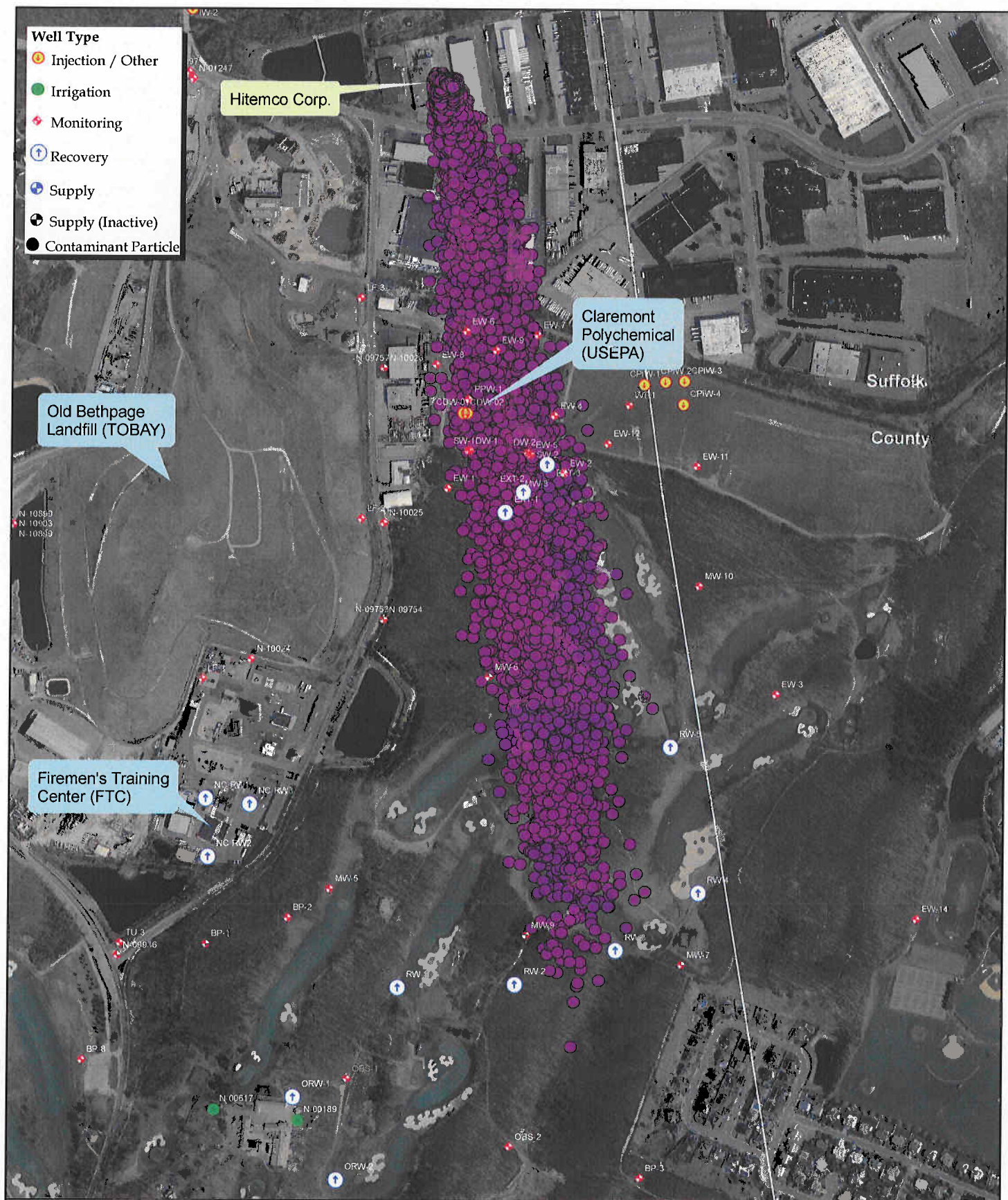
Figure 3-18 Firemen's Training Center Groundwater Model Simulated Plume from Hitemco Corporation Particles Released from Diffusion Well 1981-Present; R = 1.5 CDM
