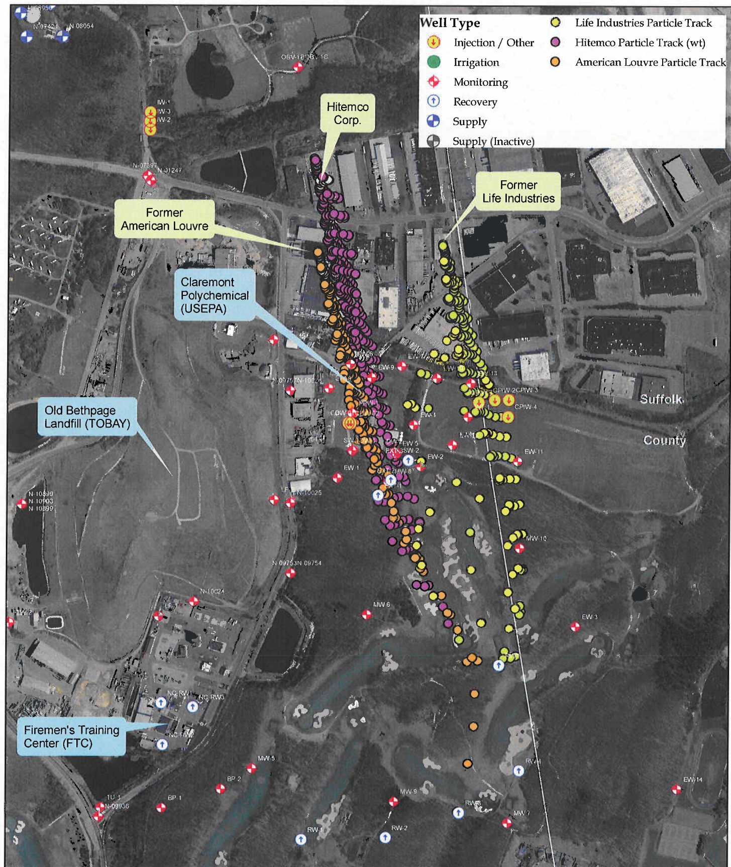
Figure 3-22 Firemen's Training Center Groundwater Model Forward Particle Tracks from American Louvre, Hitemco (Water Table), and Life Industries, 2007
