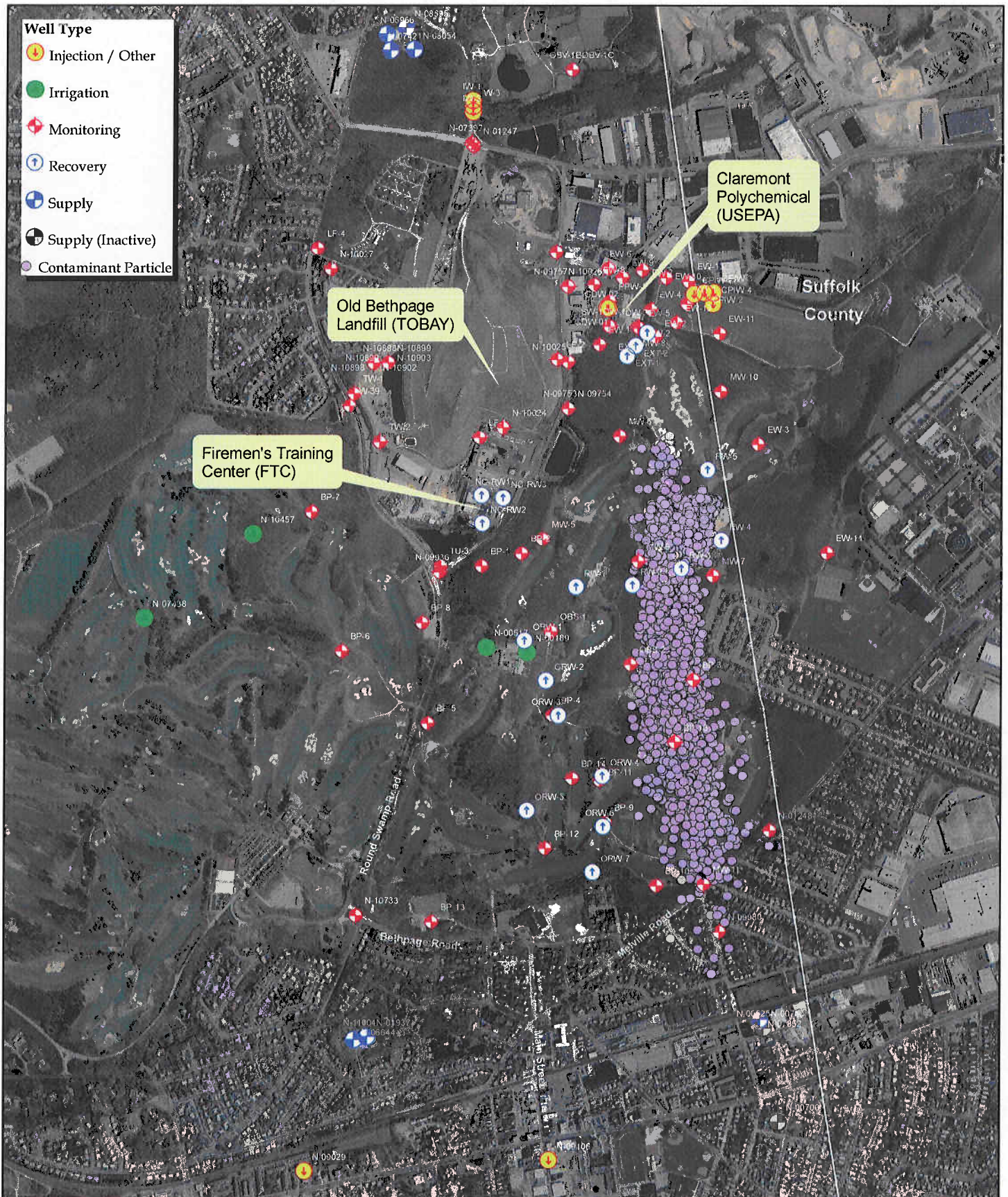
Figure 3-13 Firemen's Training Center Groundwater Model Simulated Plume from Claremont Diffusion Wells Particles Released 1968-1981; Retardation = 1.5
