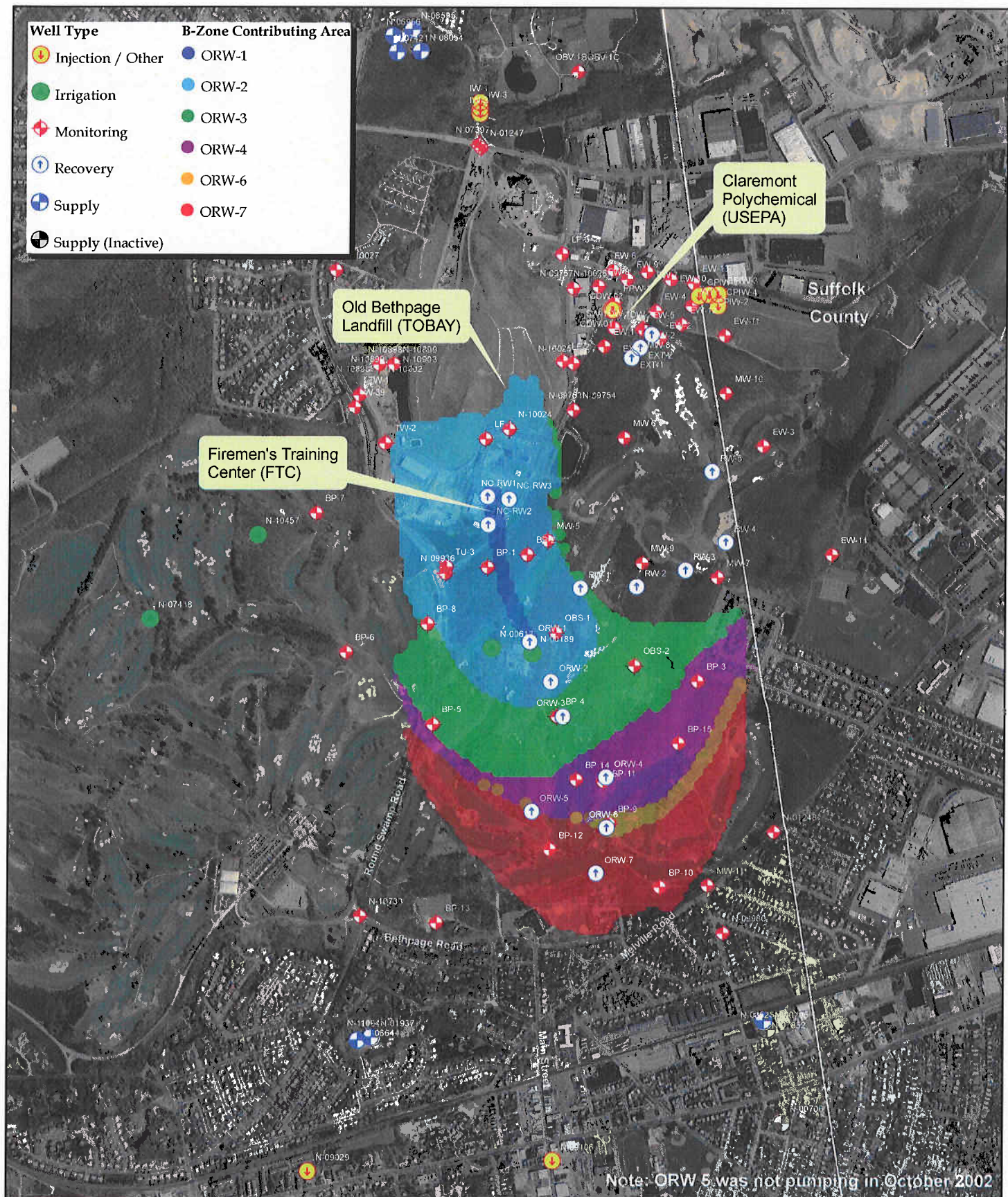
Figure 3-12 Firemen's Training Center Groundwater Model B-Zone Contributing Area to NCDPW Recovery Wells October 2002 Pumping Rates Simulated for 10 Years
