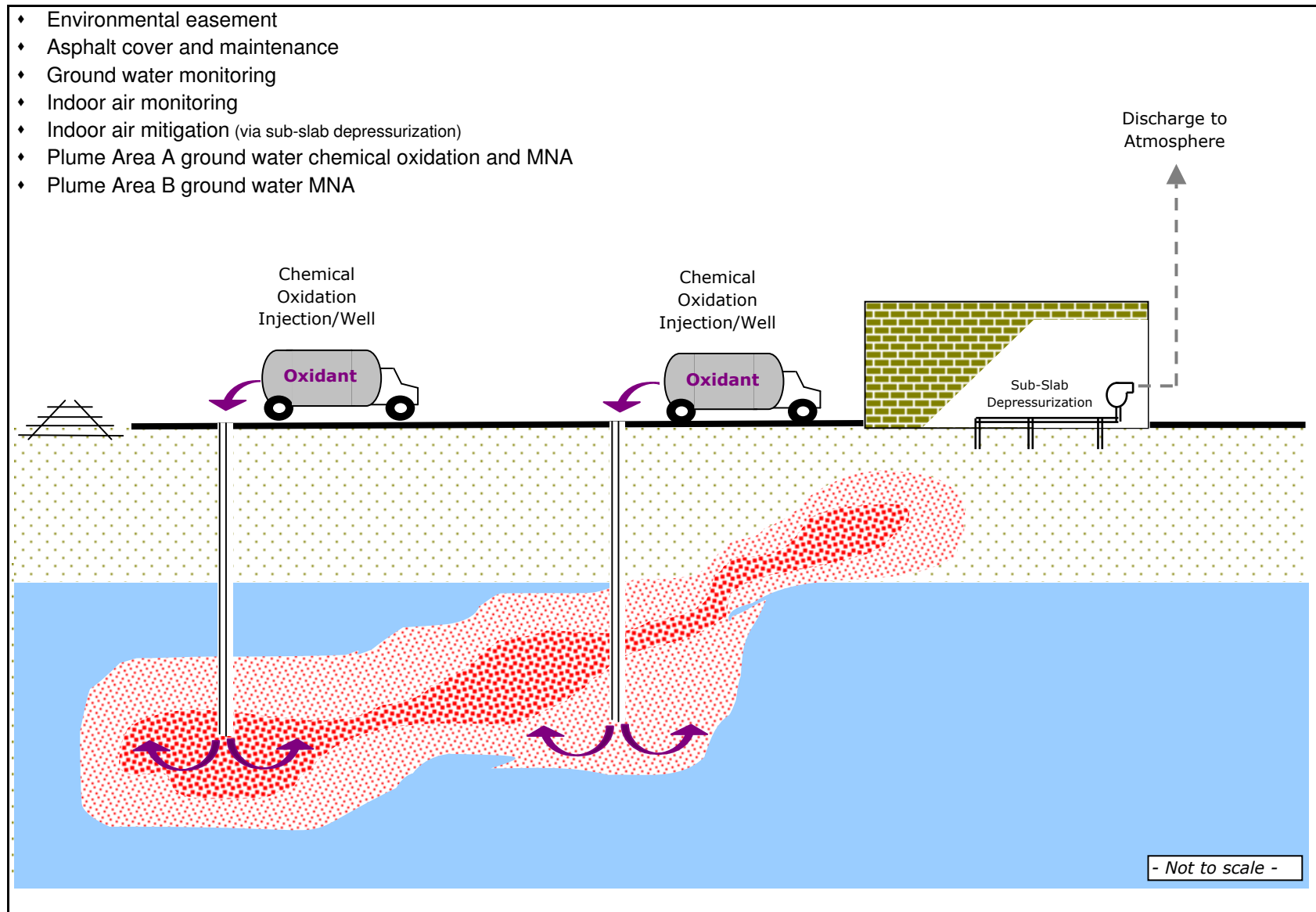
Figure 8. Schematic Diagram of Alternative 2
