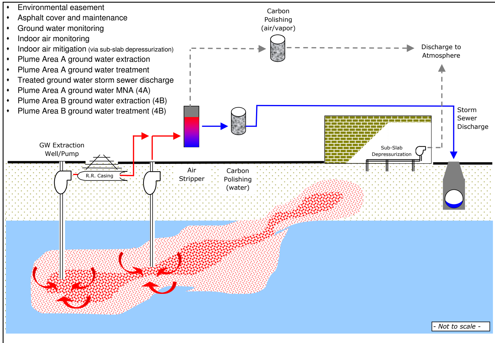
Figure 13. Schematic Diagram of Alternative 4 A/B
