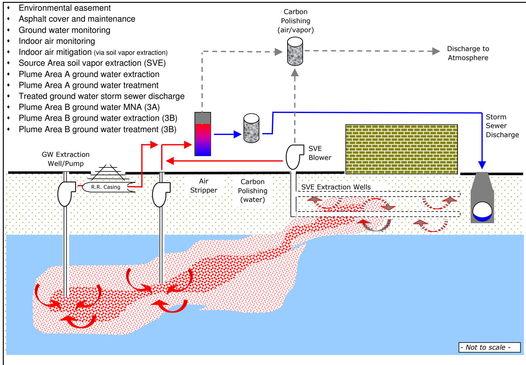
Figure 10. Schematic Diagram of Alternative 3 A/B
