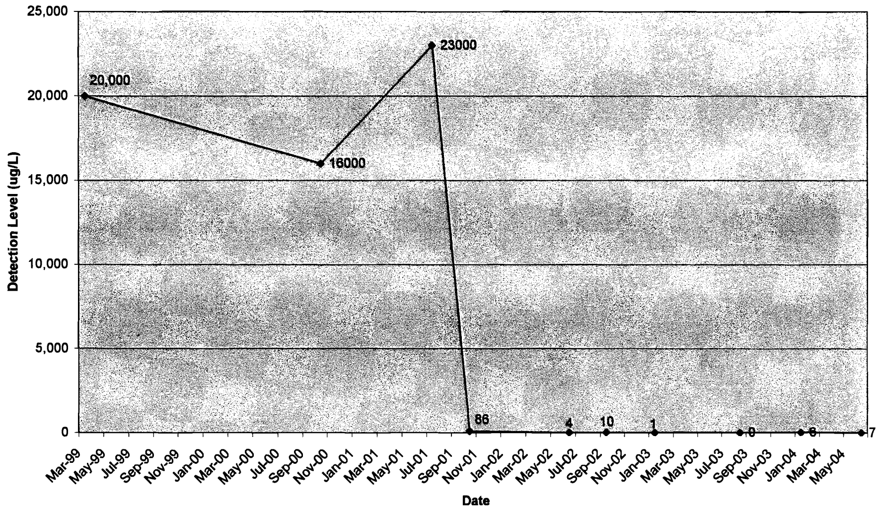
Historic Laboratory Detection Levels for Tetrachloroethene in MW # 3 (ug/L) March 31, 1999 thru June 8, 2004
