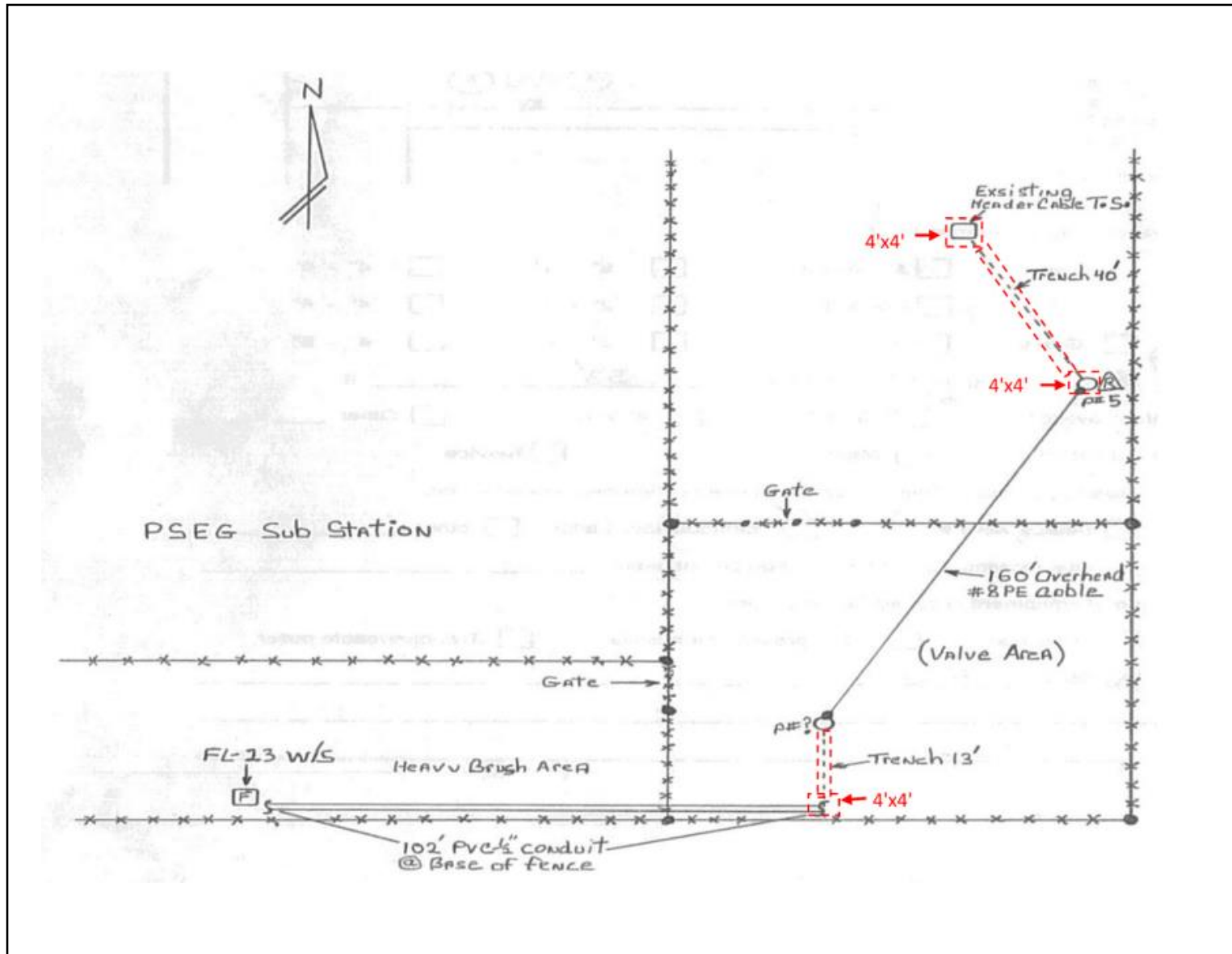
FIGURE 2.0 TRENCH AND PIT LOCATIONS
