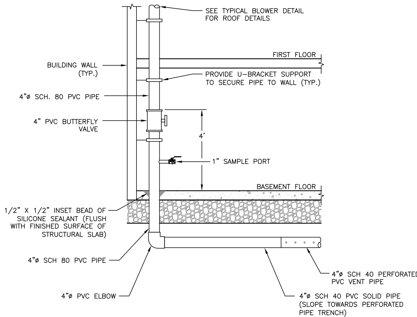
TYPICAL RISER DETAIL SCALE: NOT TO SCALE
