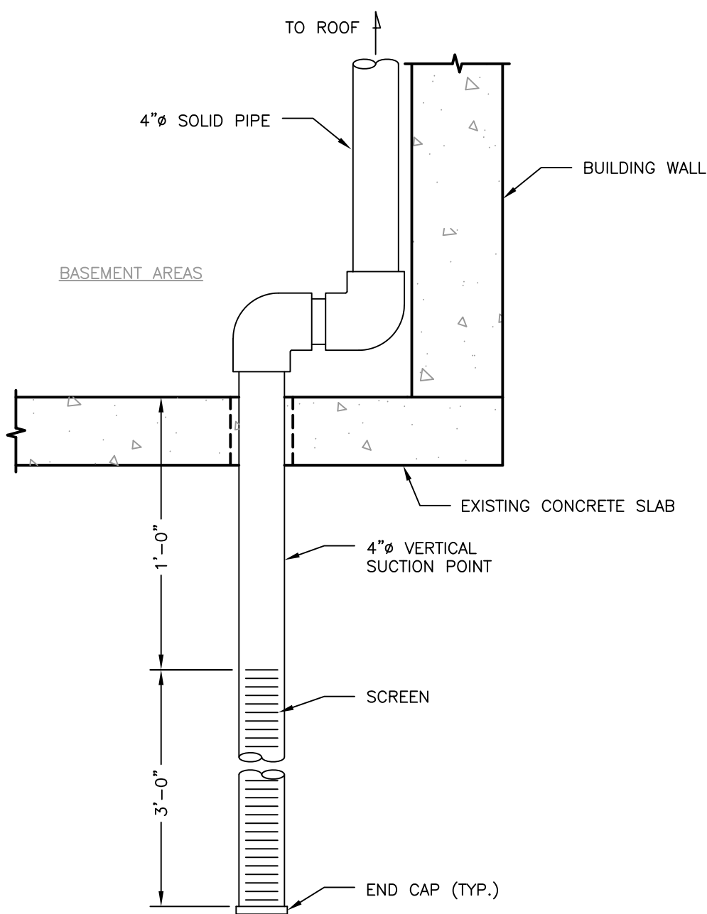
TYPICAL VERTICAL SECTION POINT DETAIL SCALE: NOT TO SCALE
