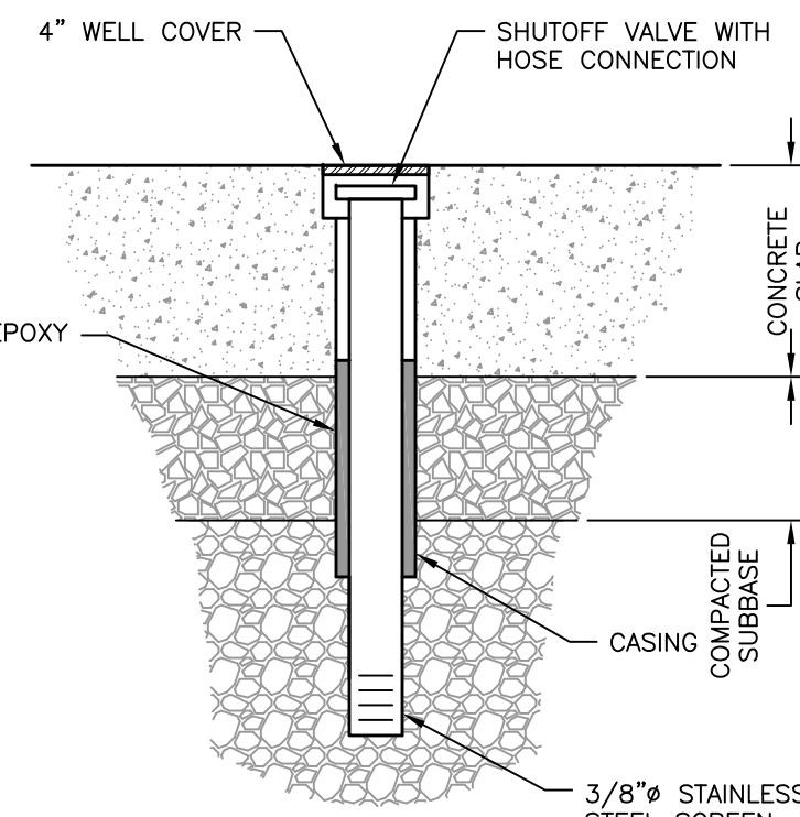
TYPICAL SOIL VAPOR MONITORING POINT DETAIL SCALE: NOT TO SCALE
