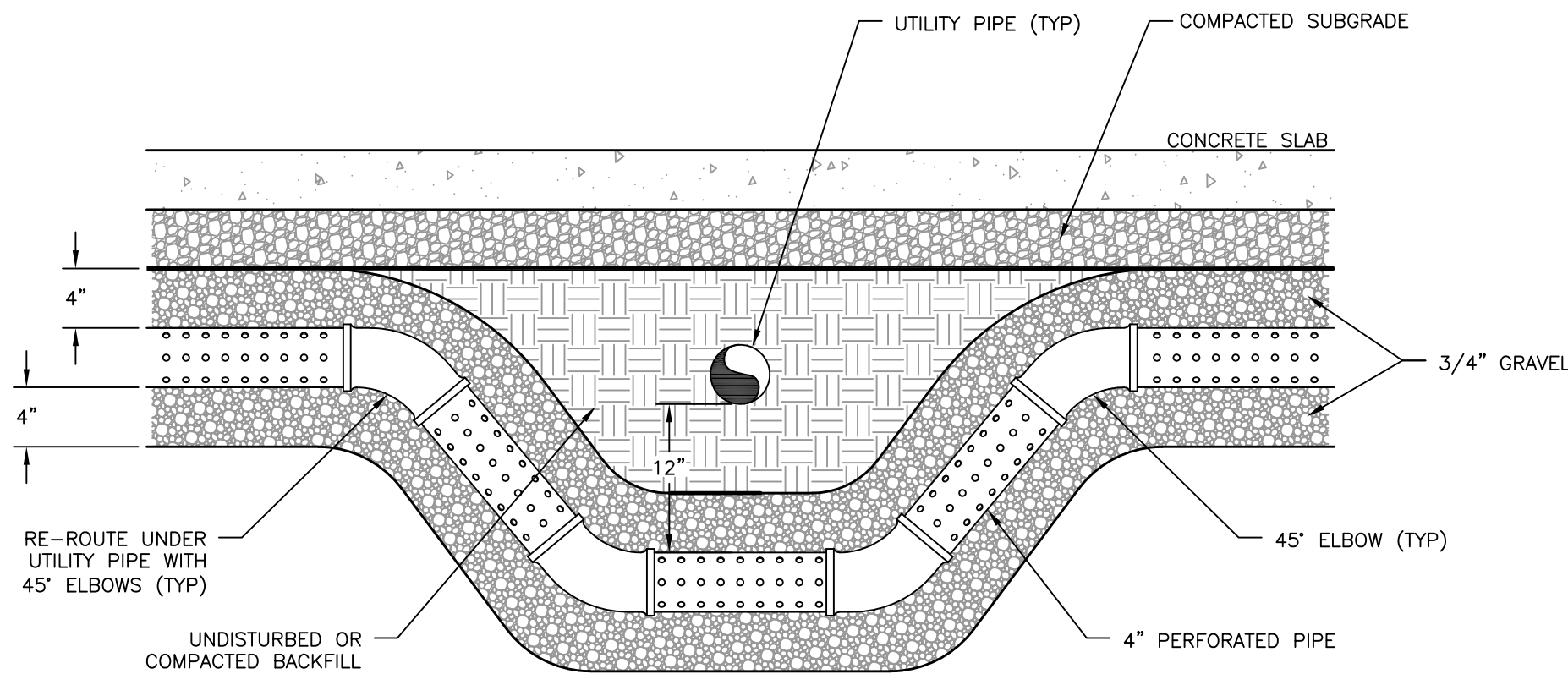
TYPICAL UTILITY PIPE CROSSING SCALE: NOT TO SCALE
