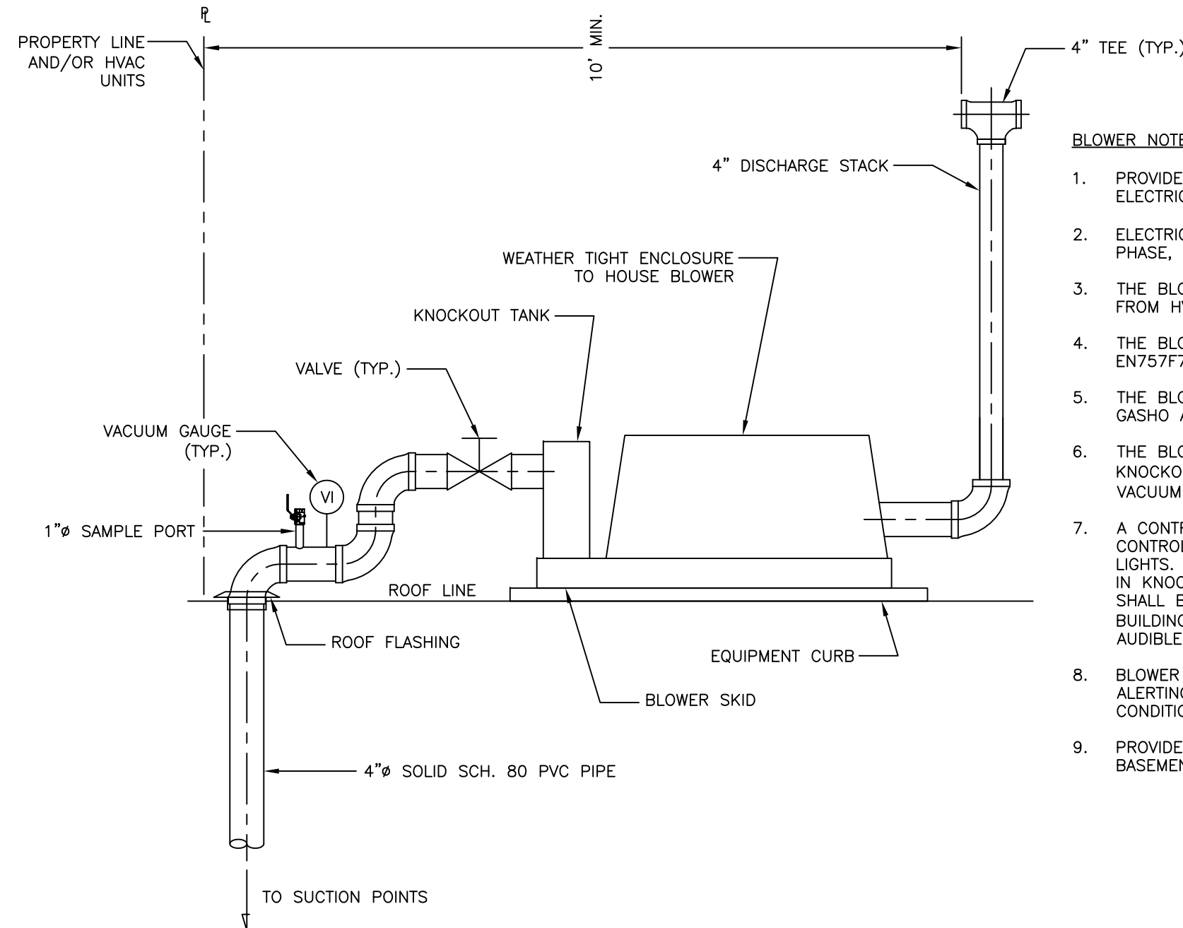
TYPICAL BLOWER DETAIL SCALE: NOT TO SCALE
