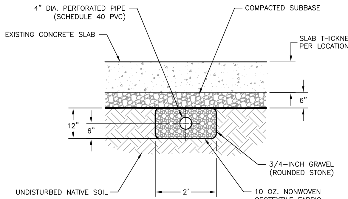
SUB-SLAB DEPRESSURIZATION SYSTEM PIPE DETAIL SCALE: NOT TO SCALE
