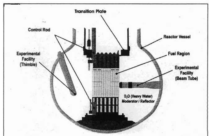
Figure 2. Reactor Components
