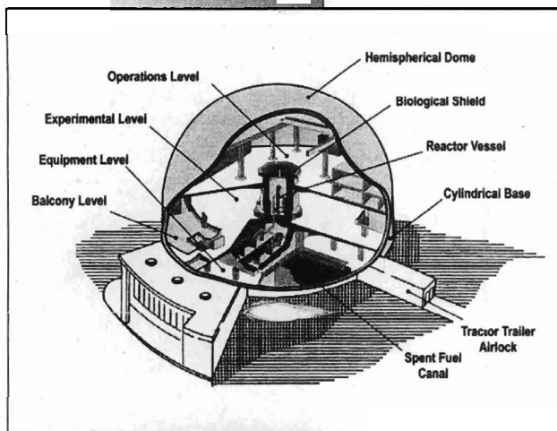
Figure 1. Confinement Building
