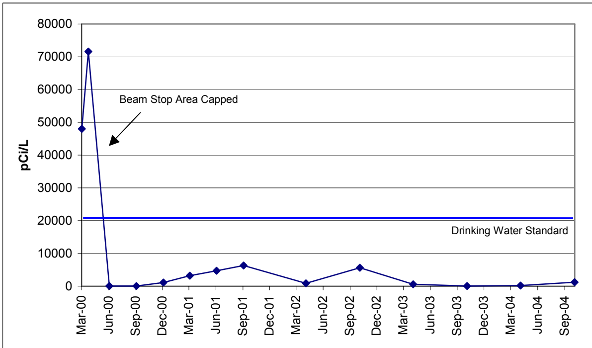
Figure 4-10. Maximum Tritium Concentrations in Temporary & Permanent Wells, Downgradient of U-Line Beam Stop.
