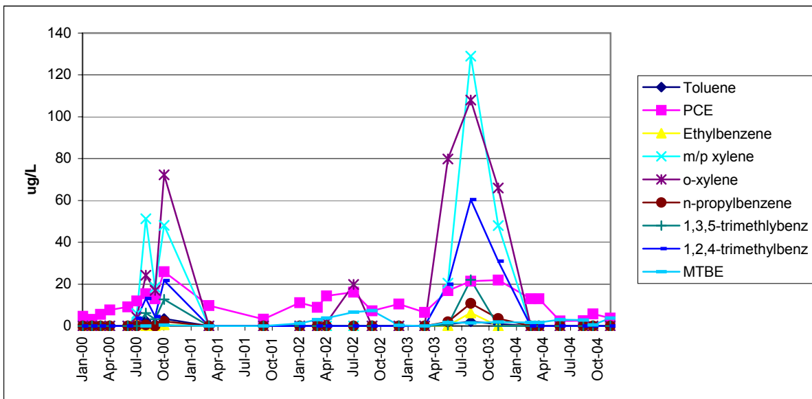
Figure 4-24. Downgradient Well 085-17: Trend of Service Station-Related VOCs. Note that carbon tetrachloride originating from the upgradient carbon tetrachloride UST source area is not included.
