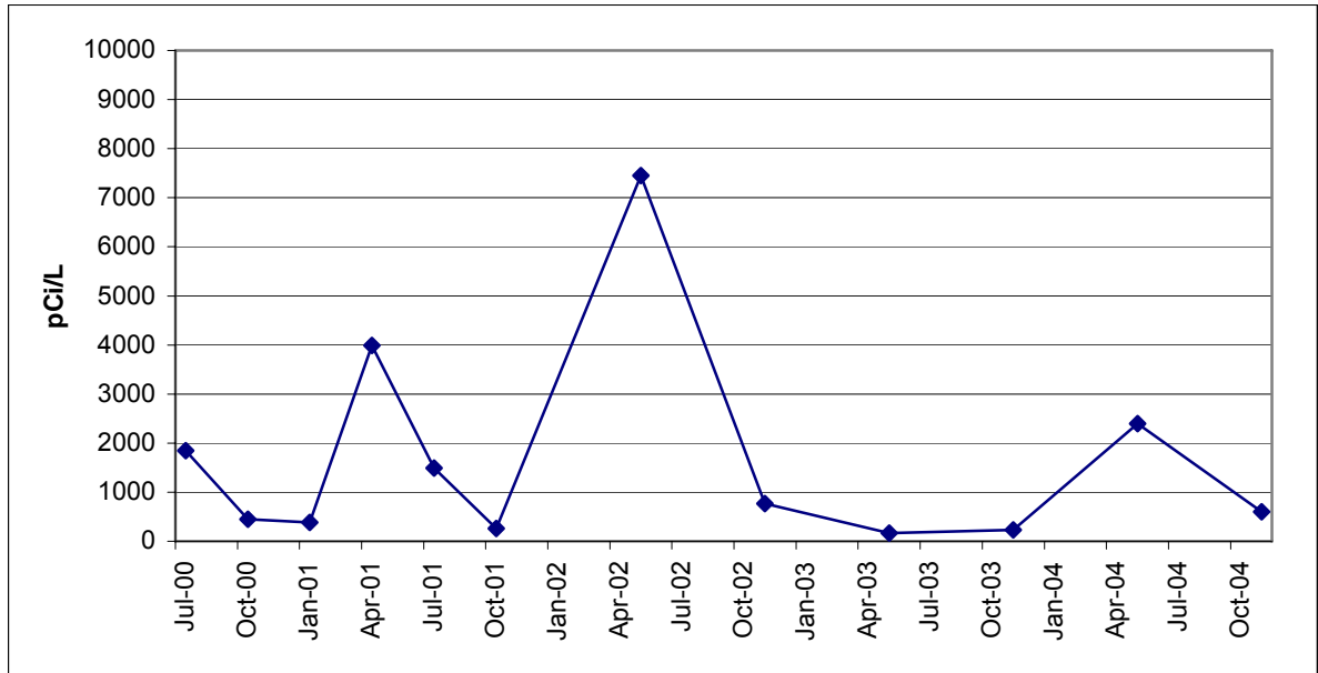
Figure 4-9: Maximum Tritium Concentrations in Well 054-129, Downgradient of the Former U-Line Beam Target.
