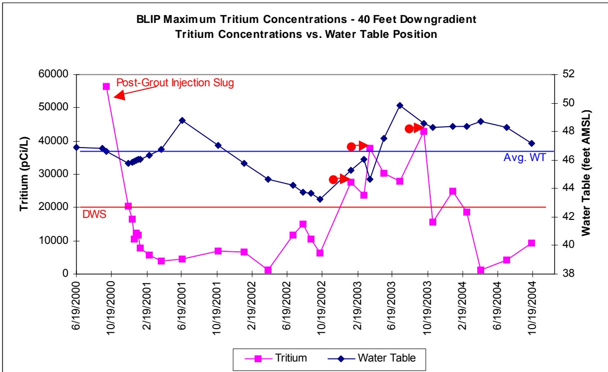
Figure 4-14. Tritium Concentrations vs. Water Table Position, 40 Feet Downgradient of the BLIP Target Vessel.
