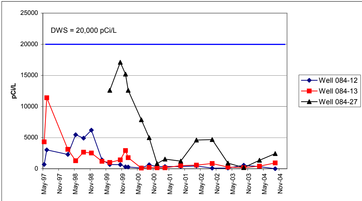
Figure 4-17. Tritium Concentrations Downgradient of the BMRR from 1997–2004.
