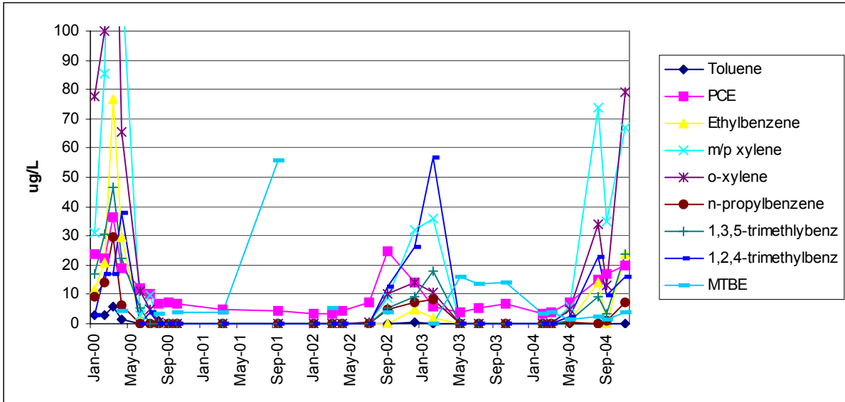
Figure 4-25. Downgradient Well 085-236: Trend of Service Station-Related VOCs. Note that carbon tetrachloride from the upgradient carbon tetrachloride UST source area is not included.
