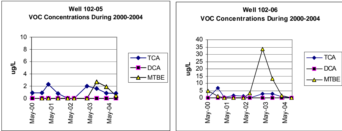
Figure 4-20. VOC Concentration Trends Downgradient of the Gasoline UST Area.
