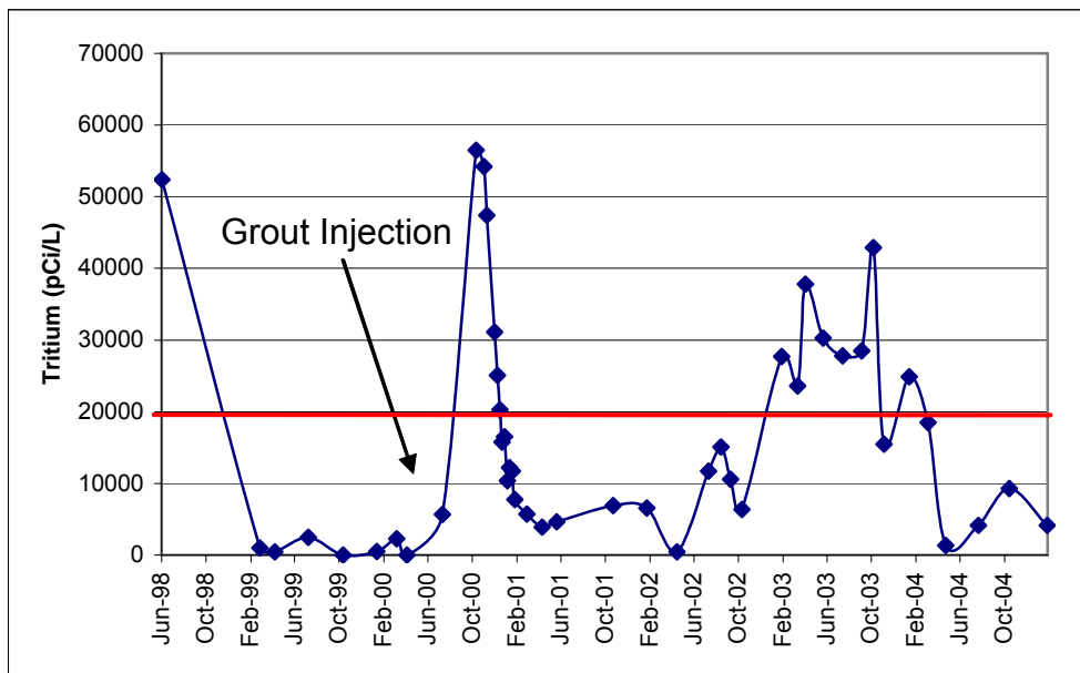
Figure 4-12. Maximum Tritium Concentrations in Wells ~ 40 feet Downgradient of BLIP Target Vessel.
