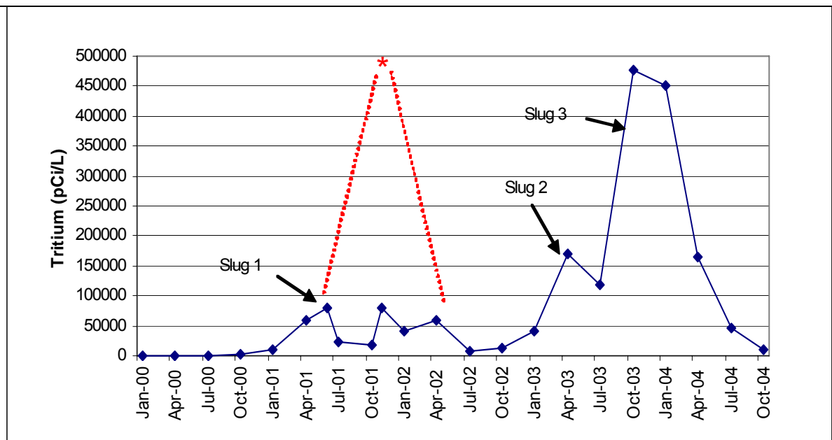
Figure 4-7. g-2 Tritium Plume Concentrations Downgradient of Building 912.
