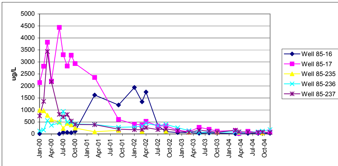
Figure 4-23. Carbon Tetrachloride Concentration Trends in Service Station Monitoring Wells.
