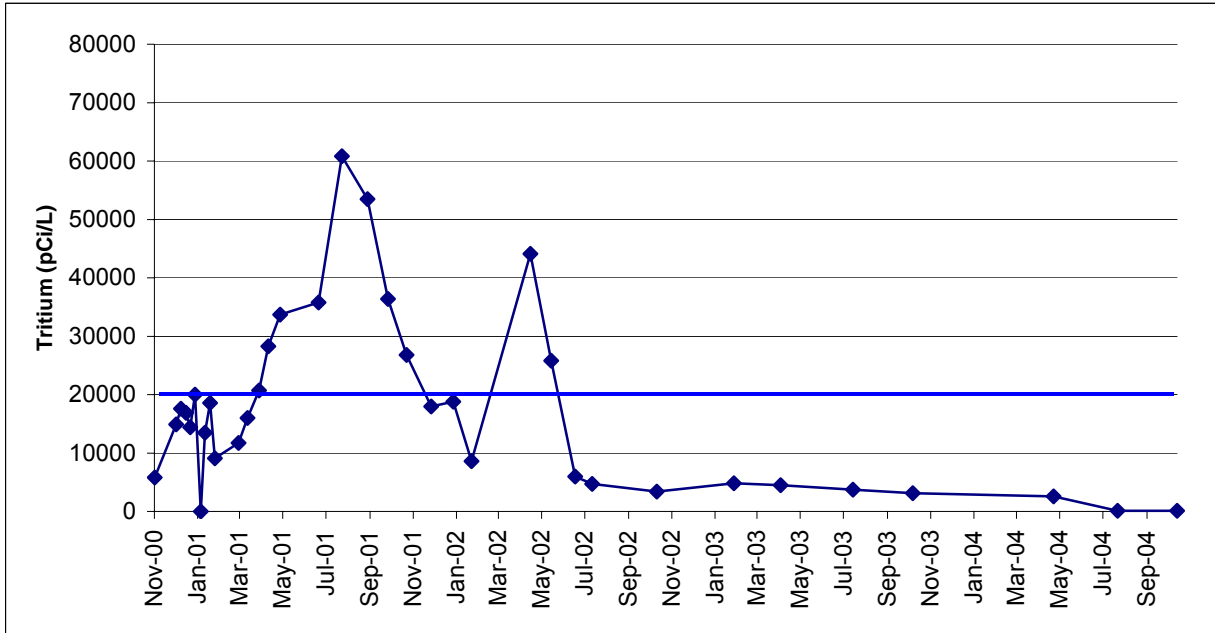
Figure 4-13. Maximum Tritium Concentrations Approximately 150 feet Downgradient of the BLIP Target Vessel.
