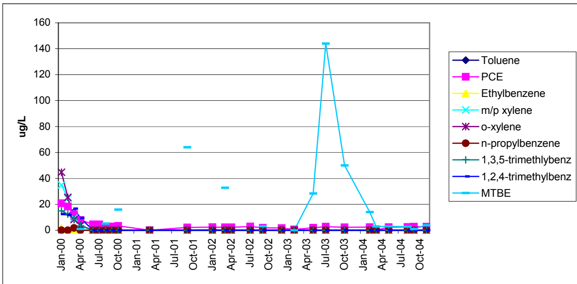
Figure 4-26. Downgradient Well 085-237: Trend of Service Station-Related VOCs. Note that carbon tetrachloride originating from the upgradient carbon tetrachloride UST source area is not included.
