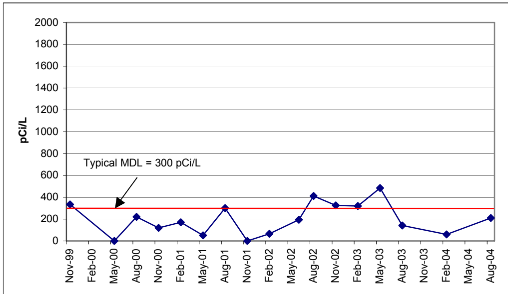
Figure 4-31. Tritium Concentration Trends in Well 066-07, Upgradient of Waste Management Facility.
