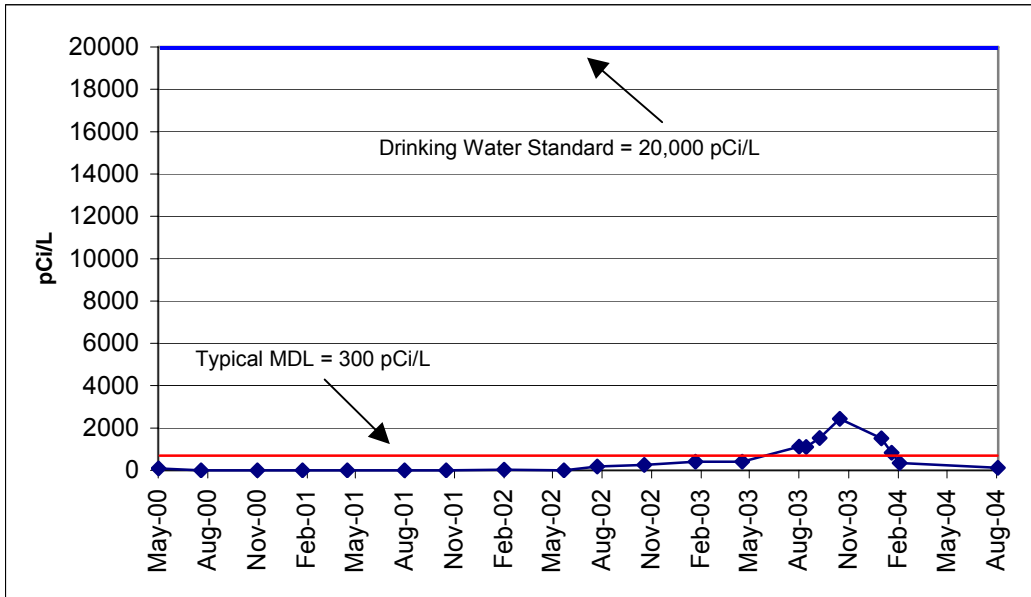
Figure 4-30. Tritium Concentration Trends in Well 056-23 Downgradient of Waste Management Facility.
