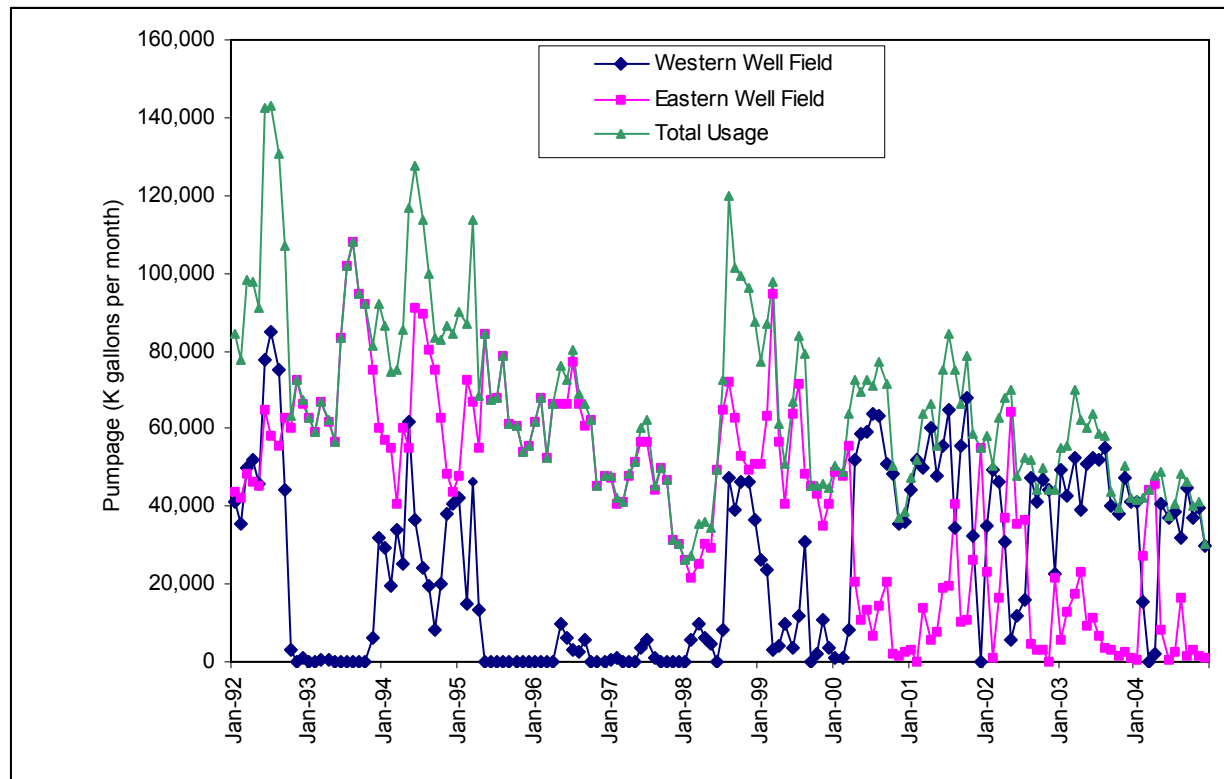
Figure 2-4. Summary of BNL Supply Well Pumpage 1992 through 2004.
