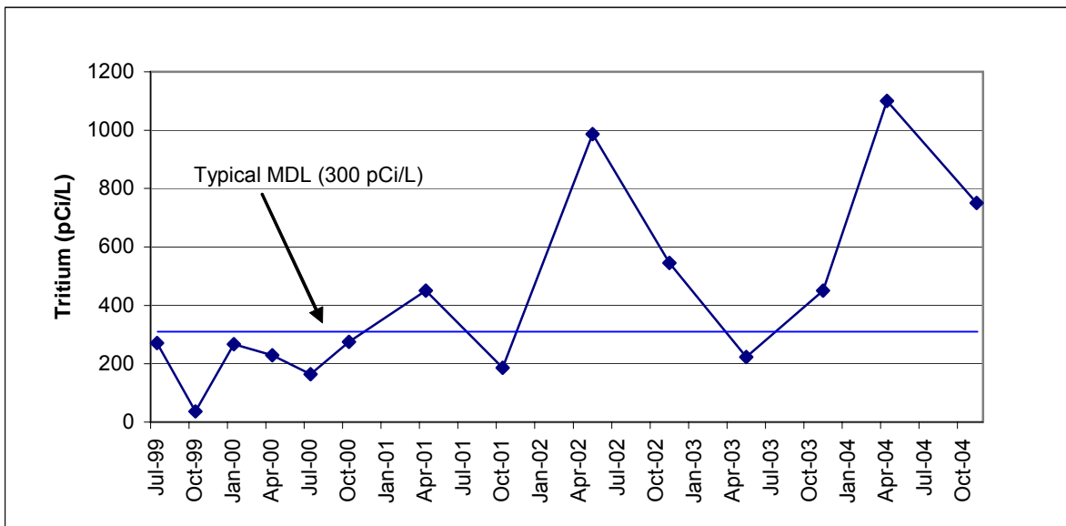
Figure 4-8. Maximum Tritium Concentrations in Wells 054-63 and 054-64, Downgradient of the J-10 Beam Stop.
