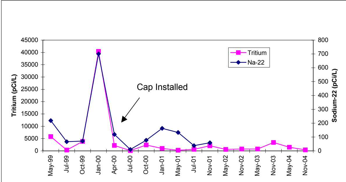
Figure 4-4. Maximum Tritium and Sodium-22 Concentrations in Temporary and Permanent Monitoring Wells Downgradient of the Former E-20 Catcher.
