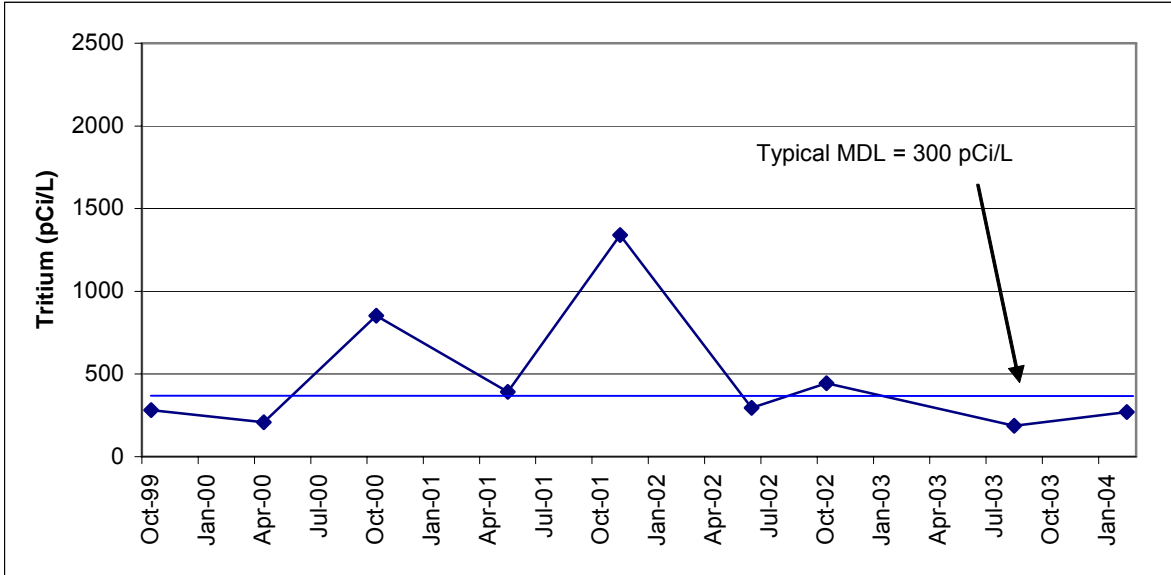
Figure 4-3. Maximum Tritium Concentrations Downgradient of AGS Booster Beam Stop (Wells 064-51 and 064-52).
