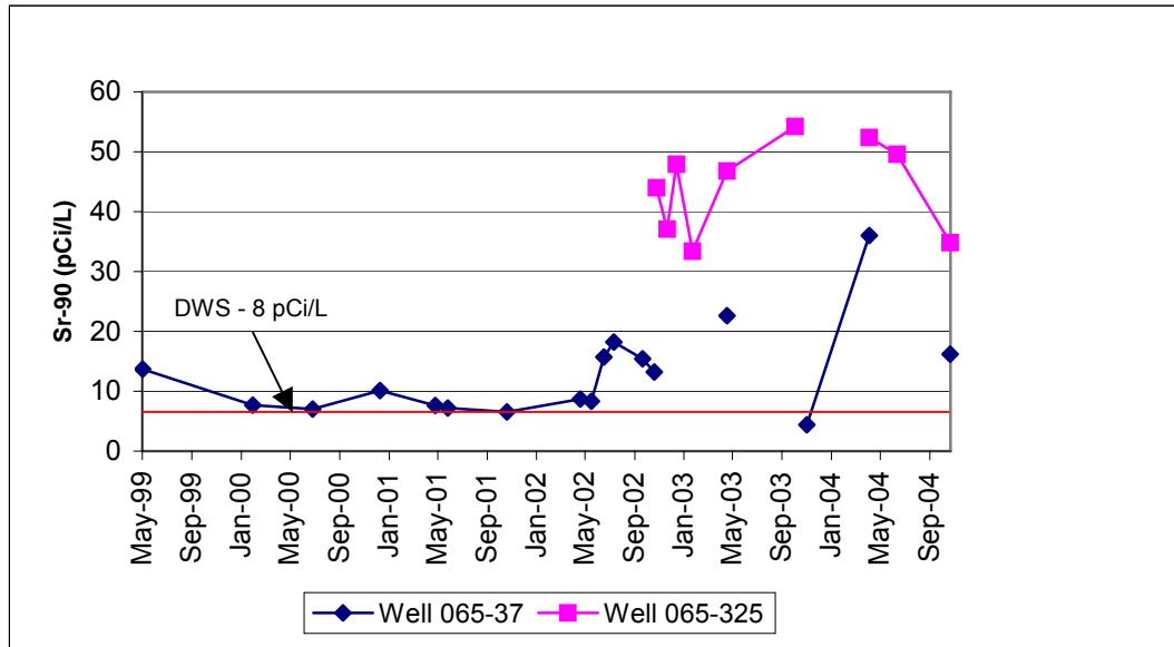
Figure 4-33. Sr-90 Concentration Trends in Downgradient Wells 065-37 and 065-325 at Building 801.
