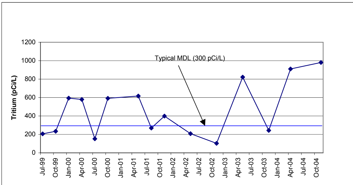
Figure 4-5. Maximum Tritium Concentrations Downgradient of 914 Transfer Tunnel (Wells 064-03, -53, and -54).
