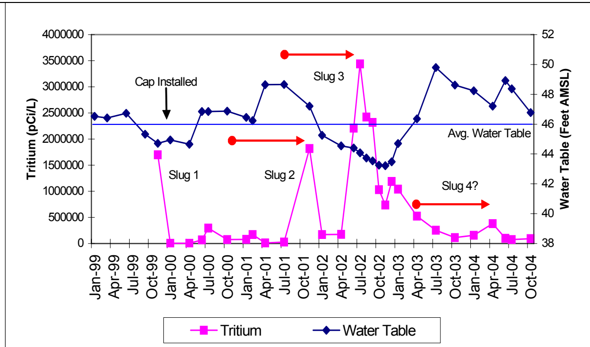
Figure 4-6. Maximum Tritium Concentrations in Permanent and Temporary Wells Downgradient of the g-2/VQ-12 Source Area (West Side of Building 912A).
