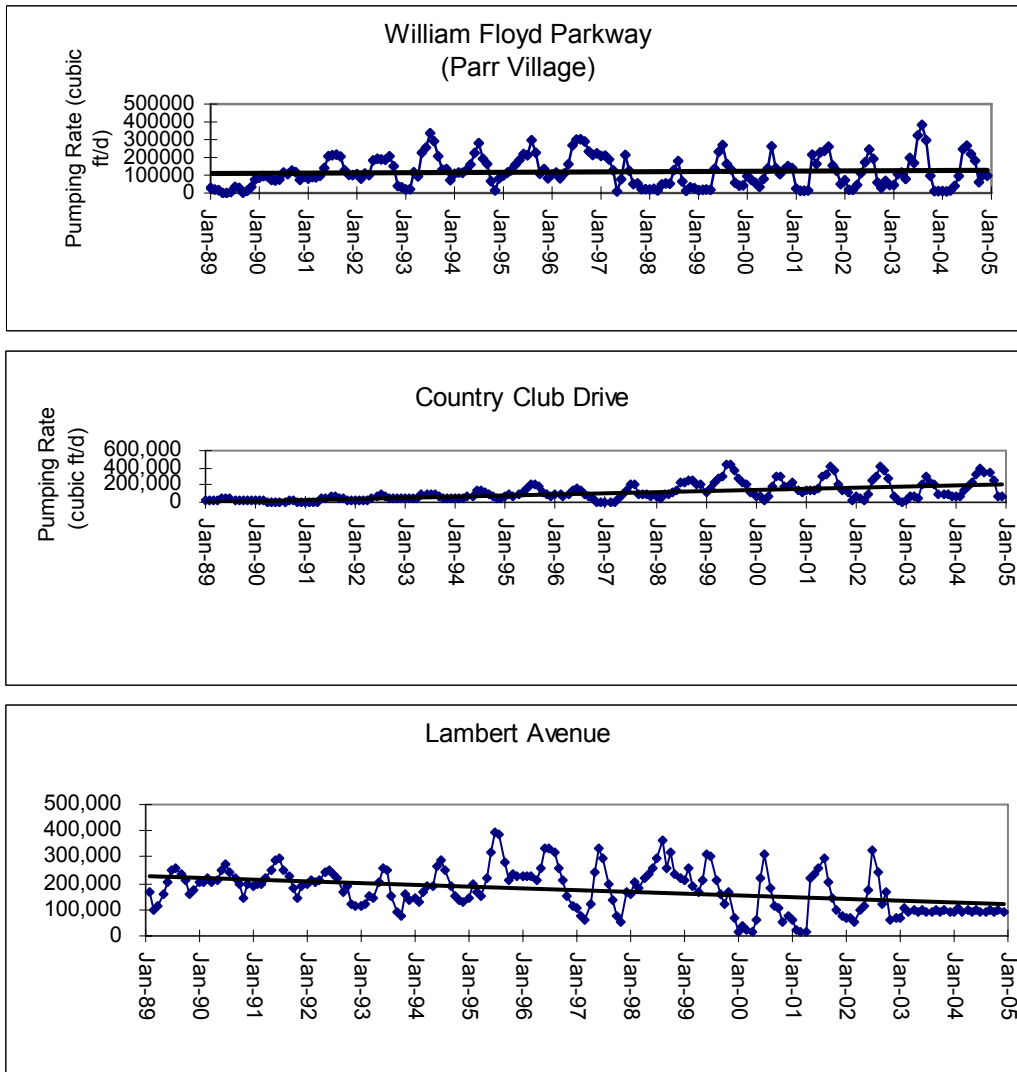
Figure 2-6. Suffolk County Water Authority Pumping Near BNL.
