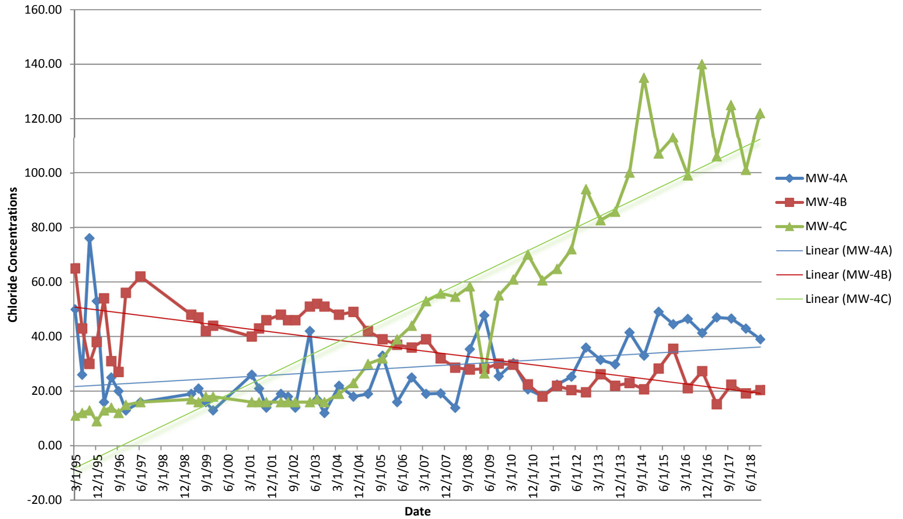
Figure 5 Monitoring Well Cluster 4 Chloride Trends (1995 - 2018)
