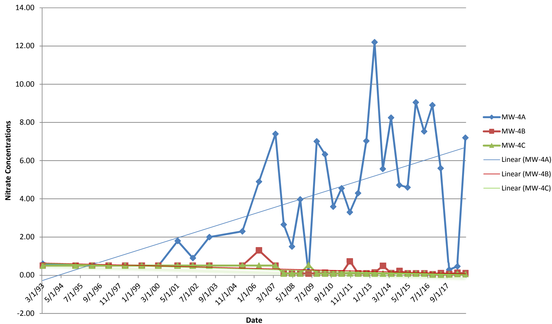
Figure 10 Monitoring Well Cluster 4 Nitrate Trends (1993 - 2018)
