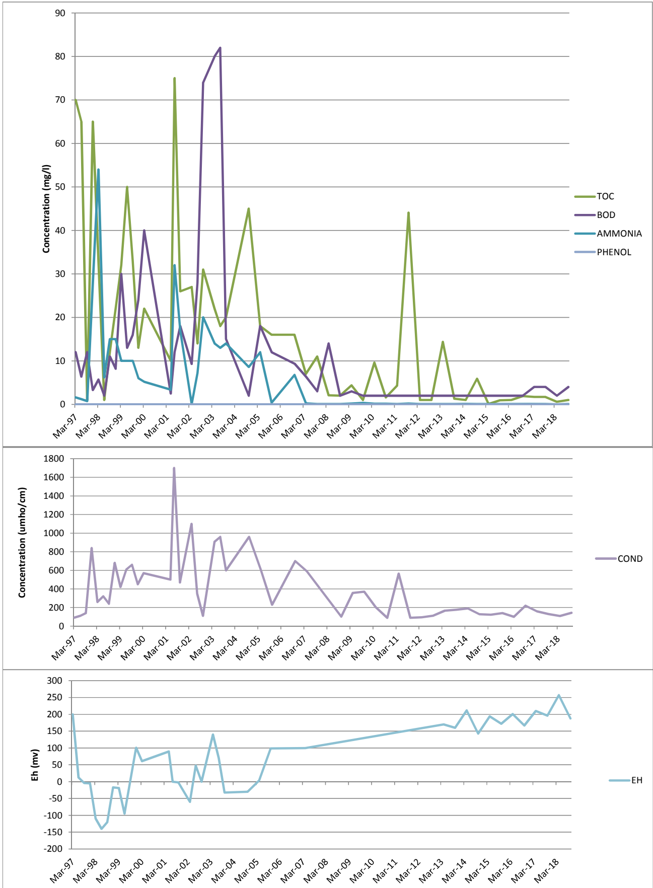
Figure 3 Monitoring Well 11B (1997 - 2018)
