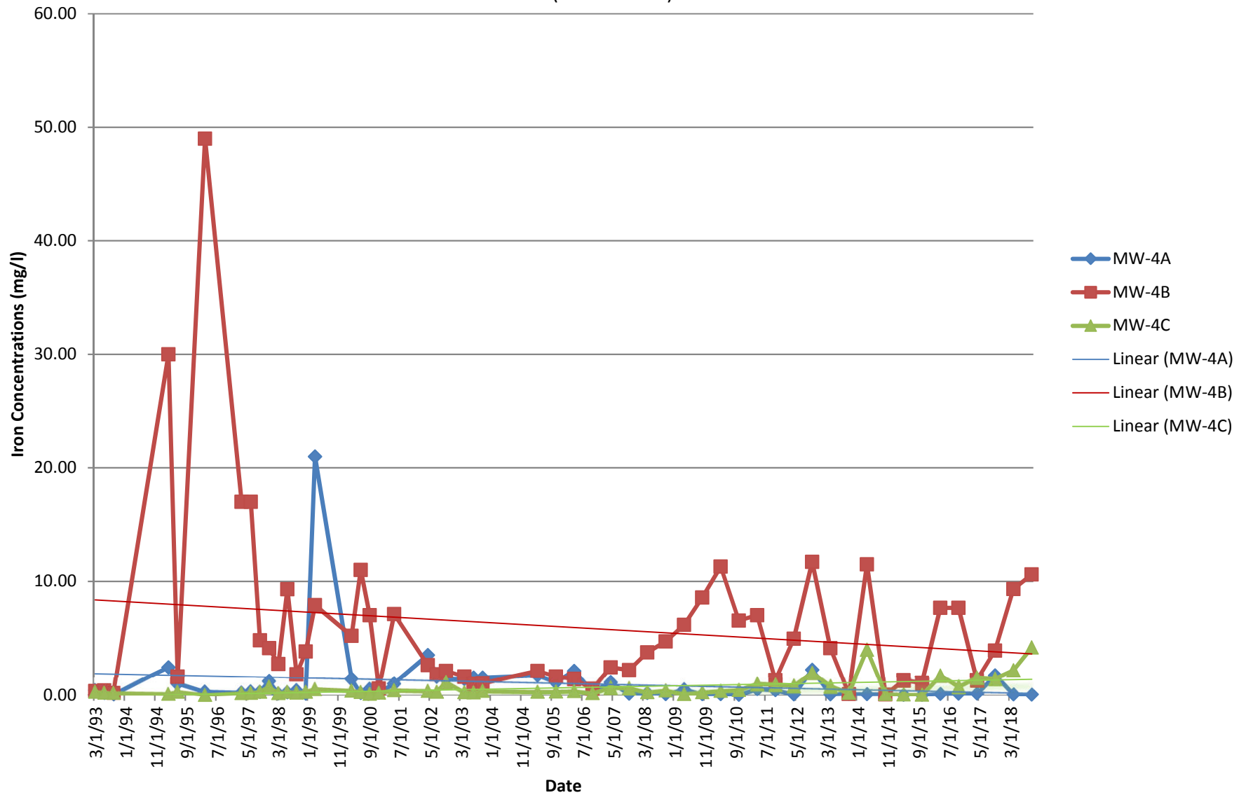
Figure 8 Monitoring Well Cluster 4 Iron Trends (1993 - 2018)
