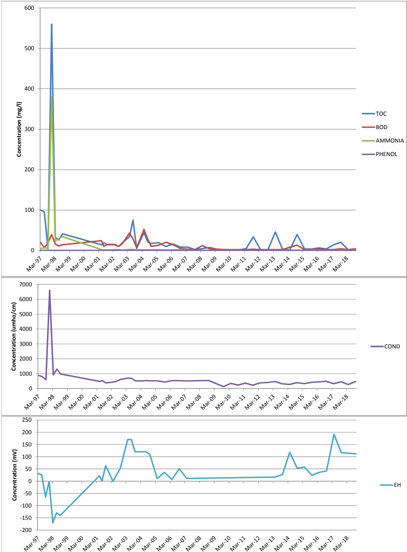
Figure 2 Monitoring Well 11A (1997 - 2018)
