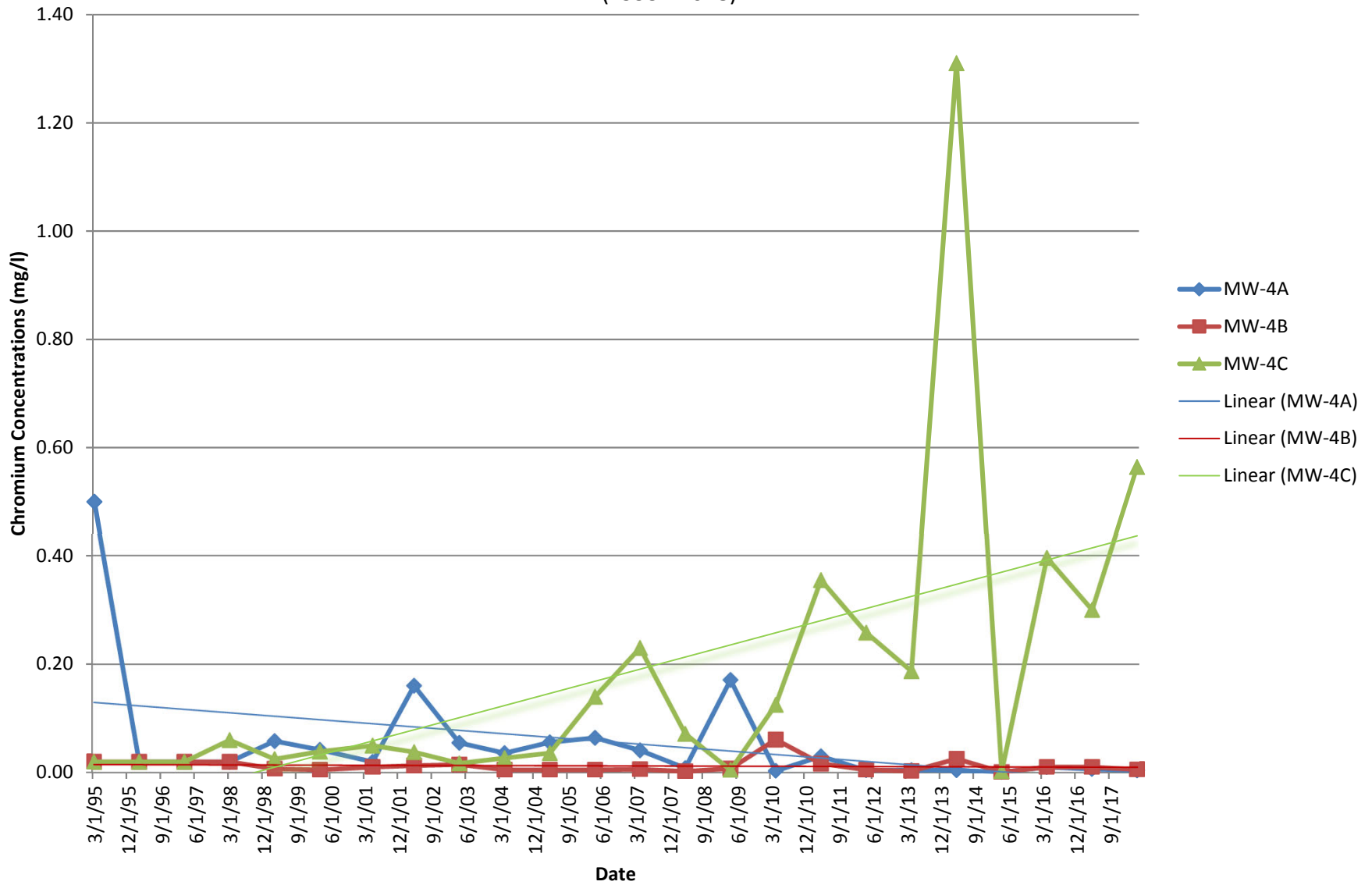
Figure 6 Monitoring Well Cluster 4 Chromium Trends (1995 - 2018)
