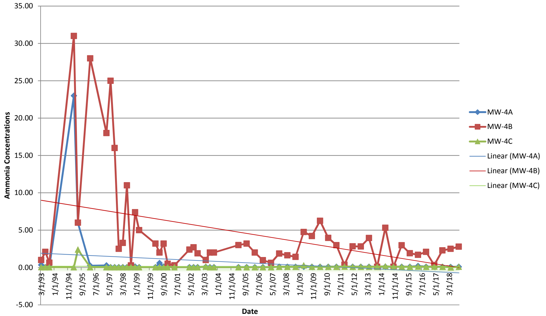
Figure 4 Monitoring Well Cluster 4 Ammonia Trends (1993 - 2018)
