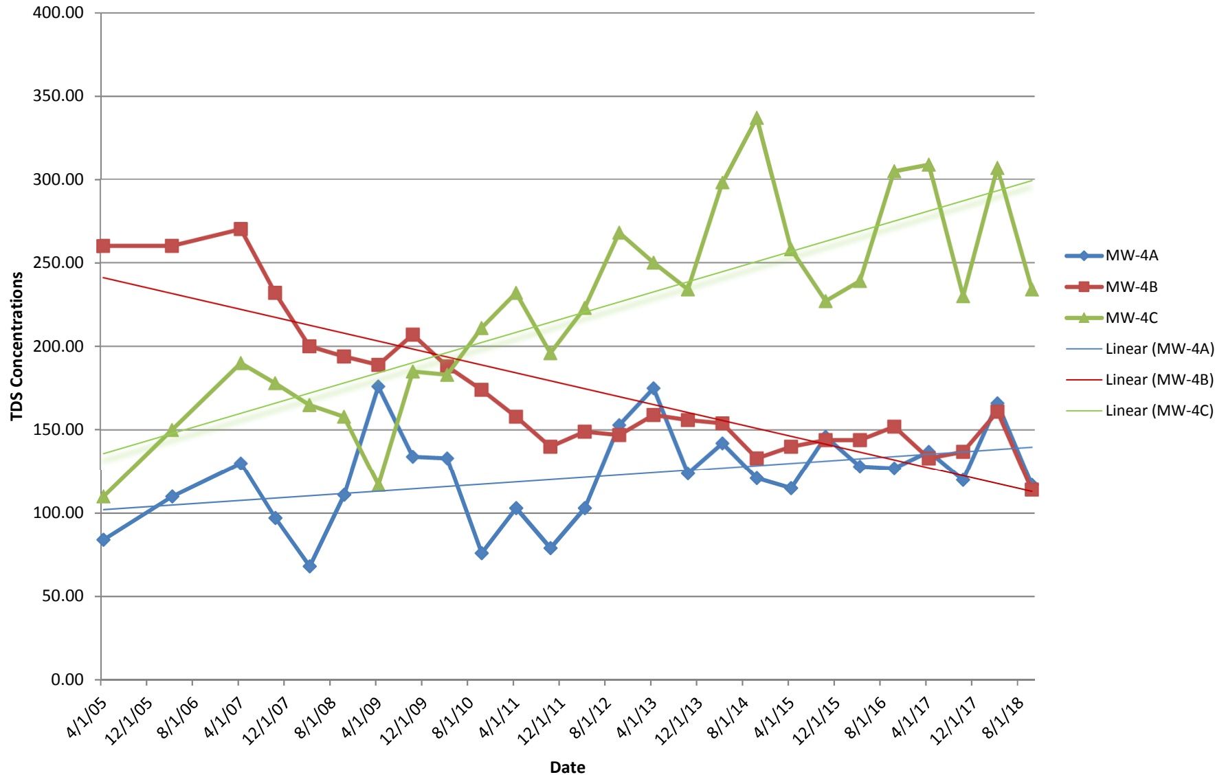
Figure 11 Monitoring Well Cluster 4 Total Dissolved Solids Trends (2005 - 2018)
