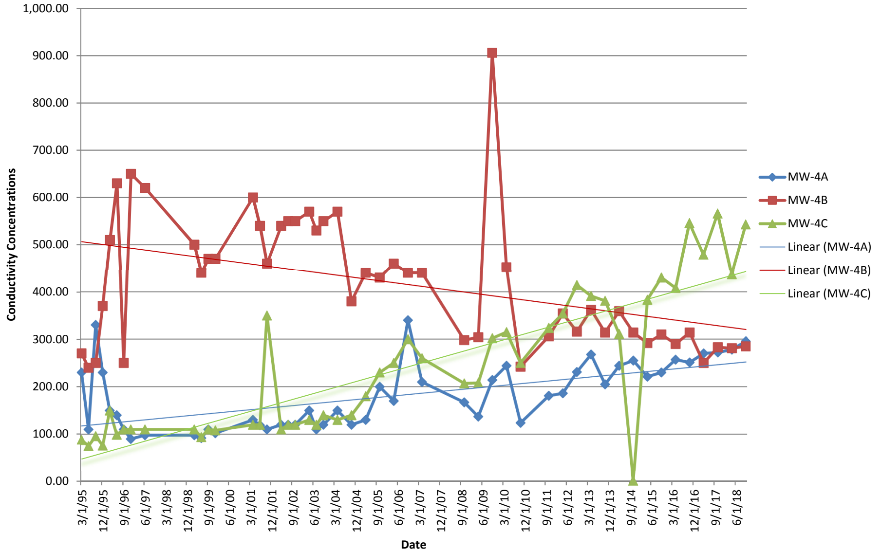
Figure 7 Monitoring Well Cluster 4 Conductivity Trends (1995 - 2018)
