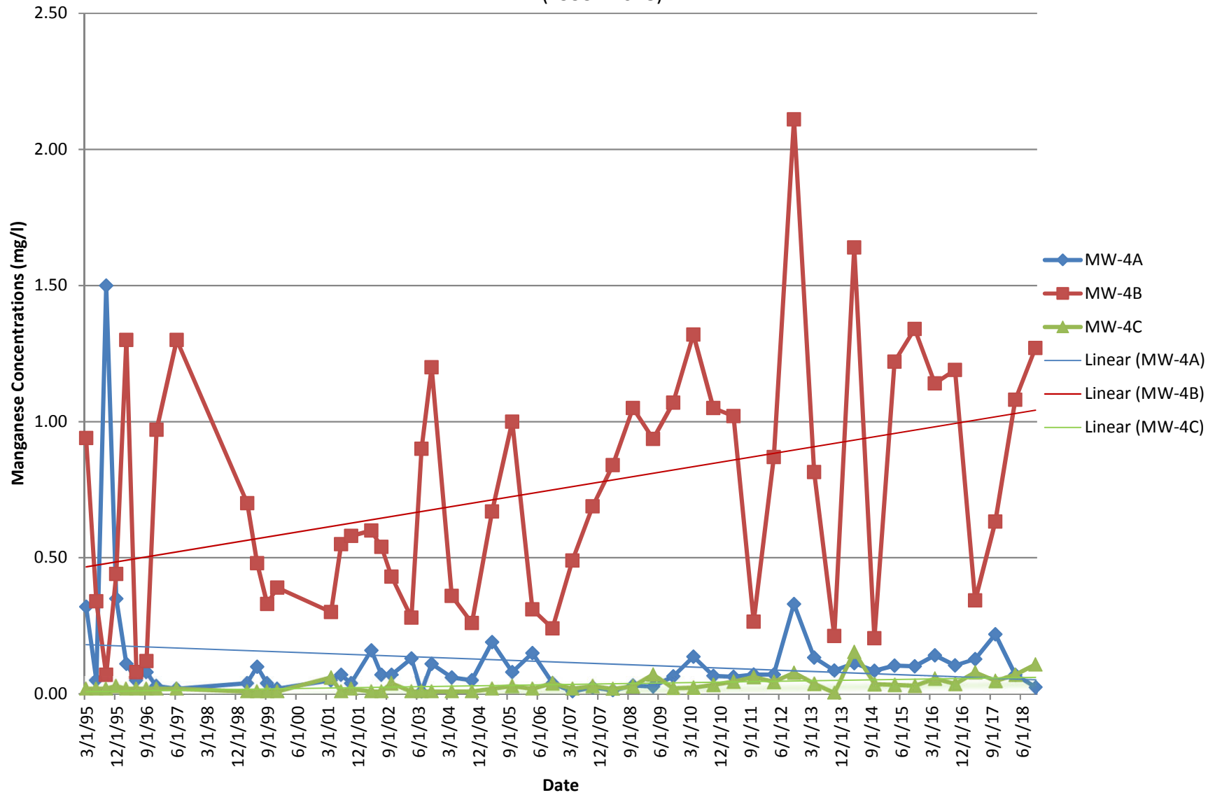
Figure 9 Monitoring Well Cluster 4 Manganese Trends (1995 - 2018)
