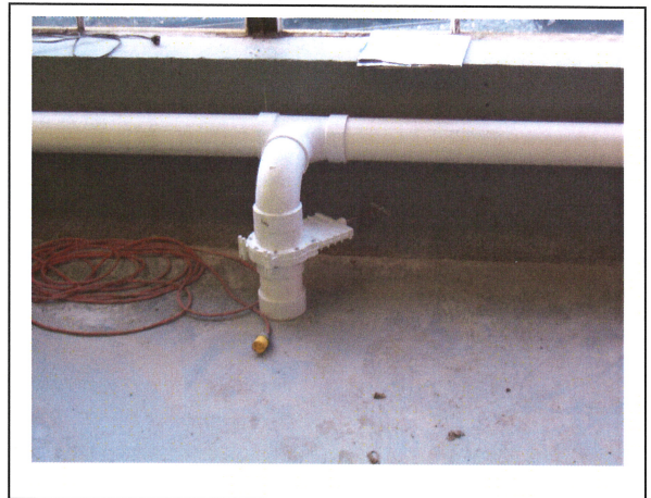
Photo #2: Extraction point and damper valve located at northwest wall.
