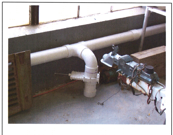
Photo #4: Extraction point and damper valve located at southeast wall.
