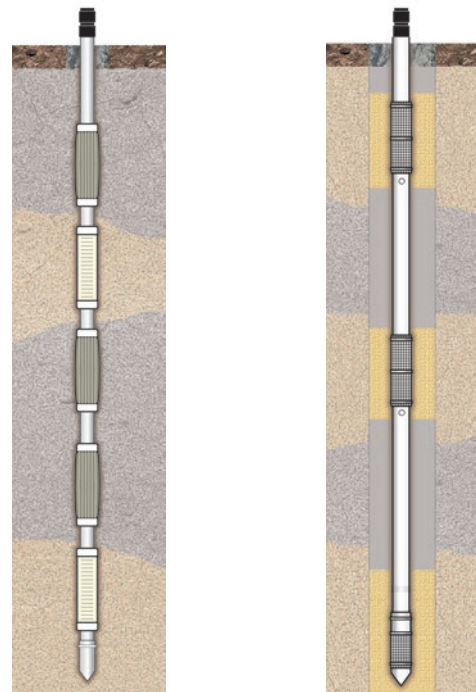
Typical 3-Channel CMT Installation in Overburden with Bentonite and Sand Cartridges
