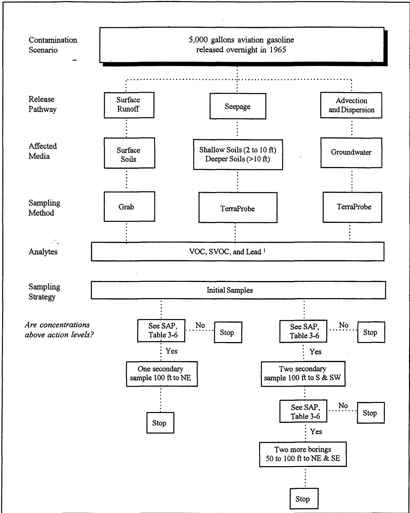
FIGURE 8-4 SAMPLING LOGIC DIAGRAM SITE 1 - AVIATION GASOLINE SPILL SITE 106 RESCUE GROUP, NYANG WESTHAMPTON BEACH, NEW YORK
