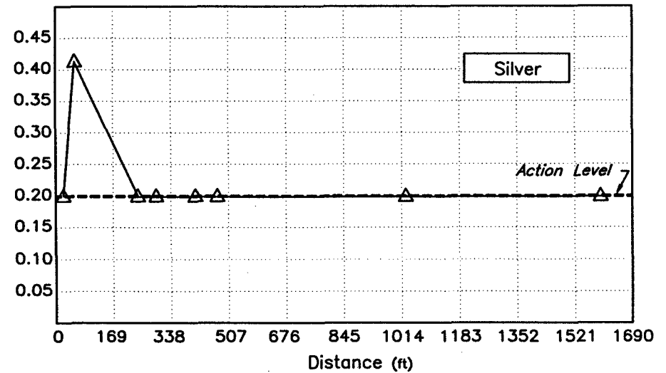
FIGURE 8-24. CONT. SEDIMENT CONCENTRATIONS VS. DISTANCE SITE 5 - SOUTHWEST STORM DRAINAGE DITCH 106TH RESCUE GROUP, NYANG WESTHAMPTON BEACH, NEW YORK
