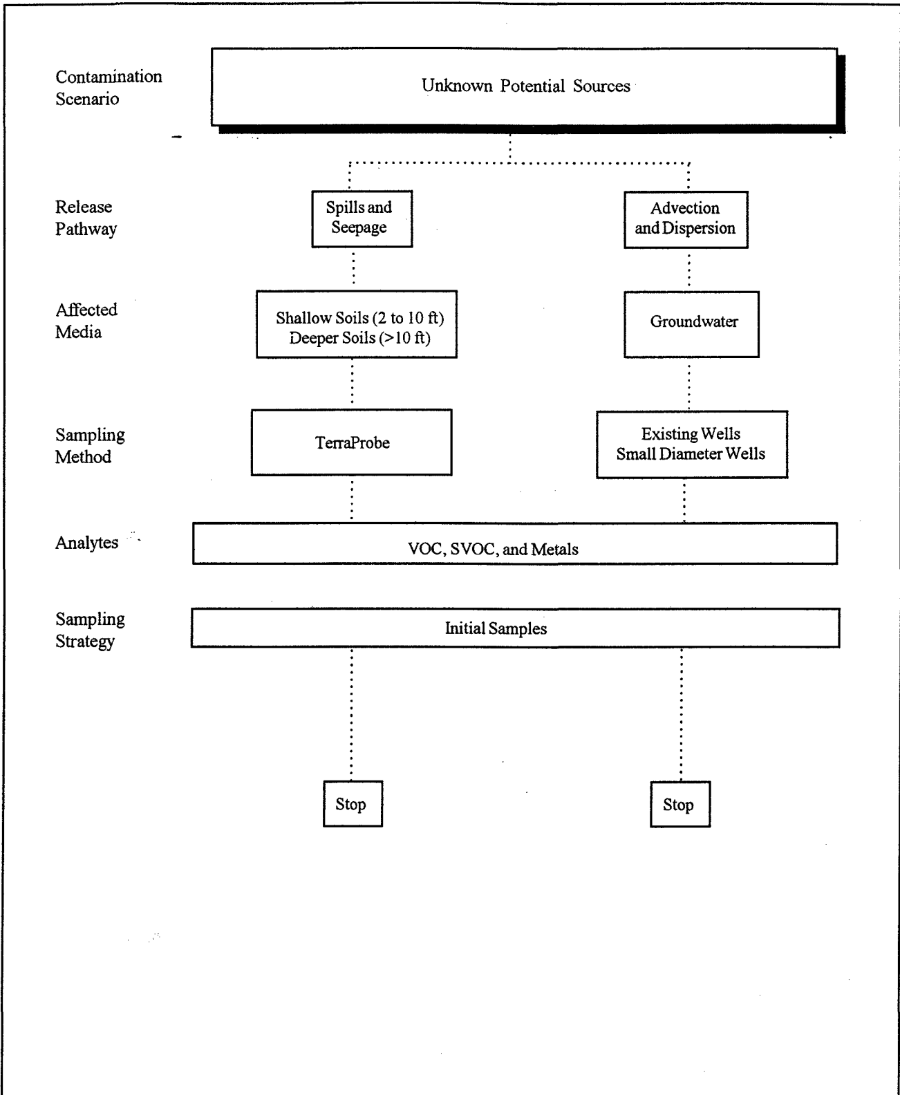
FIGURE 8-3 SAMPLING LOGIC DIAGRAM BACKGROUND 106 RESCUE GROUP, NYANG WESTHAMPTON BEACH, NEW YORK
