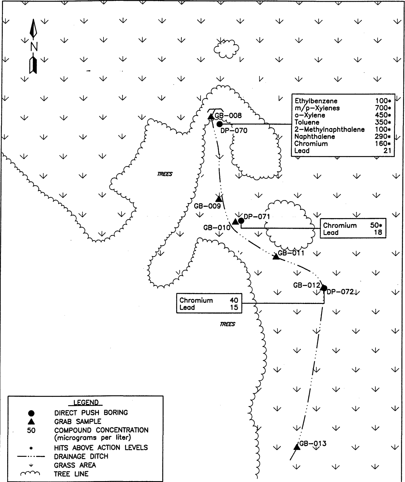
FIGURE 8-41 DETECTED CONCENTRATIONS IN GROUNDWATER SITE 9 - RAMP DRAINAGE OUTFALL 106TH RESCUE GROUP, NYANG WESTHAMPTON BEACH, NEW YORK
