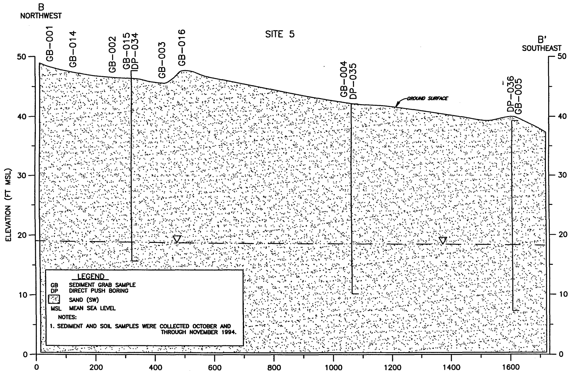
FIGURE 8-22 CROSS SECTION B-B' 106TH RESCUE GROUP, NYANG WESTHAMPTON BEACH, NEWYORK
