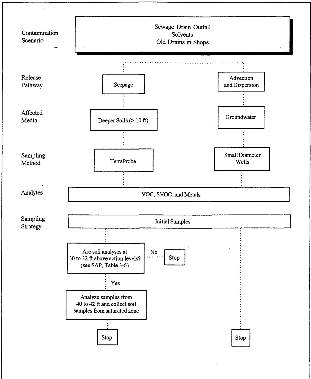
FIGURE 8-25 SAMPLING LOGIC DIAGRAM SITE 8 - OLD BASE SEPTIC SYSTEMS 106 RESCUE GROUP, NYANG WESTHAMPTON BEACH, NEW YORK
