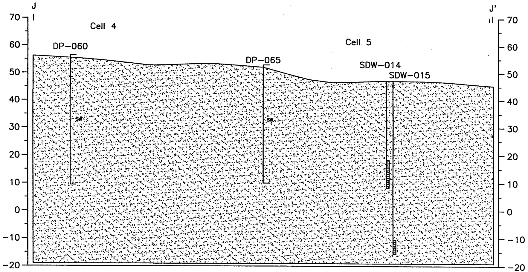
FIGURE 8-34 Cross Section J-J' Site 8, Cells 4 & 5 106th rescue Group, NYANG Westhampton Beach, New York
