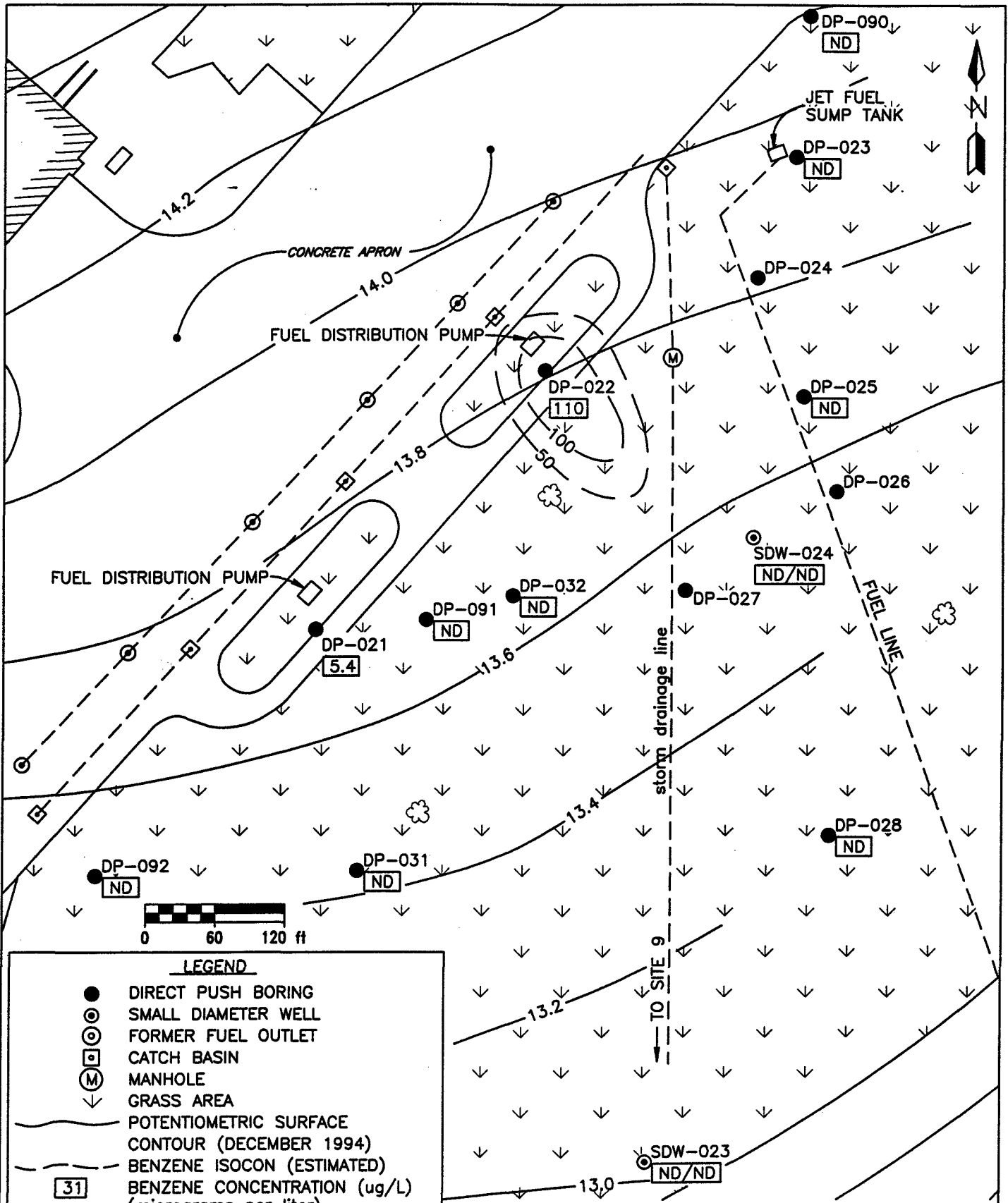
FIGURE 8-17 BENZENE ISOCONCENTRATION CONTOURS IN SHALLOW GROUNDWATER SITE 4 - AIRCRAFT REFUELING APRON SPILL SITE 106TH RESCUE GROUP, NYANG WESTHAMPTON BEACH, NEW YORK
