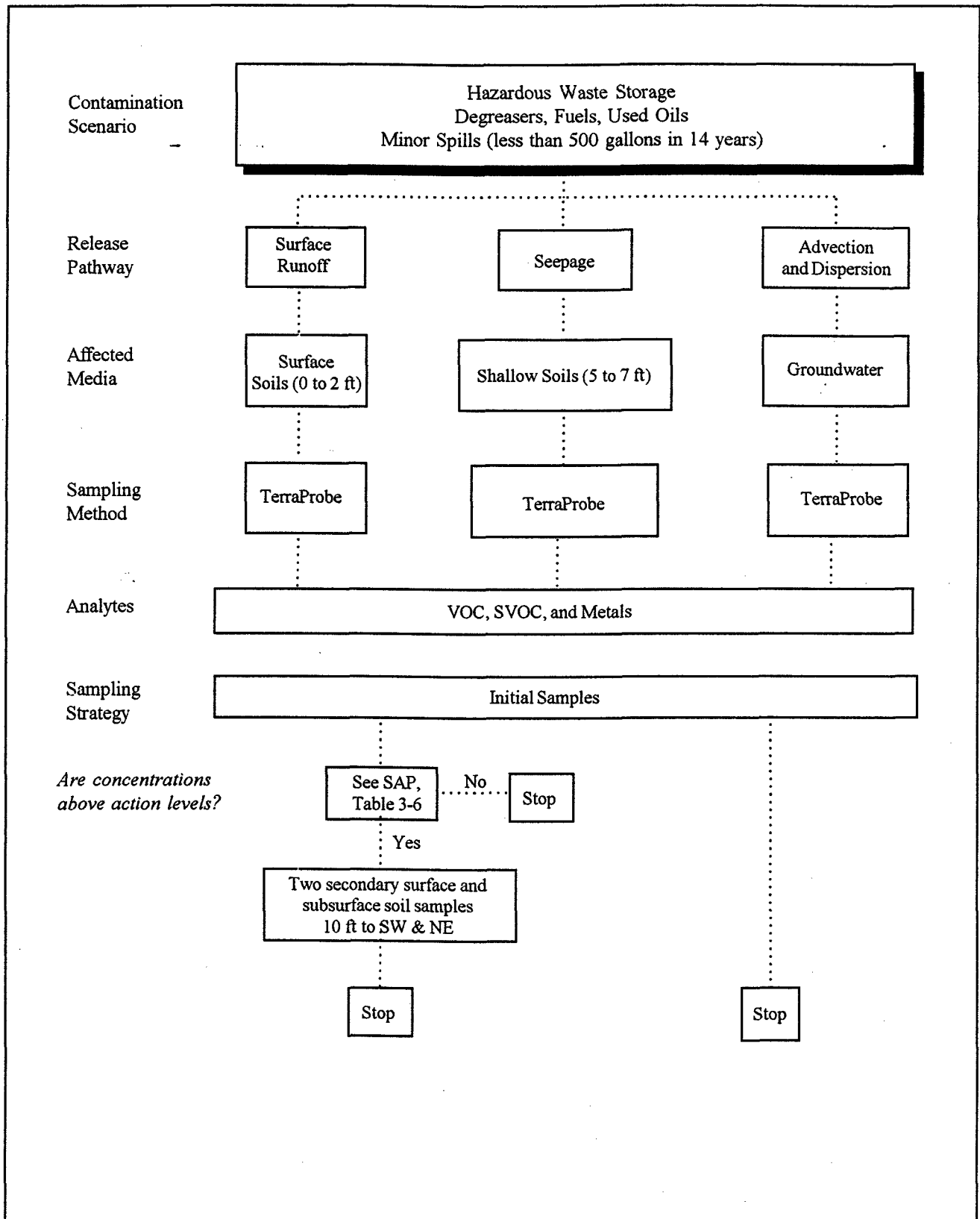
FIGURE 8-8 SAMPLING LOGIC DIAGRAM SITE 2 - FORMER HAZARDOUS WASTE STORAGE AREA 106 RESCUE GROUP, NYANG WESTHAMPTON BEACH, NEW YORK
