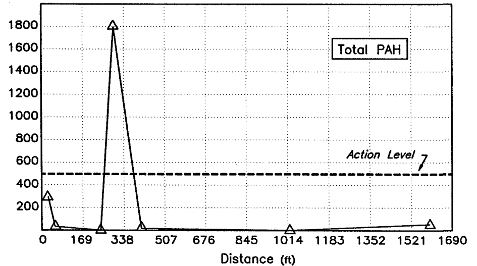
FIGURE 8-24 SEDIMENT CONCENTRATIONS VS. DISTANCE SITE 5 - SOUTHWEST STORM DRAINAGE DITCH 106TH RESCUE GROUP, NYANG WESTHAMPTON BEACH, NEW YORK
