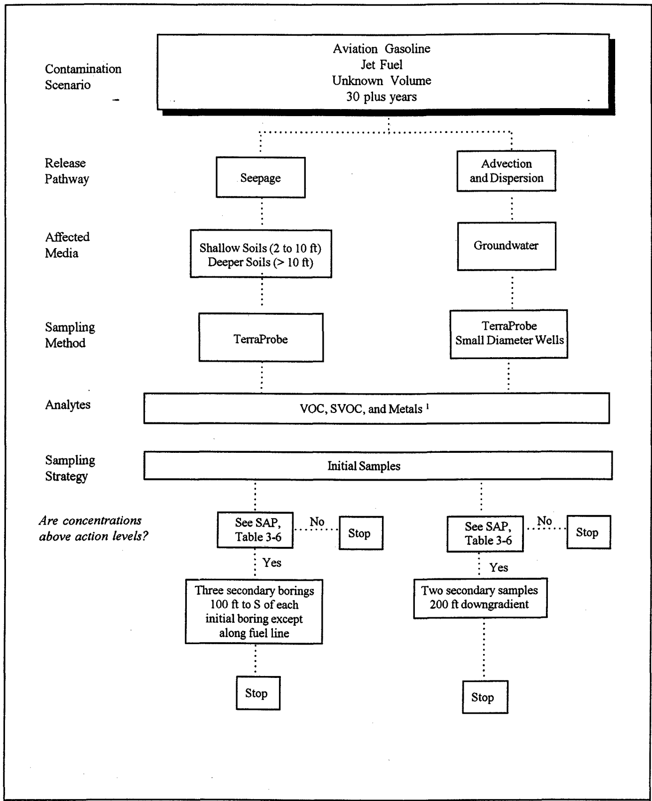
FIGURE 8-12 SAMPLING LOGIC DIAGRAM SITE 4 - AIRCRAFT REFUELING APRON SPILL SITE 106 RESCUE GROUP, NYANG WESTHAMPTON BEACH, NEW YORK
