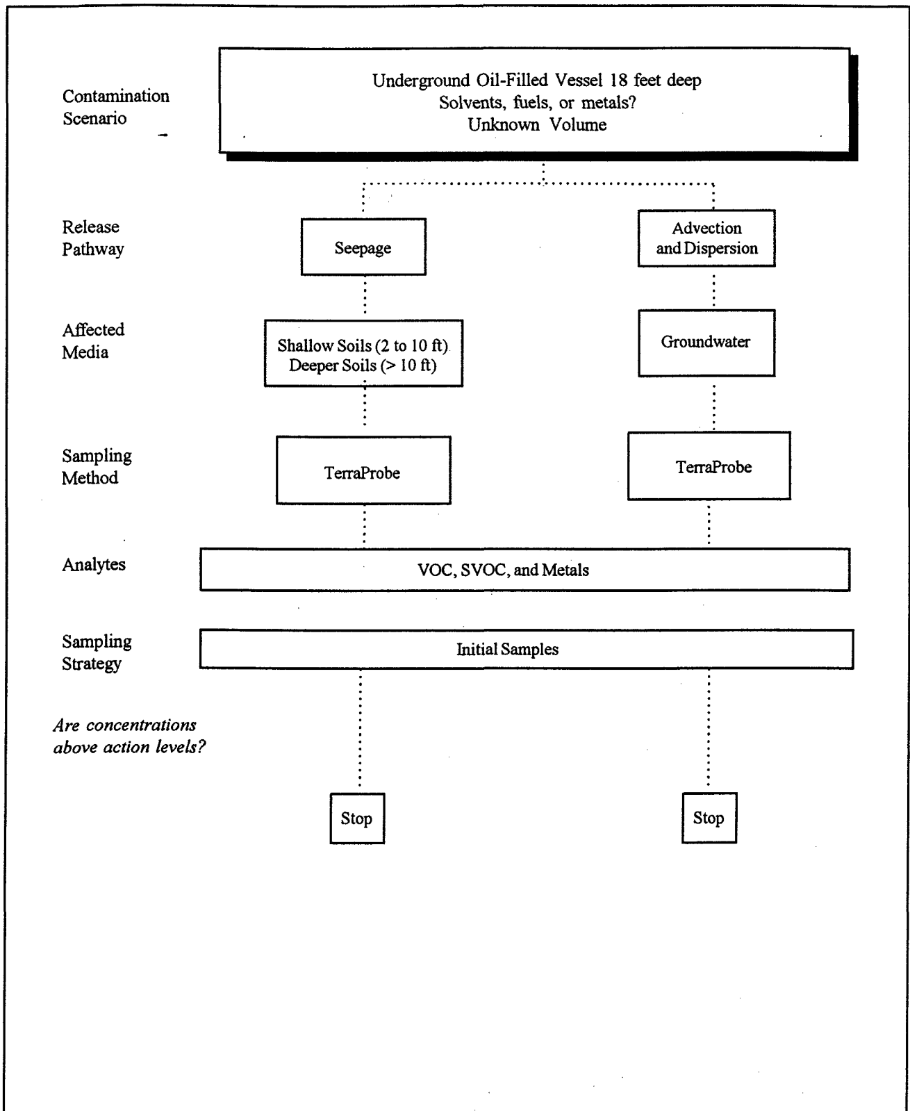
FIGURE 8-44 SAMPLING LOGIC DIAGRAM SITE 11 - WASTE OIL VESSEL, BLDG. 230 106 RESCUE GROUP, NYANG WESTHAMPTON BEACH, NEW YORK
