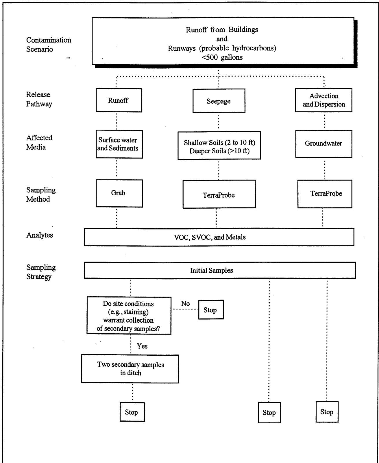
FIGURE 8-20 SAMPLING LOGIC DIAGRAM SITE 5 - SOUTHWEST STORM DRAINAGE DITCH 106 RESCUE GROUP, NYANG WESTHAMPTON BEACH, NEW YORK
