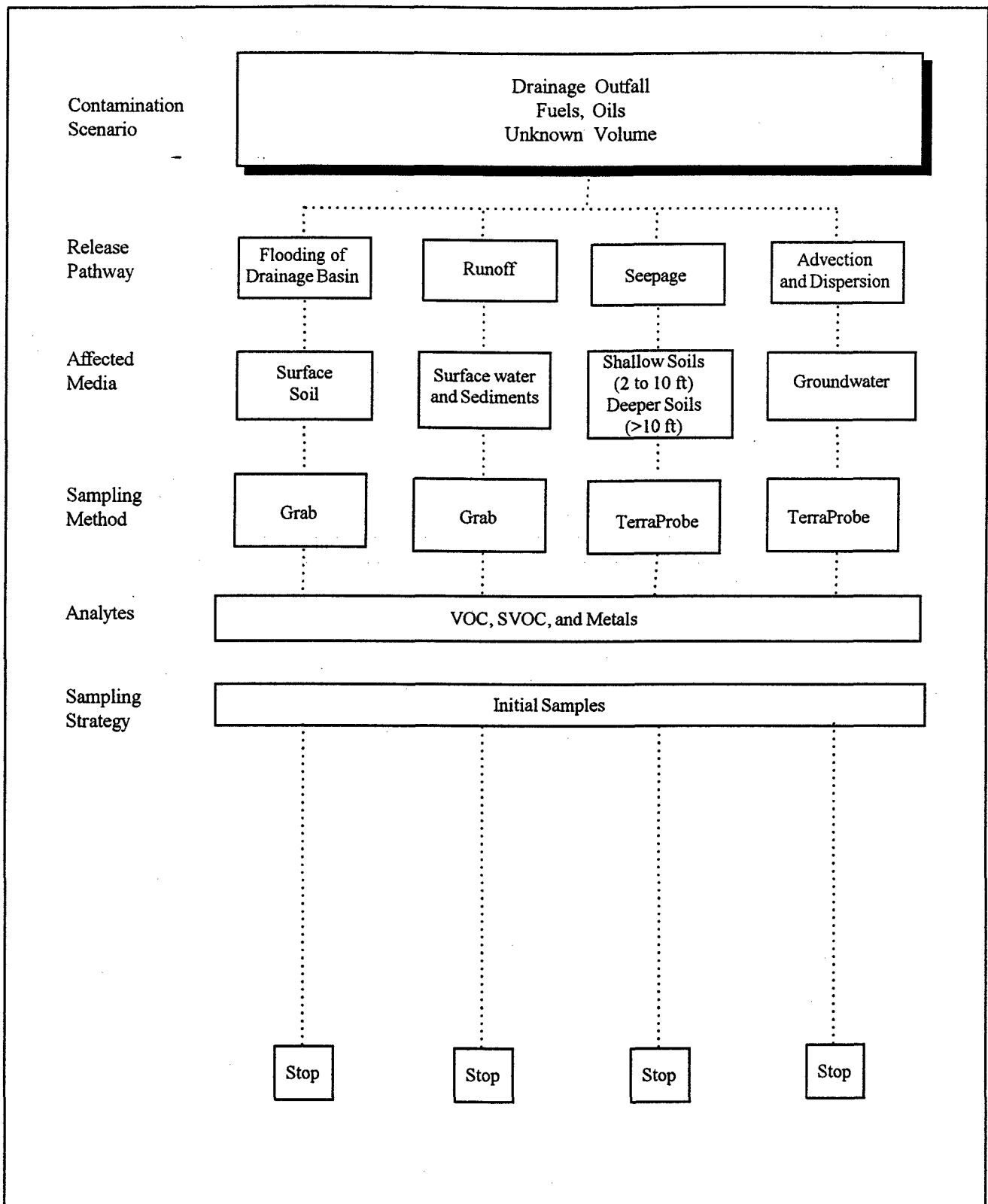
FIGURE 8-38 SAMPLING LOGIC DIAGRAM SITE 9 - RAMP DRAINAGE OUTFALL 106 RESCUE GROUP, NYANG WESTHAMPTON BEACH, NEW YORK
