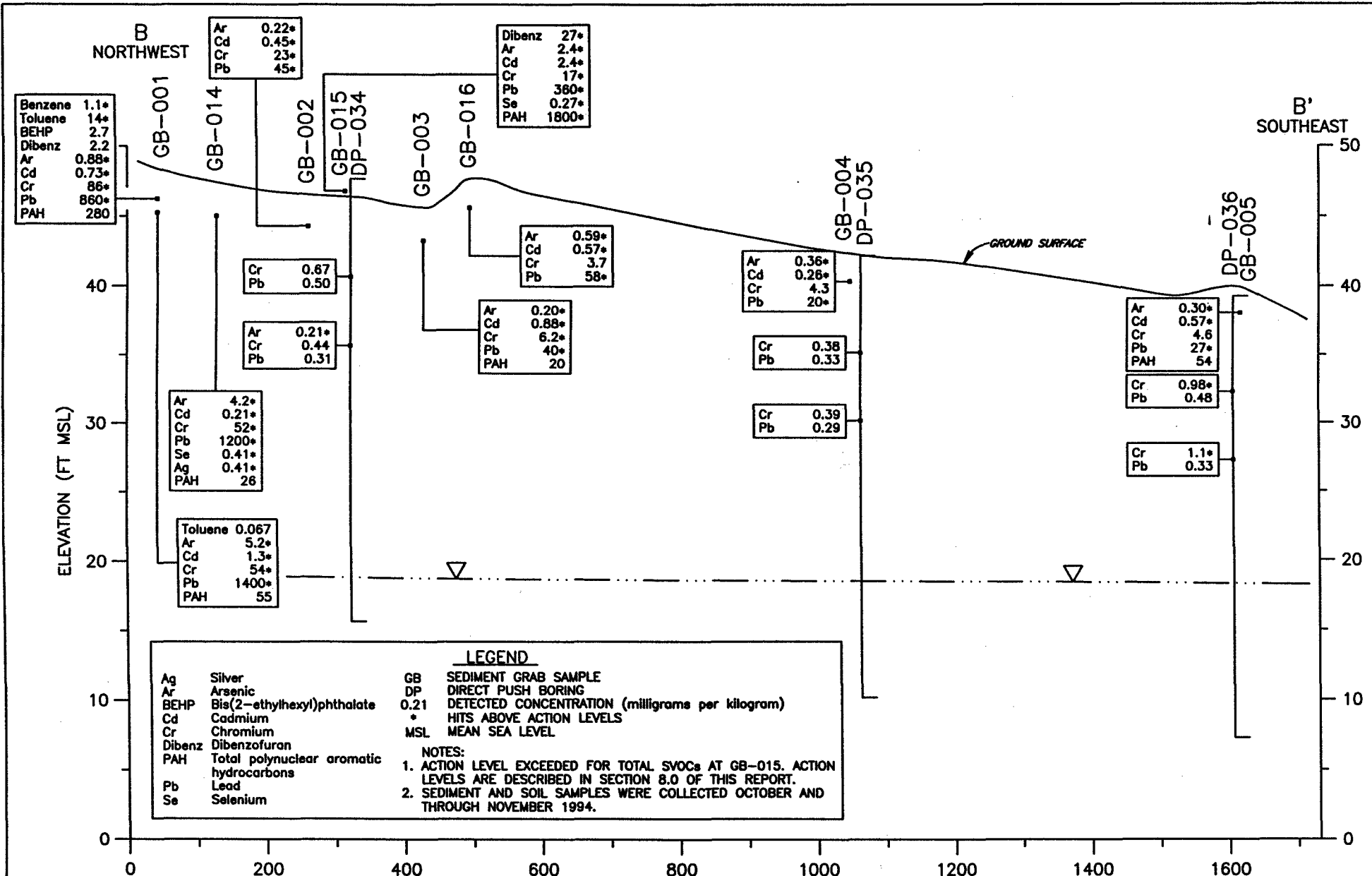
FIGURE 8-23 DETECTED CONCENTRATIONS IN SEDIMENT AND SUBSURFACE SOILS 106TH RESCUE GROUP, NYANG WESTHAMPTON BEACH, NEW YORK ABB Environmental Services, Inc.
