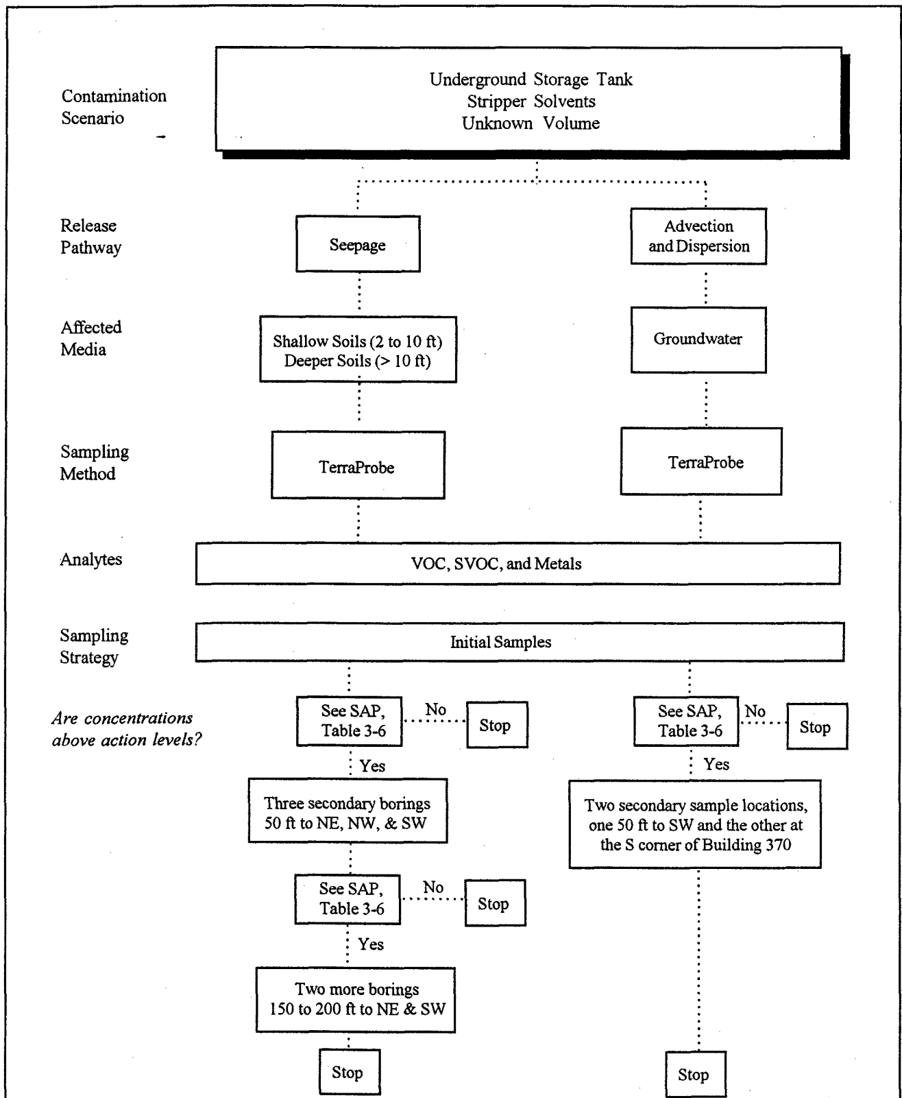
FIGURE 8-42 SAMPLING LOGIC DIAGRAM SITE 10 - WASTE STRIPPER TANK #61, BLDG. 370 106 RESCUE GROUP, NYANG WESTHAMPTON BEACH, NEW YORK
