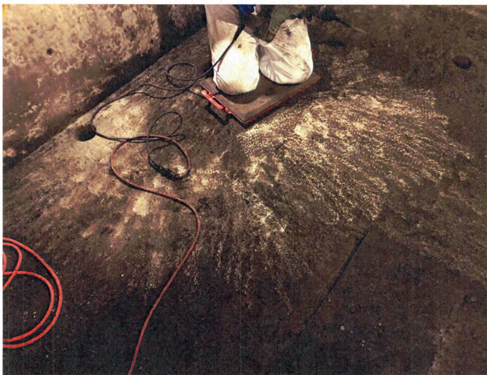
Limited PCB-Impacted Concrete Removal via Chipping Gun
