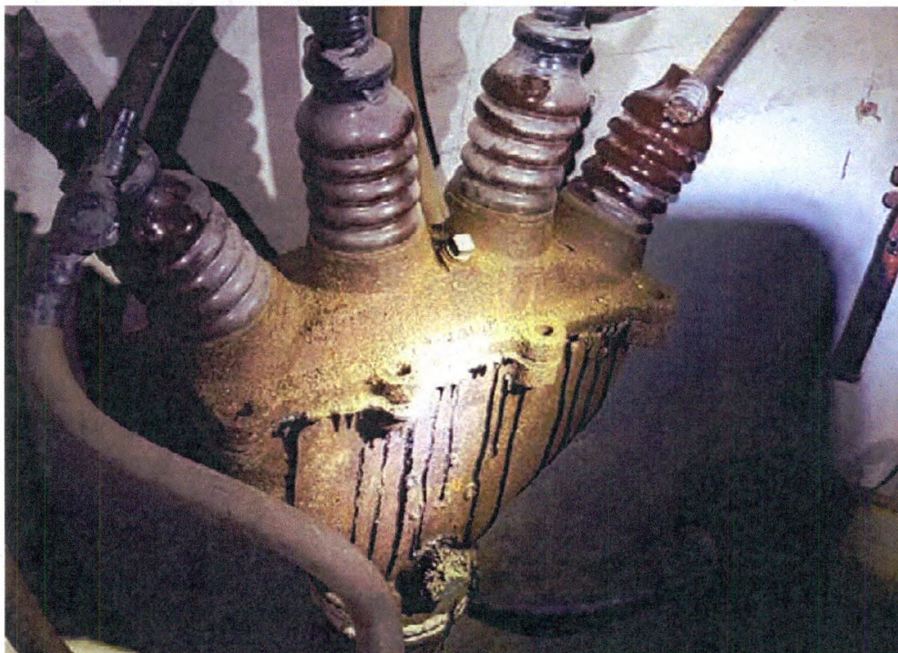
Polychlorinated Biphenyl (PCB) Fluid Dried on Exterior of Transformer
