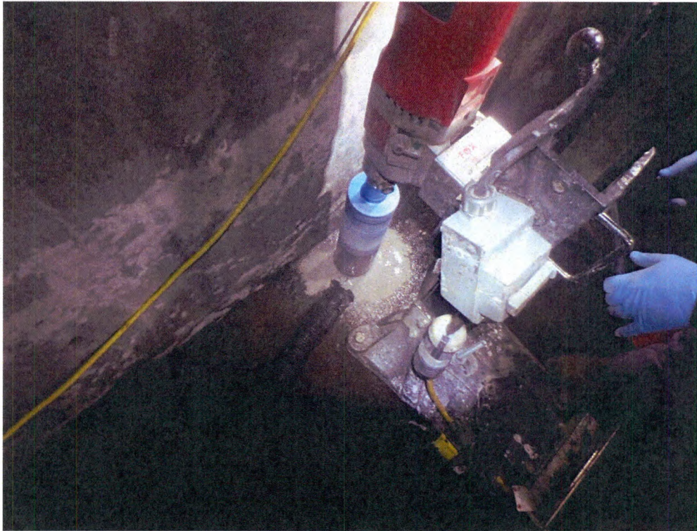
Concrete Sampling via Core Drill with Continuous Mist and HEPA Vacuum
