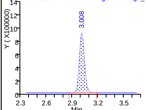
22 Perfluorooctane Sulfonamide
