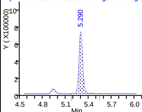
46 Perfluorooctadecanoic acid
