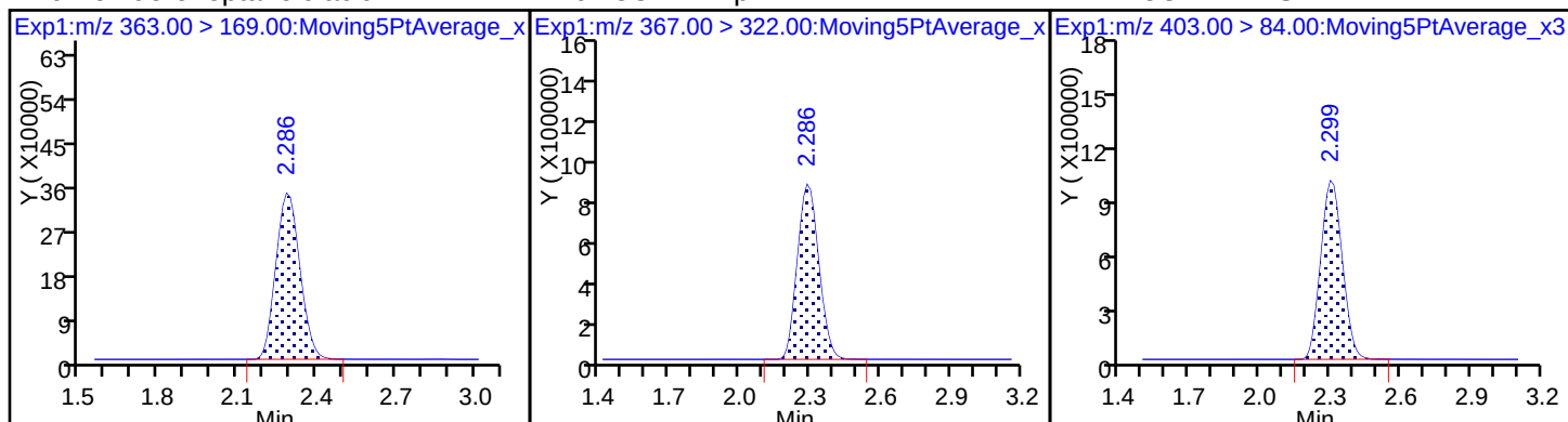
8 Perfluorohexanesulfonic acid
