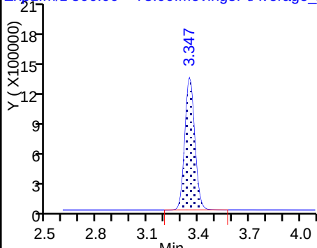
25 Sodium 1H,1H,2H,2H-perfluorodeca
