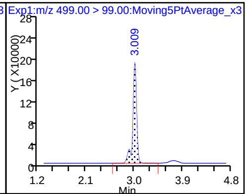
20 Perfluorononanoic acid
