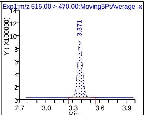
25 Sodium 1H,1H,2H,2H-perfluorodecanoate
