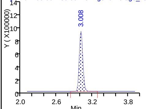
20 Perfluorononanoic acid
