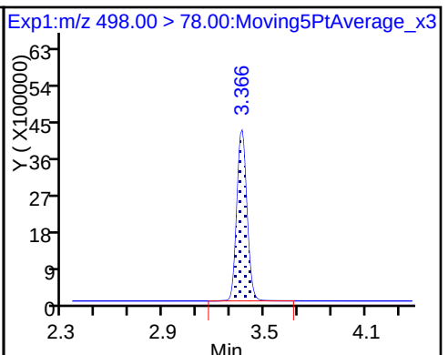
25 Sodium 1H,1H,2H,2H-perfluorodeca
