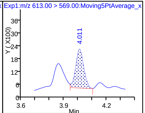
37 Perfluorododecanoic acid
