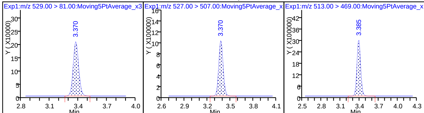
25 Sodium 1H,1H,2H,2H-perfluorodecanoate
