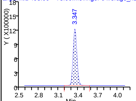
25 Sodium 1H,1H,2H,2H-perfluorodeca
