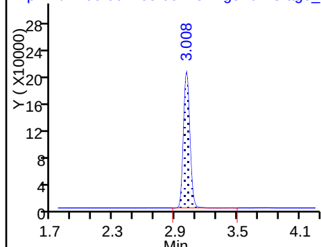
20 Perfluorononanoic acid
