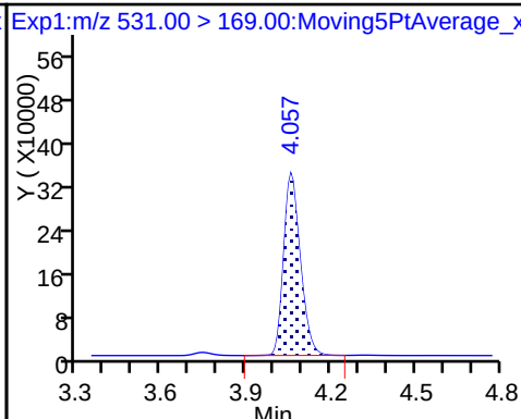
41 Perfluorotridecanoic acid
