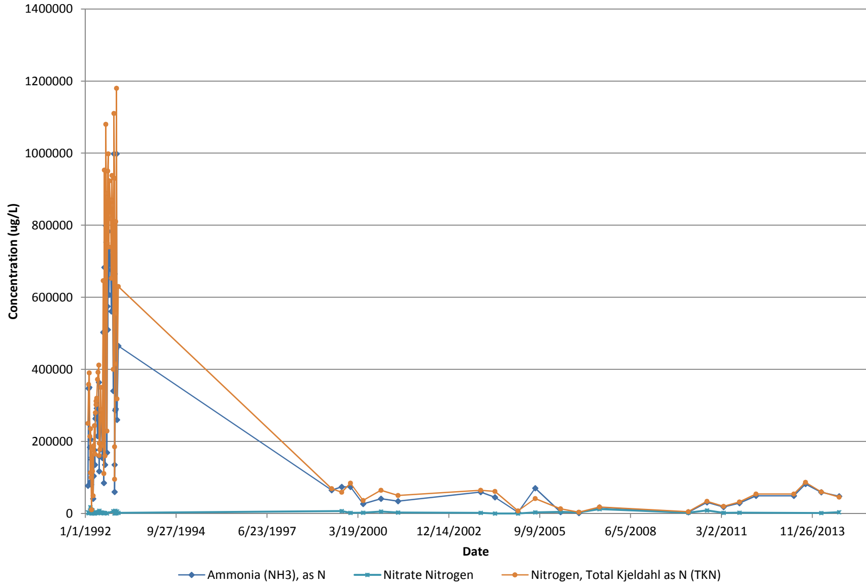
Figure 5: Concentrations of Ammonia, Nitrate Nitrogen, and Total Kjeldahl Nitrogen Versus Time in Leachate Samples Pelham Bay Landfill, Bronx, New York
