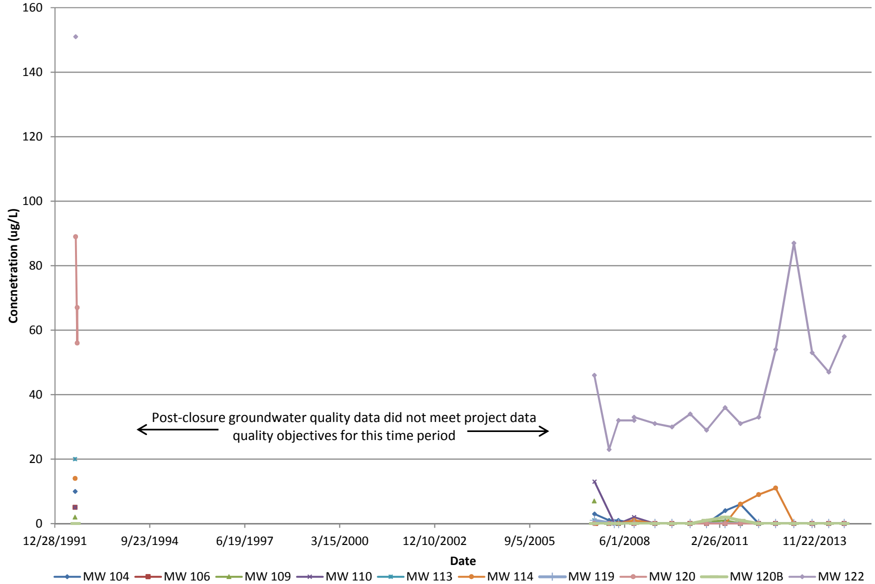
Figure 8: Concentration of Total VOCs Versus Time in Groundwater Samples Pelham Bay Landfill, Bronx, New York
