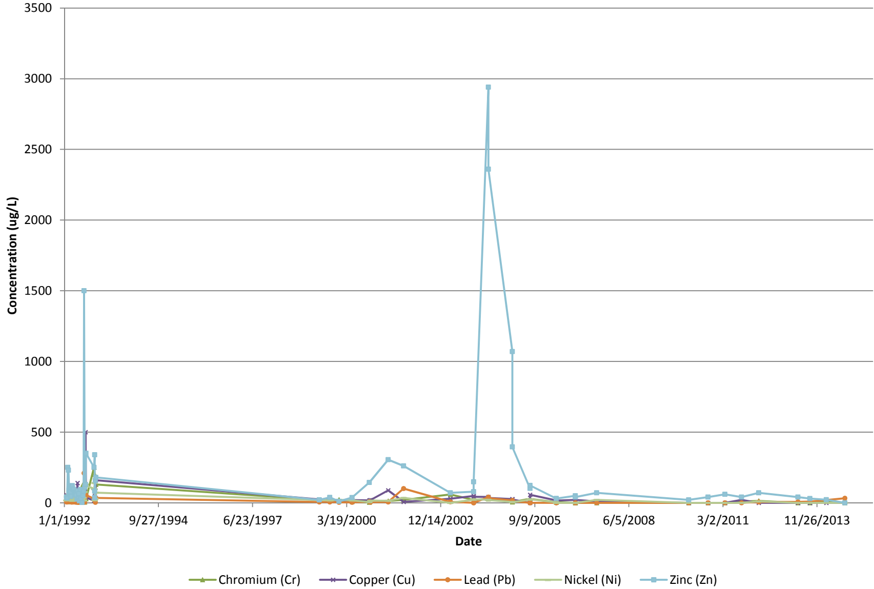
Figure 3: Concentrations of Select Inorganic Compounds Versus Time in Leachate Samples Pelham Bay Landfill, Bronx, New York
