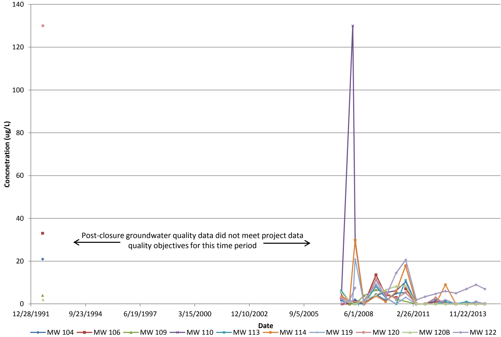
Figure 9: Concentration of Total SVOCs Versus Time in Groundwater Samples Pelham Bay Landfill, Bronx, New York
