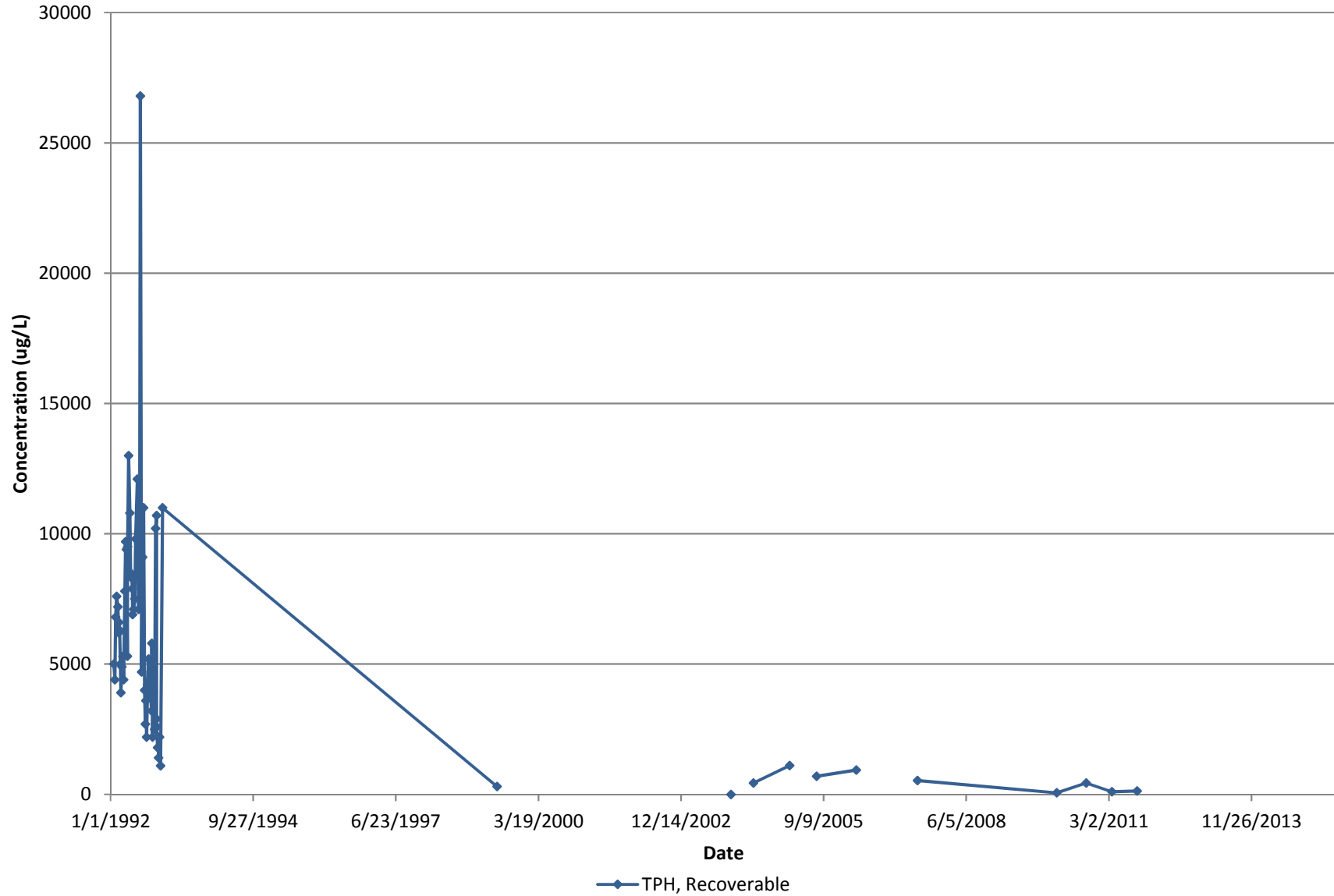
Figure 1: Concentration of Total Petroleum Hydrocarbons Versus Time in Leachate Samples Pelham Bay Landfill, Bronx, New York
