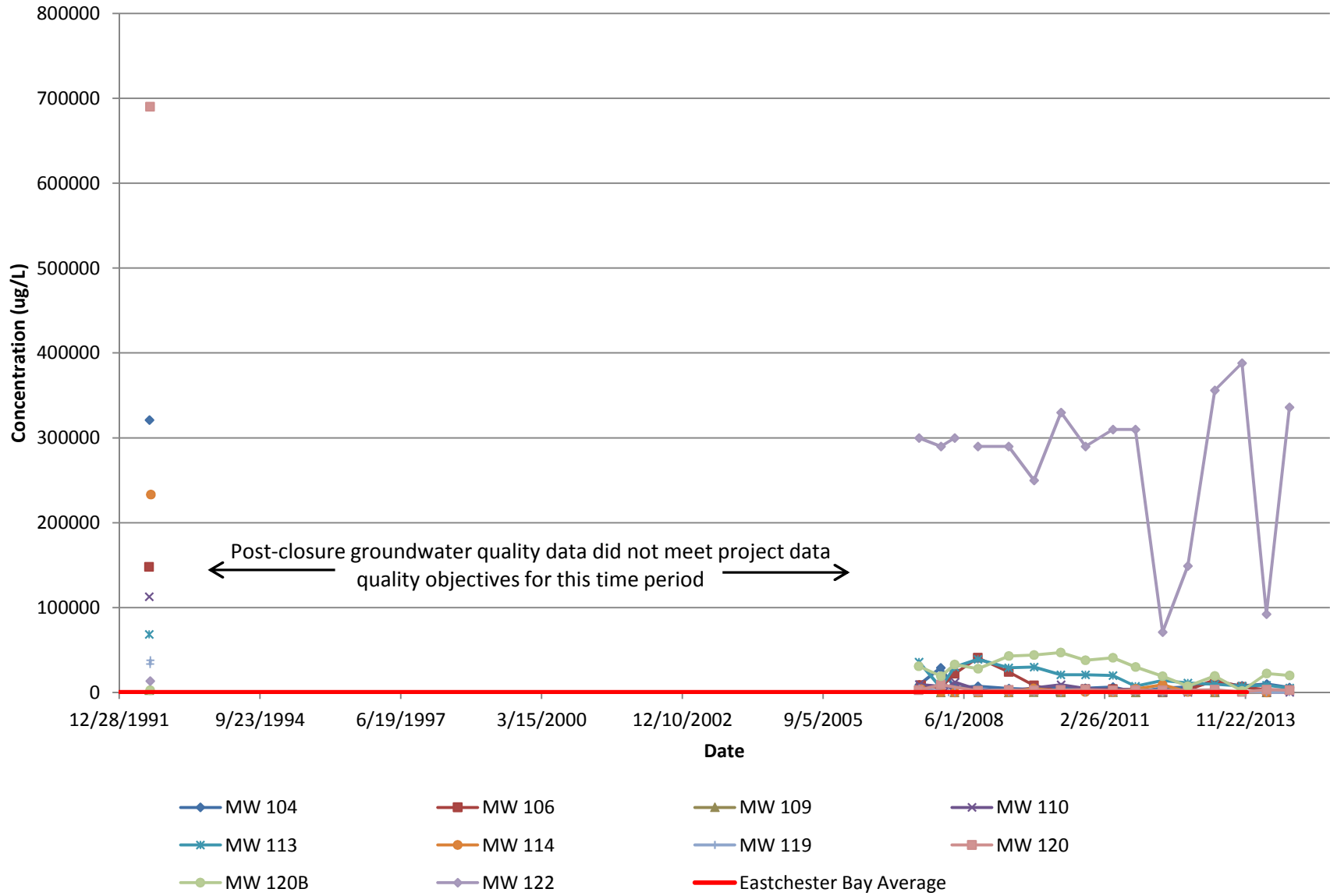
Figure 11: Concentration of Ammonia Versus Time in Groundwater Samples Pelham Bay Landfill, Bronx, New York
