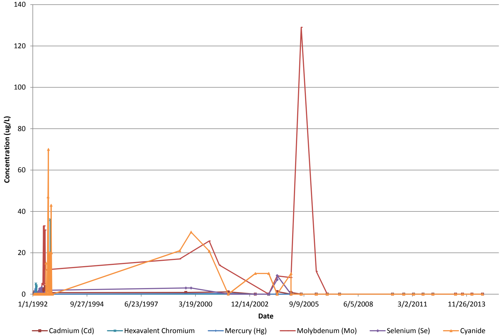
Figure 2: Concentrations of Select Inorganic Compounds Versus Time in Leachate Samples Pelham Bay Landfill, Bronx, New York
