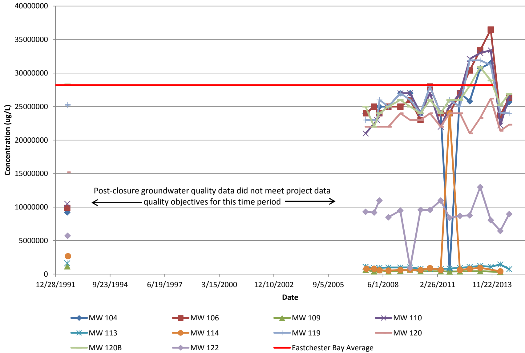
Figure 15: Concentration of Total Dissolved Solids Versus Time in Groundwater Samples Pelham Bay Landfill, Bronx, New York
