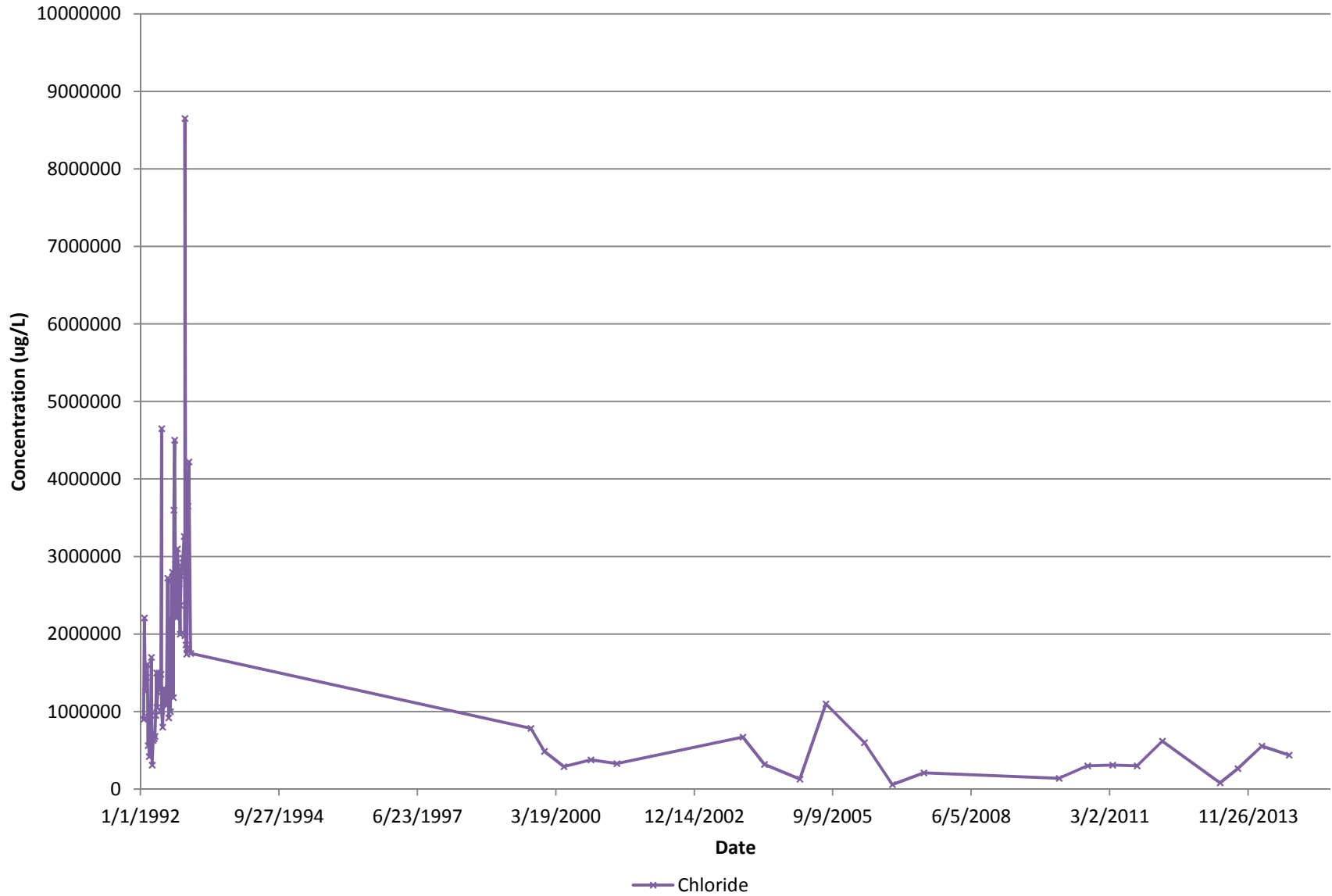
Figure 6: Concentration of Chloride Versus Time in Leachate Samples Pelham Bay Landfill, Bronx, New York
