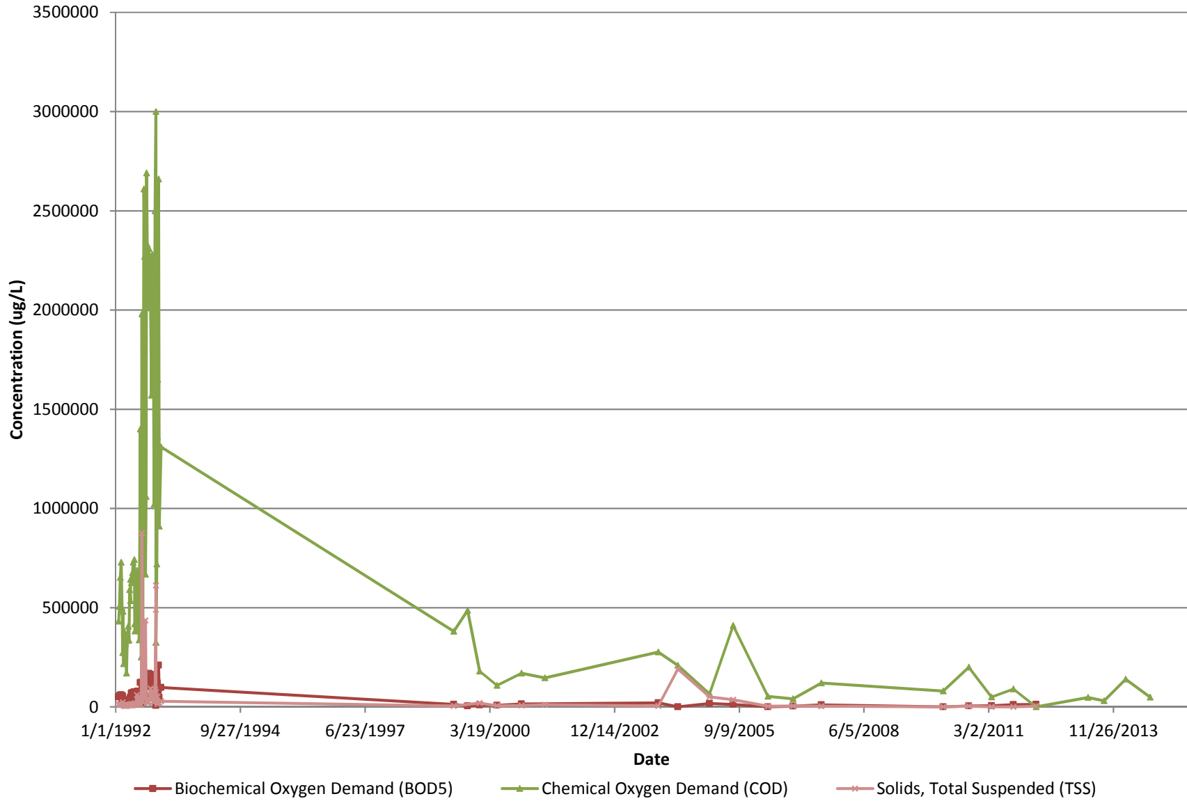
Figure 7: Concentrations of BOD, COD and Total Suspended Solids Versus Time in Leachate Samples Pelham Bay Landfill, Bronx, New York
