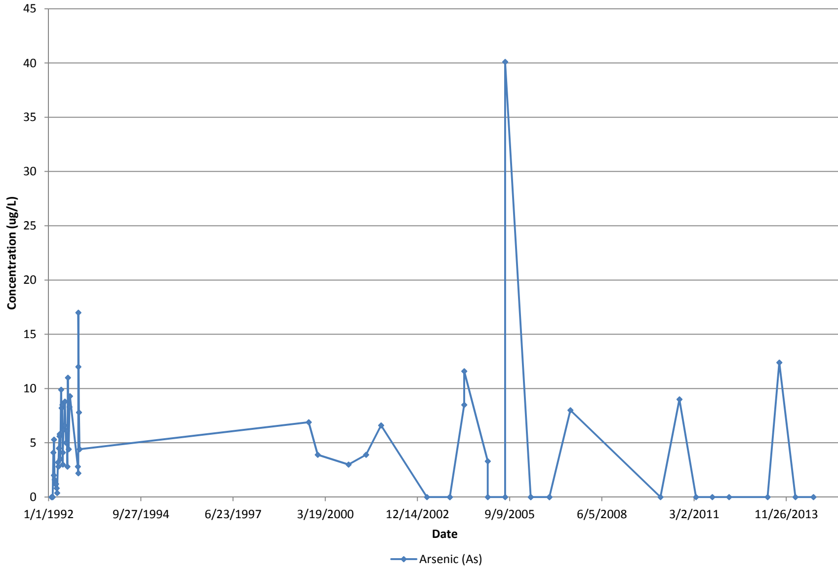
Figure 4: Concentration of Arsenic Versus Time in Leachate Samples Pelham Bay Landfill, Bronx, New York
