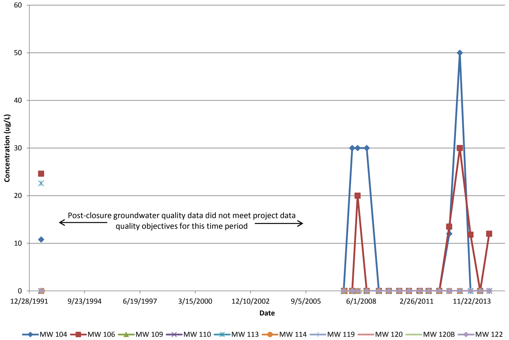
Figure 10: Concentration of Cyanide Versus Time in Groundwater Samples Pelham Bay Landfill, Bronx, New York
