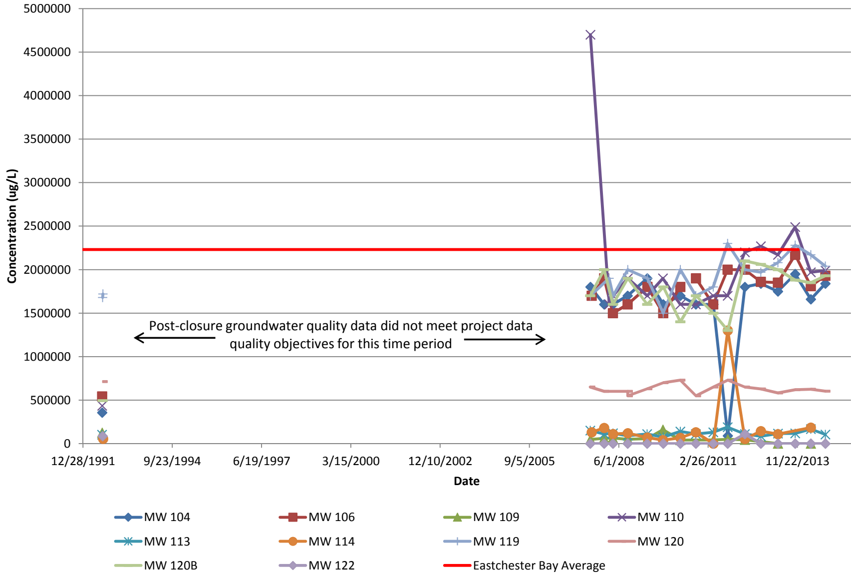
Figure 14: Concentration of Sulfate Versus Time in Groundwater Samples Pelham Bay Landfill, Bronx, New York
