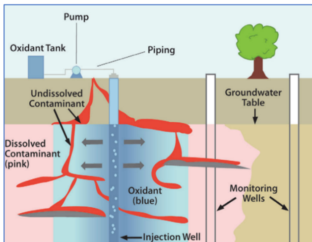
This graphic is a generic depiction (prepared by the US EPA) of ISCO injections. Additional details on ISCO injections can be accessed on the US EPA website: https://archive.epa.gov/ada/web/pdf/a_citizens_guide_to_in_situ_chemical_oxidation.pdf .
