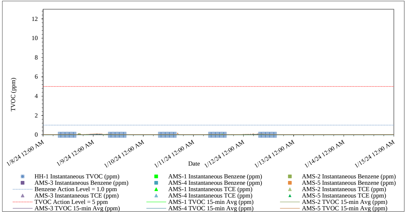
Figure 2 – Summary of TVOC, Benzene, and Tri-chloroethylene Concentrations 01/08/24 through 01/14/24
