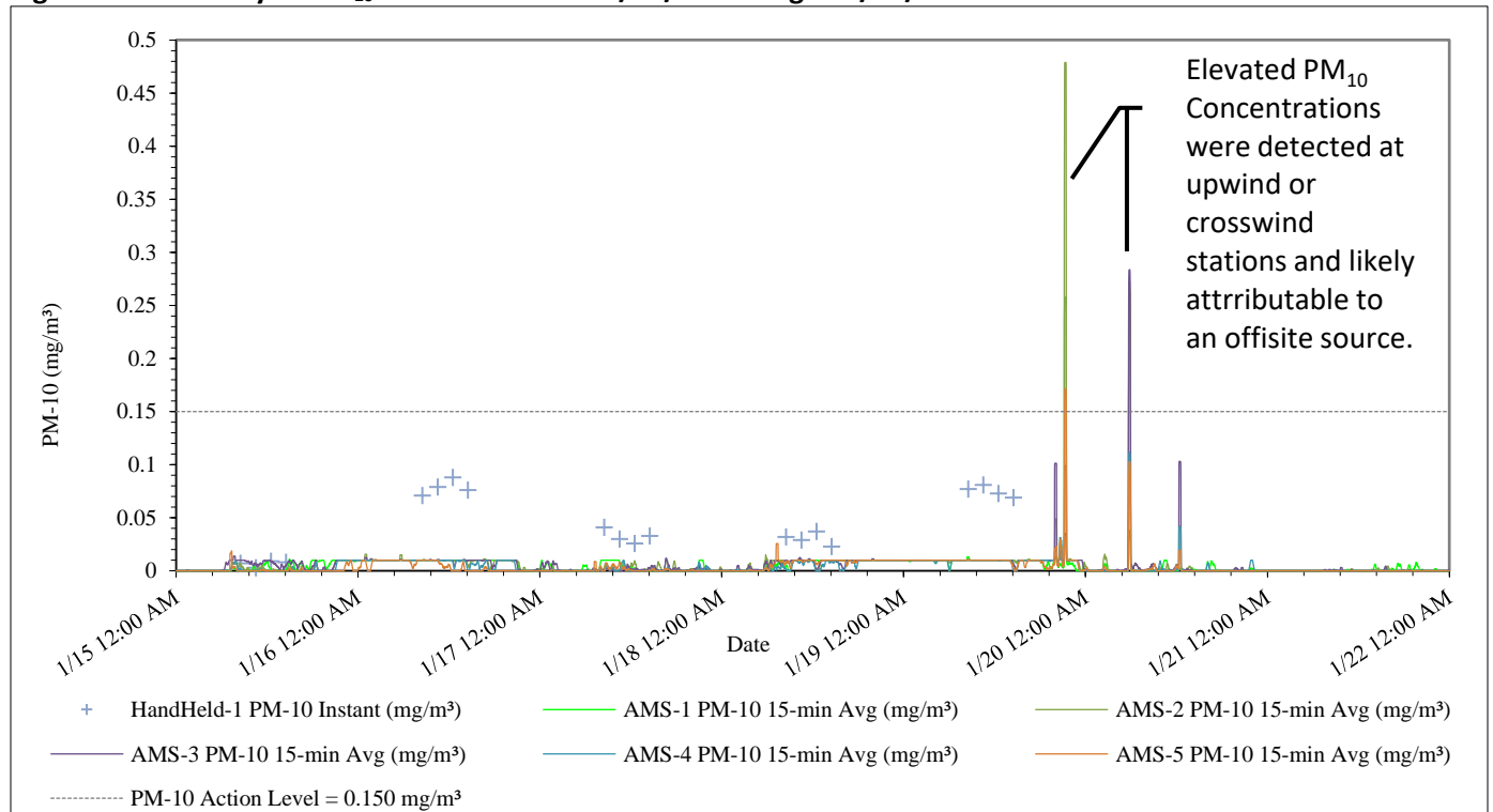
Figure 3 – Summary of PM 10 Concentrations 01/15/24 through 01/21/24
