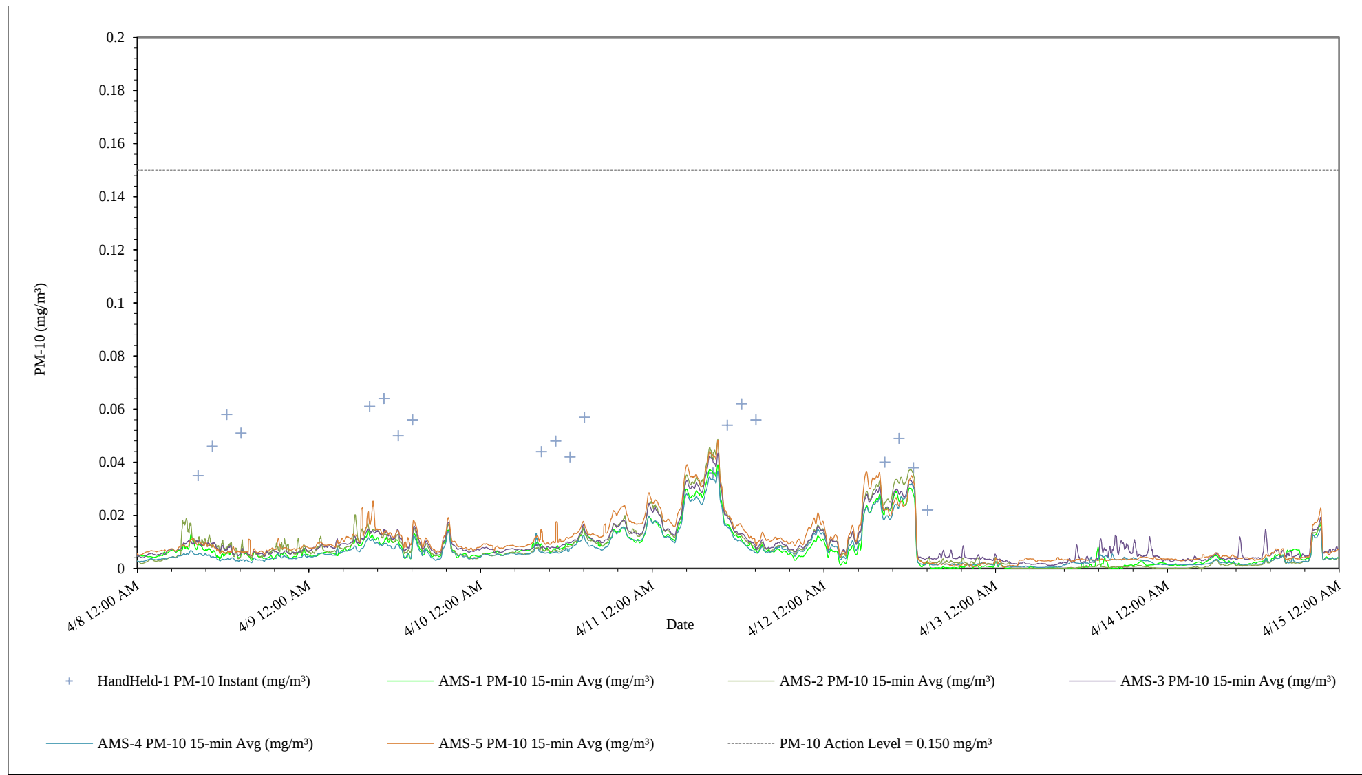
Figure 3 – Summary of PM 10 Concentrations 04/08/24 through 04/14/24
