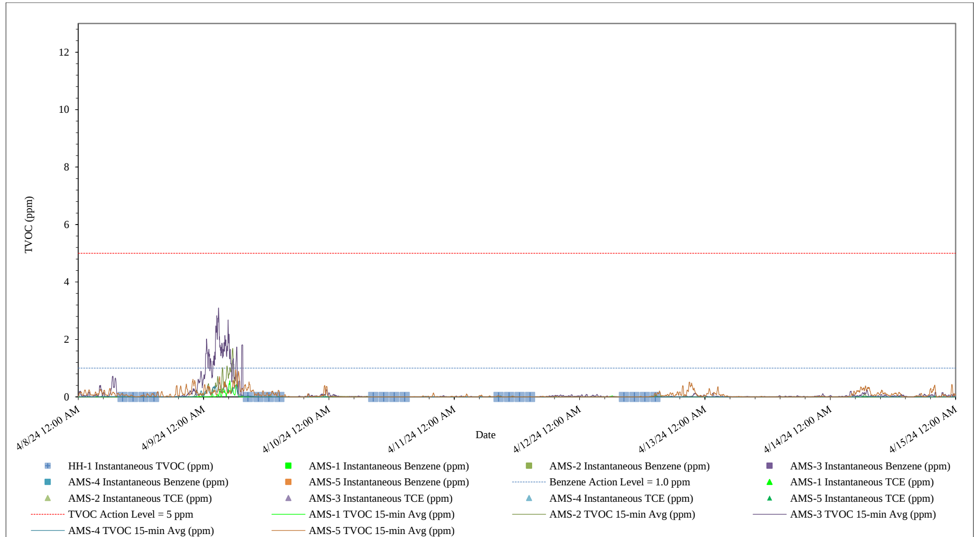
Figure 2 – Summary of TVOC, Benzene, and Tri-chloroethylene Concentrations 04/08/24 through 04/14/24
