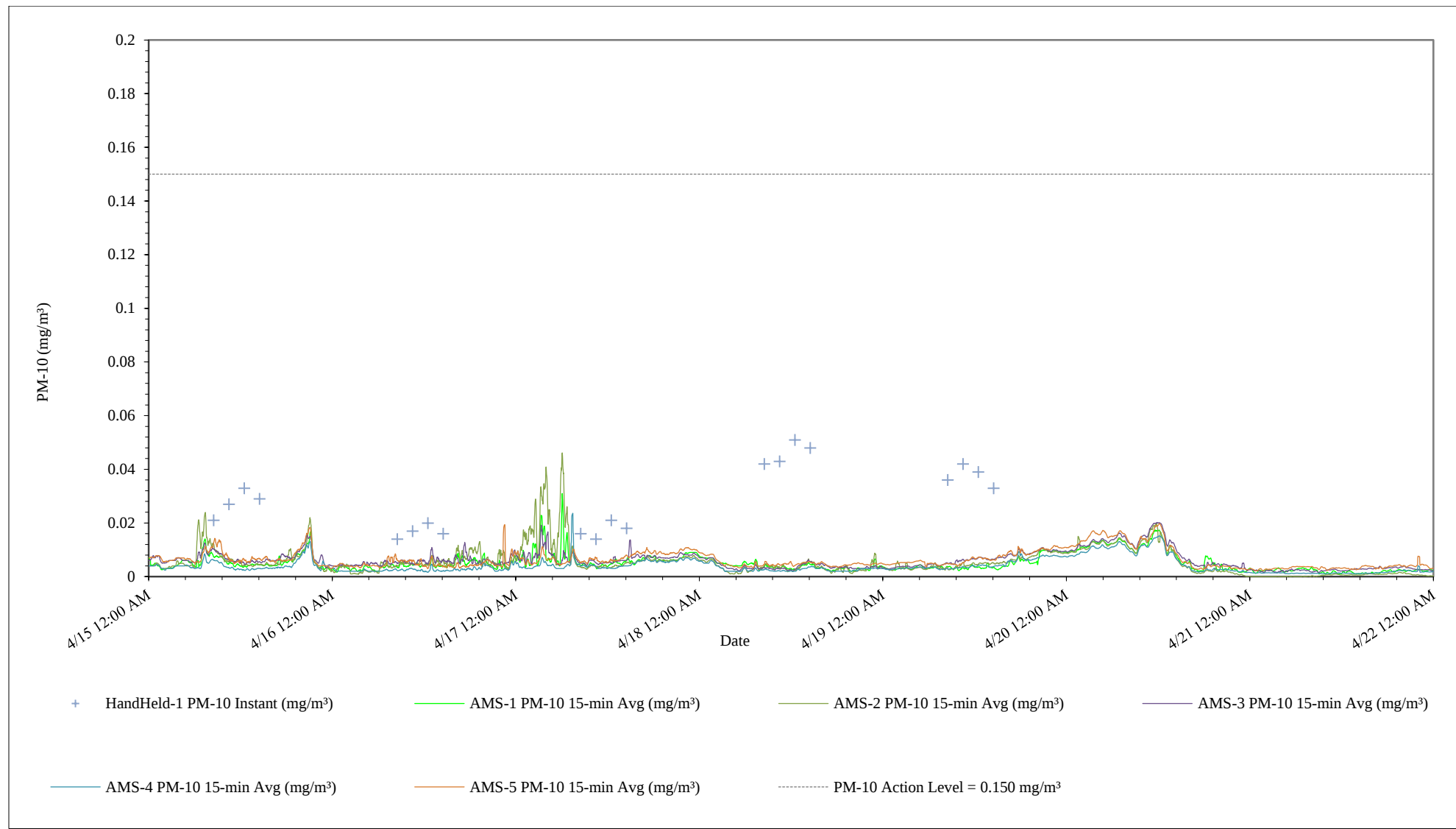
Figure 3 – Summary of PM 10 Concentrations 04/15/24 through 04/22/24
