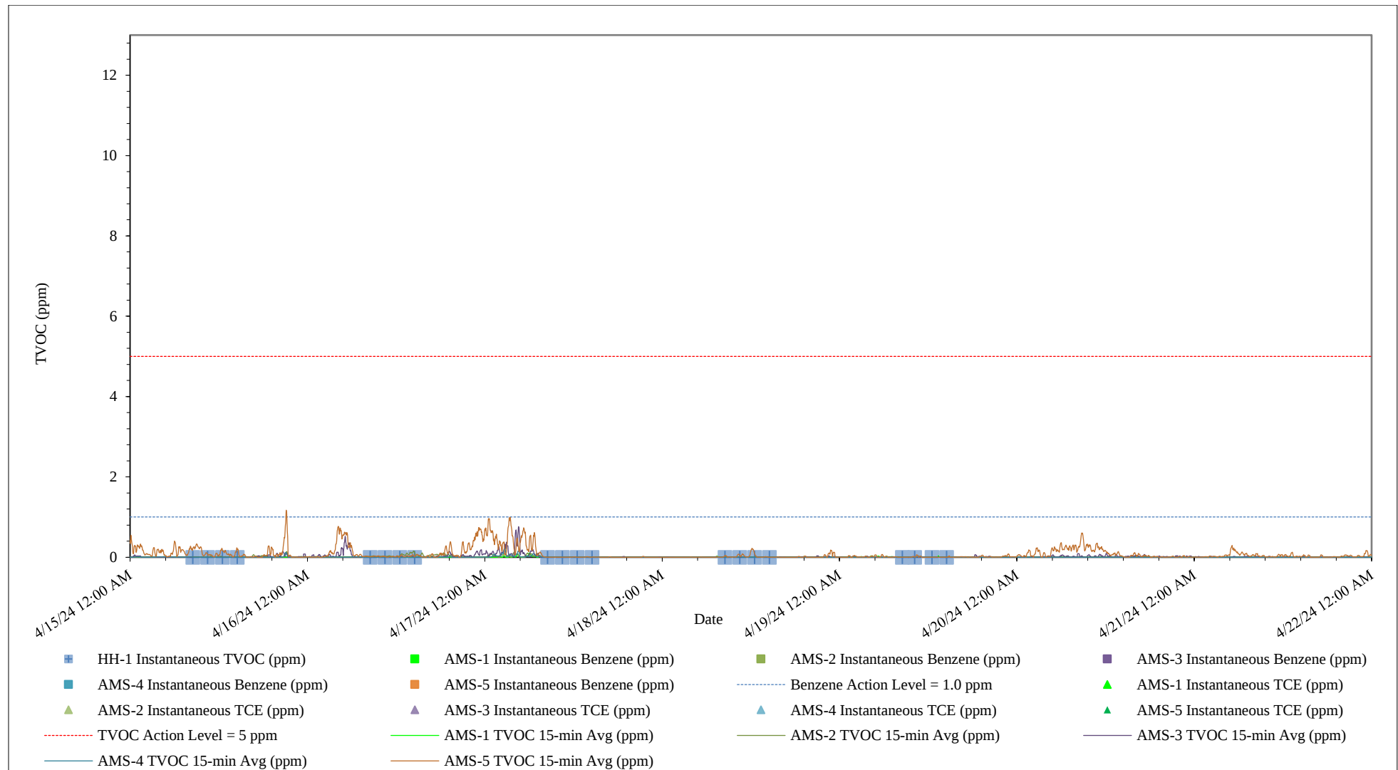
Figure 2 – Summary of TVOC, Benzene, and Tri-chloroethylene Concentrations 04/15/24 through 04/22/24
