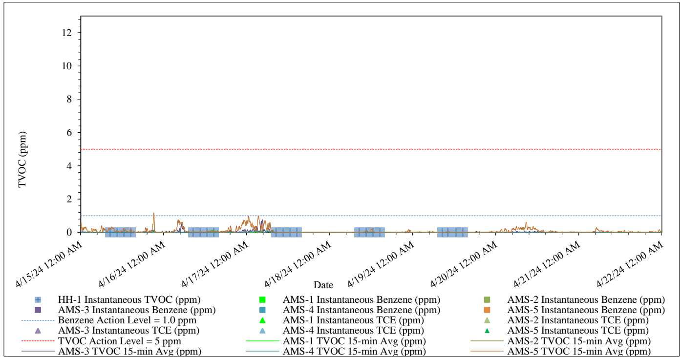
Figure 2 – Summary of TVOC, Benzene, and Tri-chloroethylene Concentrations 04/15/24 through 04/22/24
