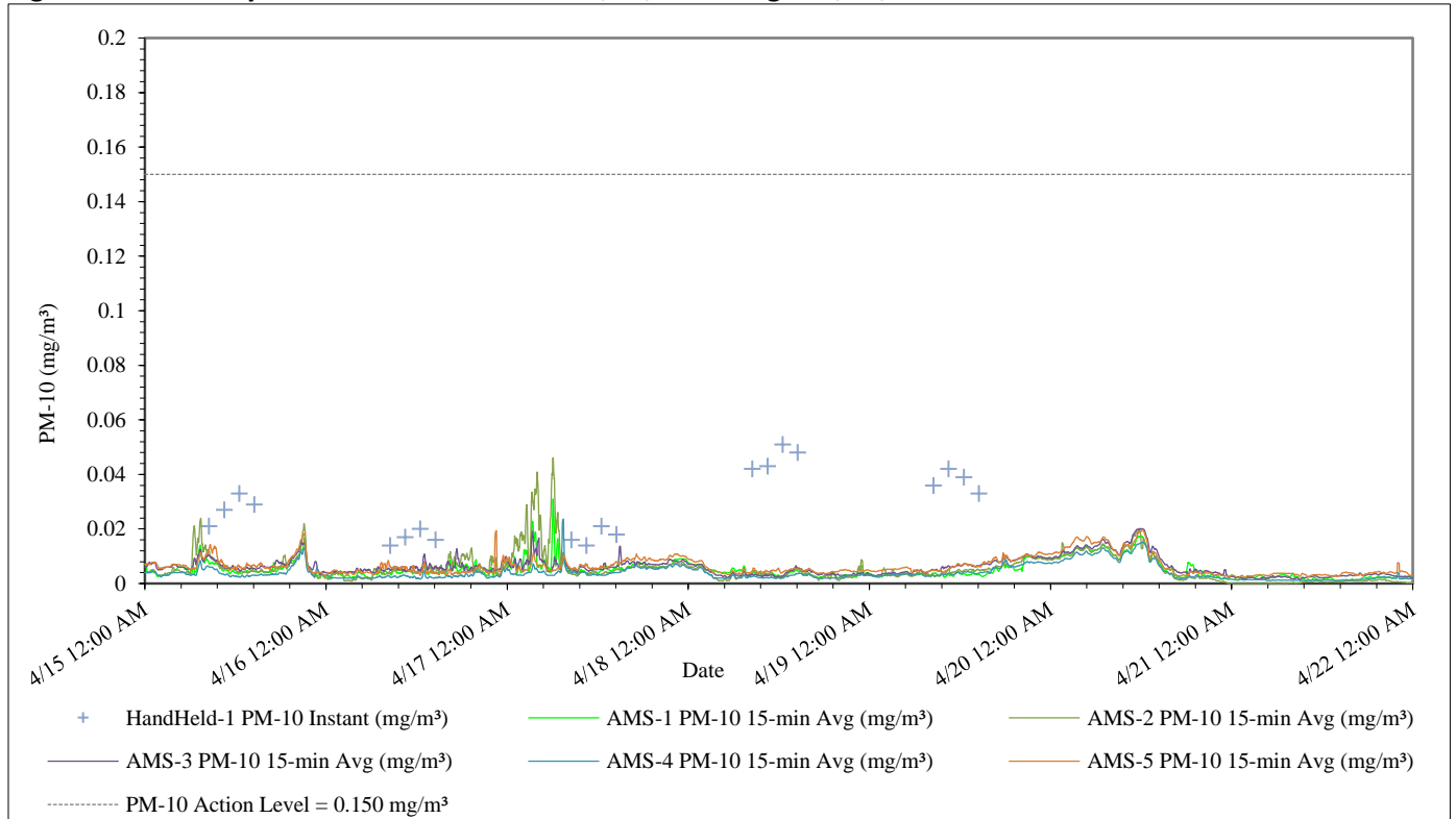
Figure 3 – Summary of PM 10 Concentrations 04/15/24 through 04/22/24
