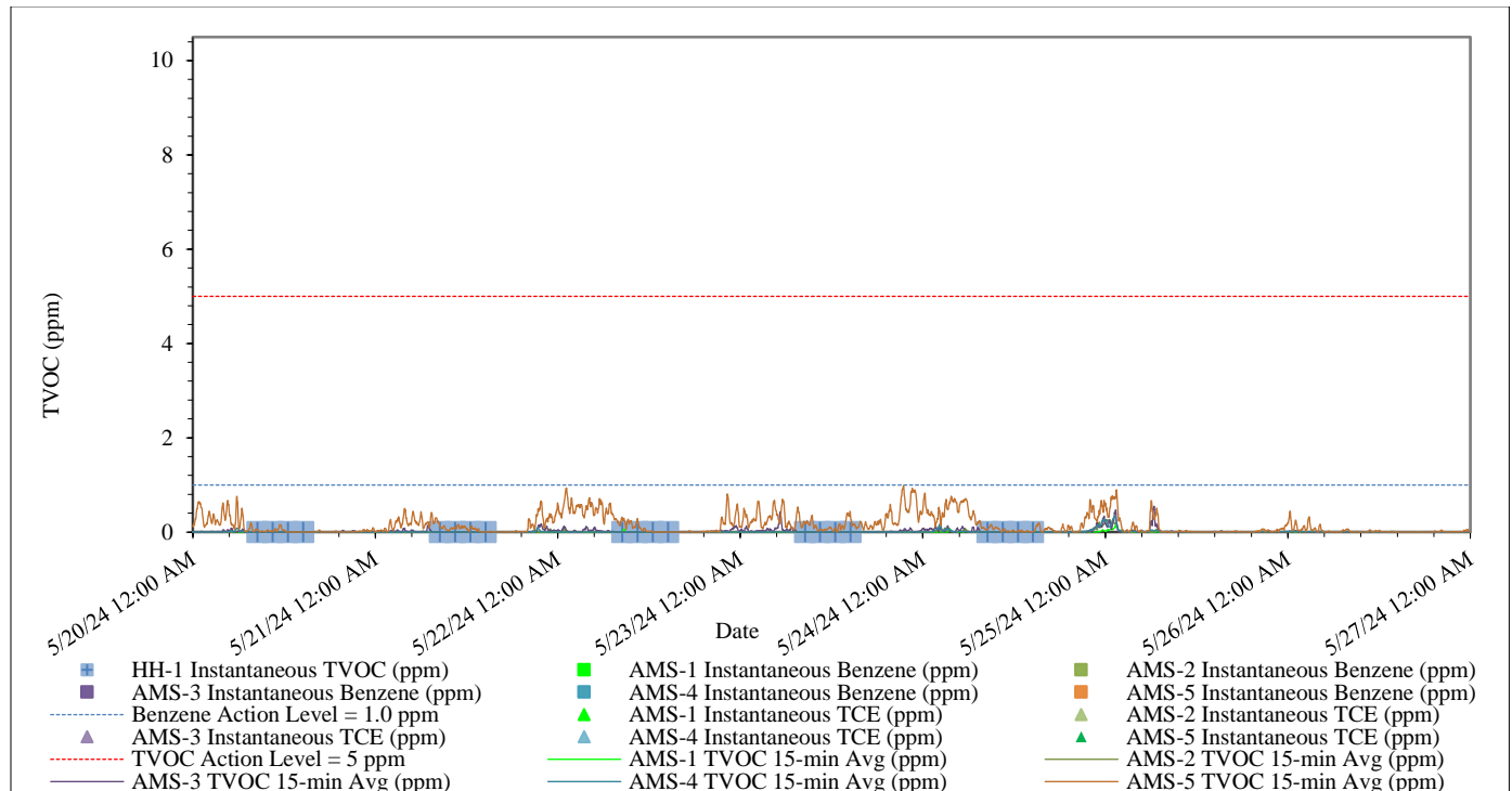
Figure 2 – Summary of TVOC, Benzene, and Tri-chloroethylene Concentrations 05/20/24 through 05/26/24
