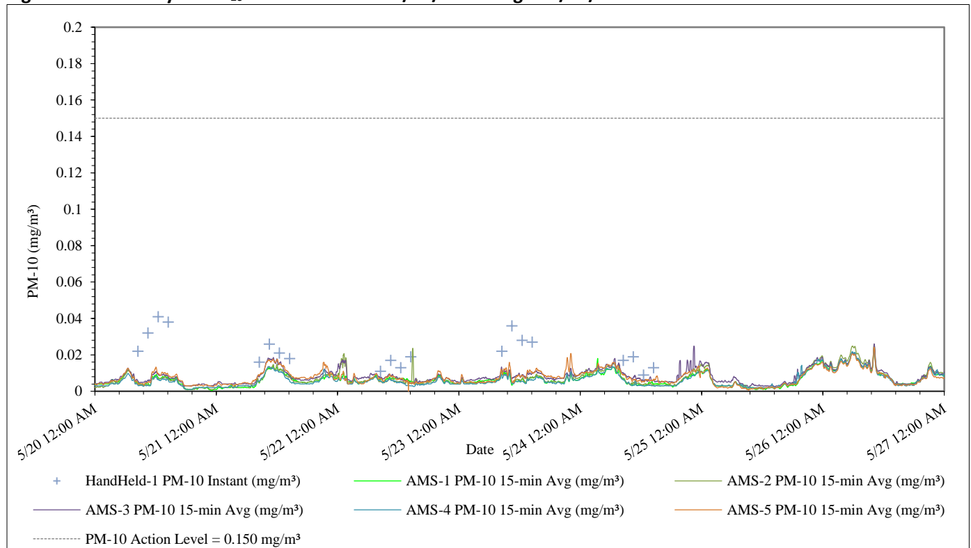
Figure 3 – Summary of PM 10 Concentrations 05/20/24 through 05/26/24
