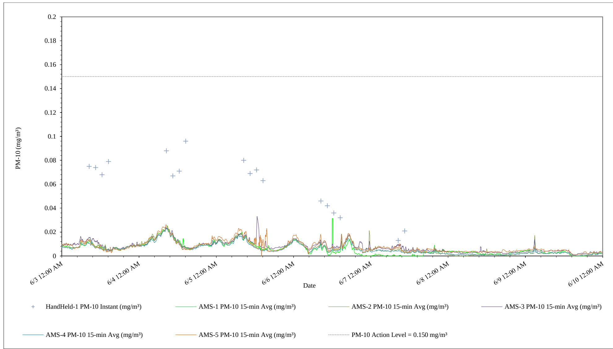
Figure 3 – Summary of PM 10 Concentrations 06/03/24 through 06/09/24
