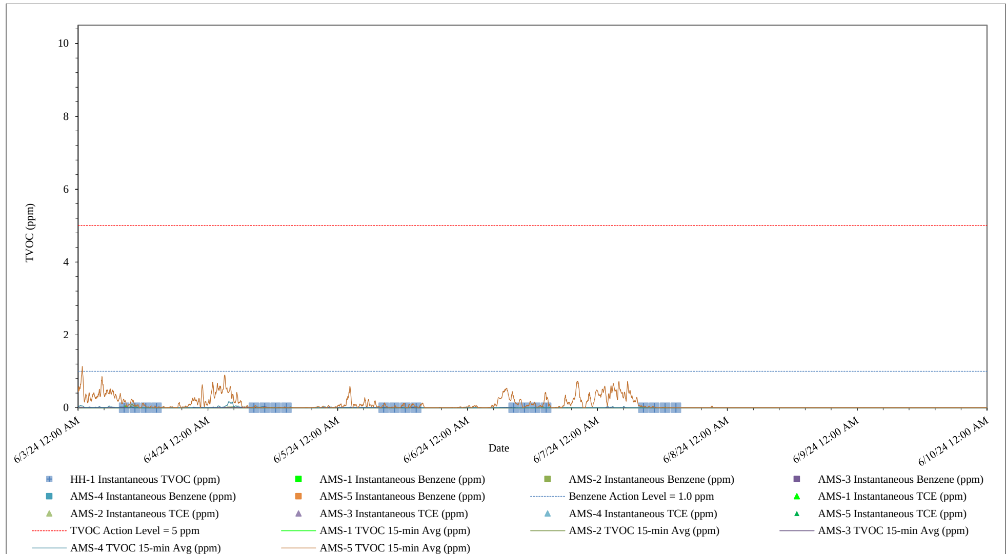
Figure 2 – Summary of TVOC, Benzene, and Tri-chloroethylene Concentrations 06/03/24 through 06/09/24
