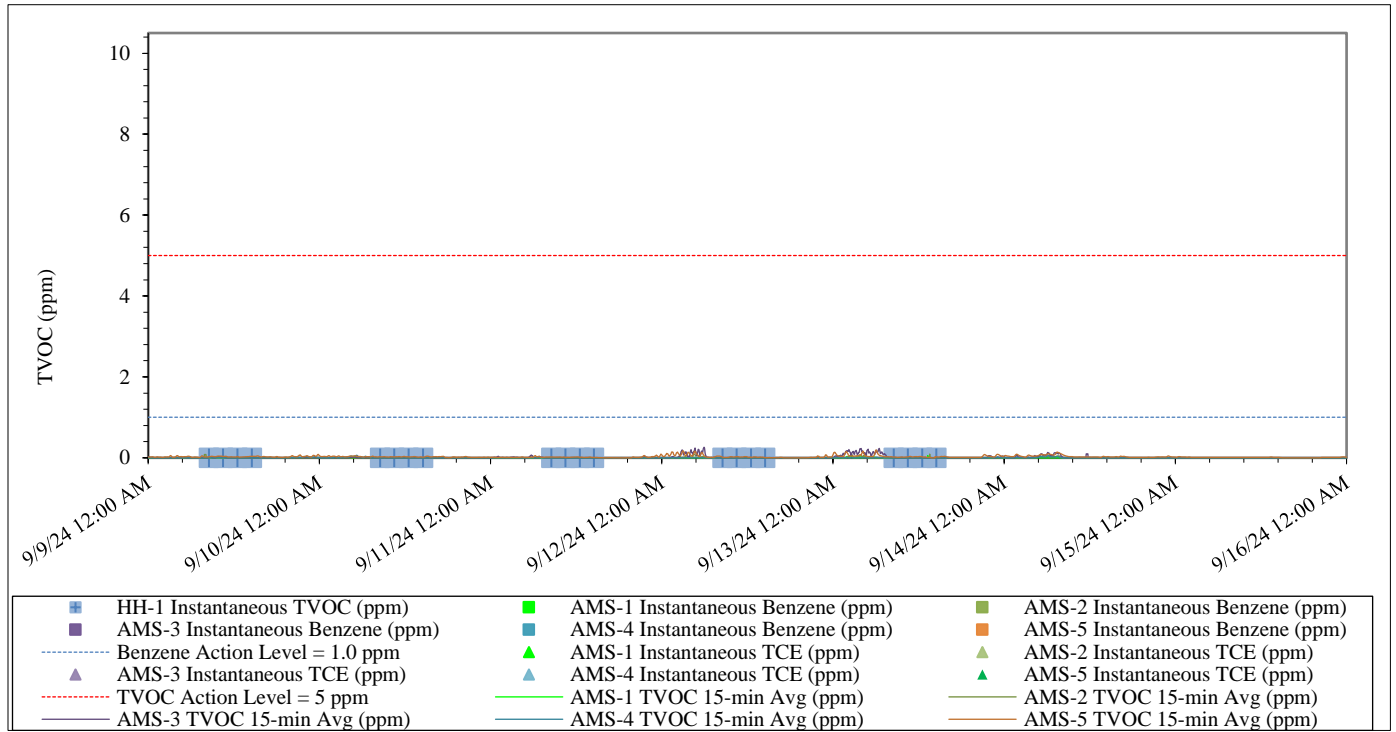
Figure 2 – Summary of TVOC, Benzene, and Tri-chloroethylene Concentrations 09/09/24 through 09/15/24
