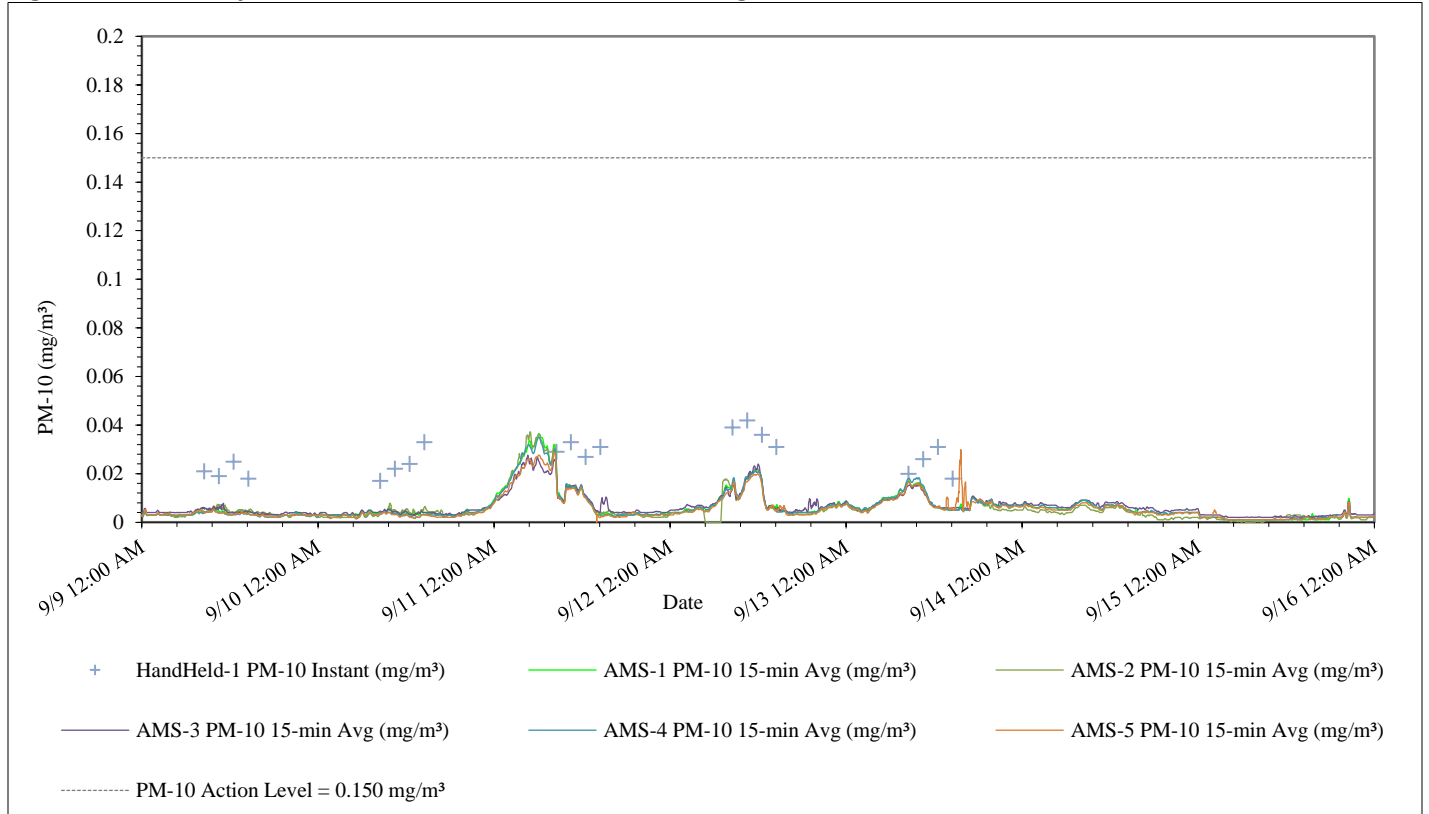
Figure 3 – Summary of PM 10 Concentrations 09/09/24 through 09/15/24
