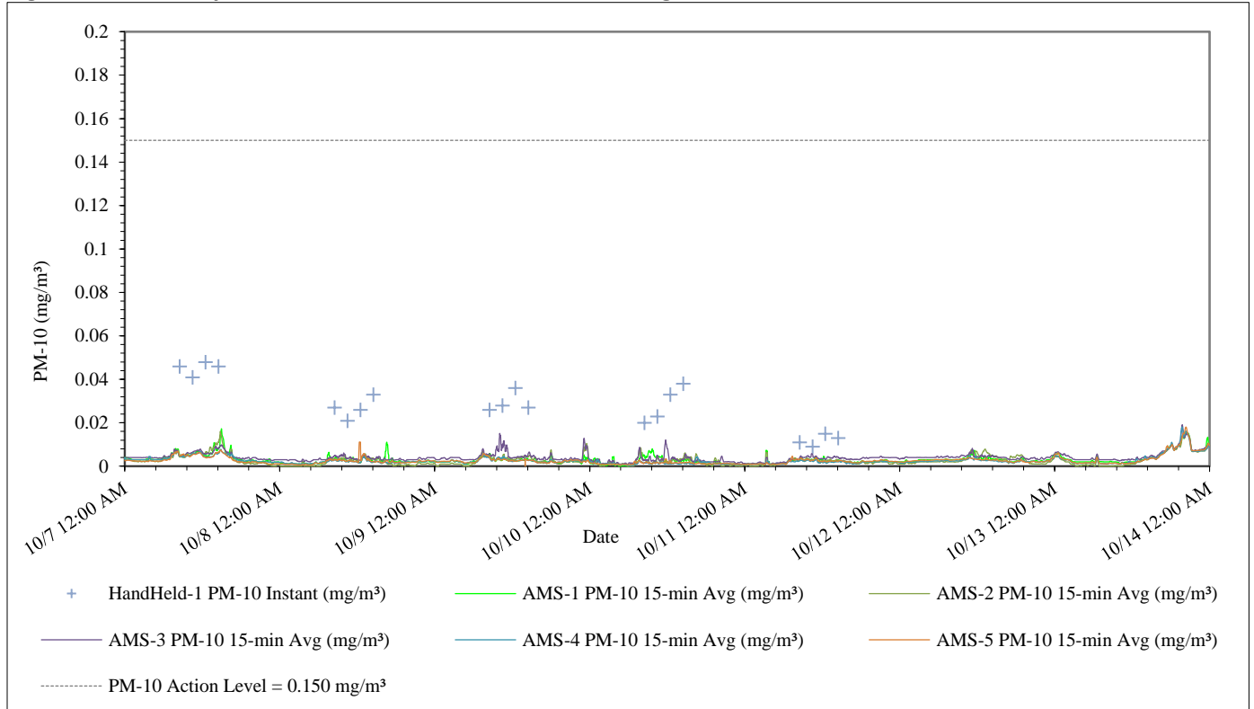
Figure 3 – Summary of PM 10 Concentrations 10/07/24 through 10/13/24
