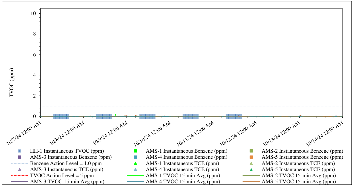
Figure 2 – Summary of TVOC, Benzene, and Tri-chloroethylene Concentrations 10/07/24 through 10/13/24
