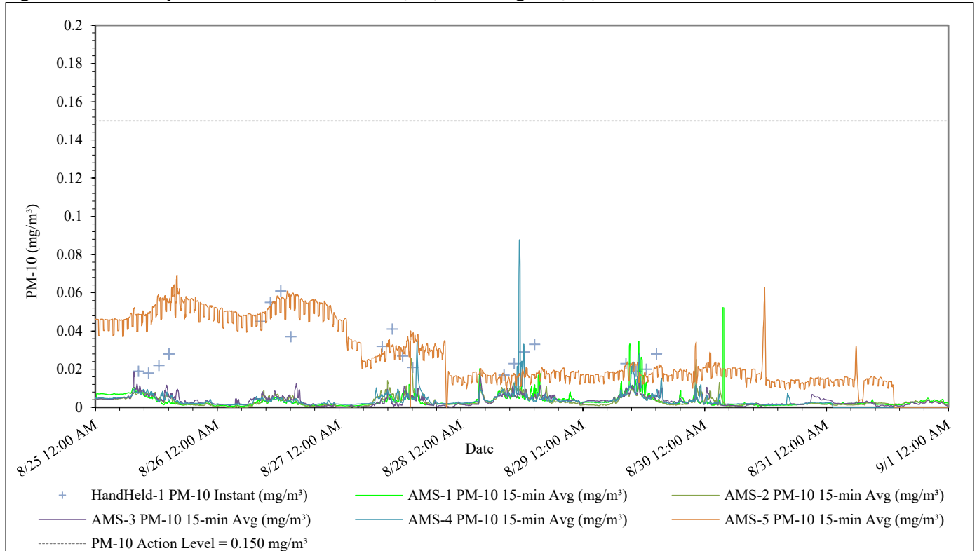
Figure 3 – Summary of PM 10 Concentrations 08/25/25 through 08/31/25
