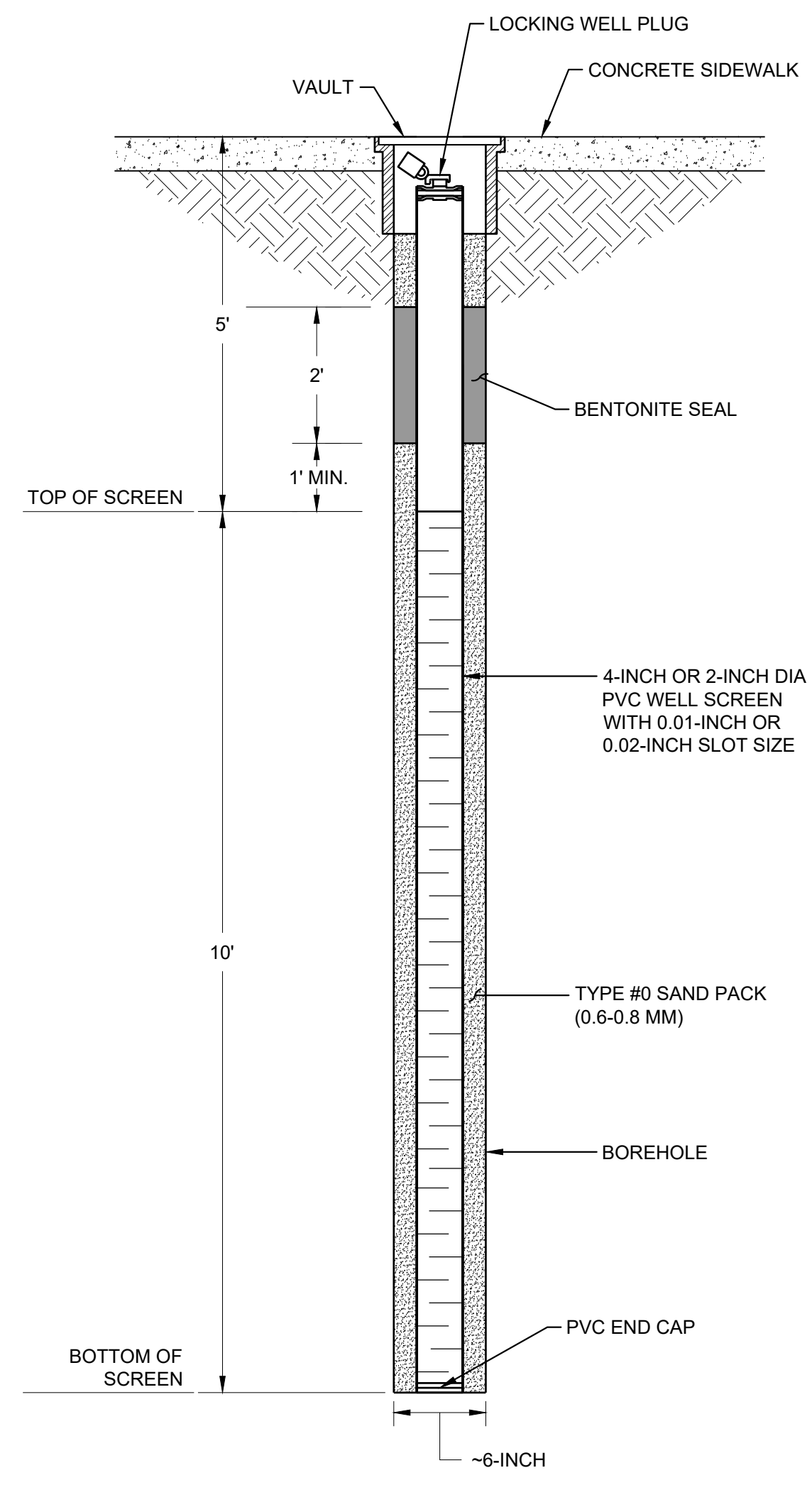
1 LNAPL RECOVERY WELL SCALE: NTS
