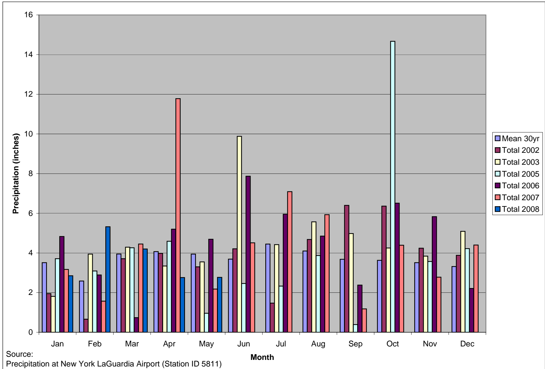
FIGURE 3-3 MONTHLY PRECIPITATION IN LONG ISLAND CITY, NEW YORK
