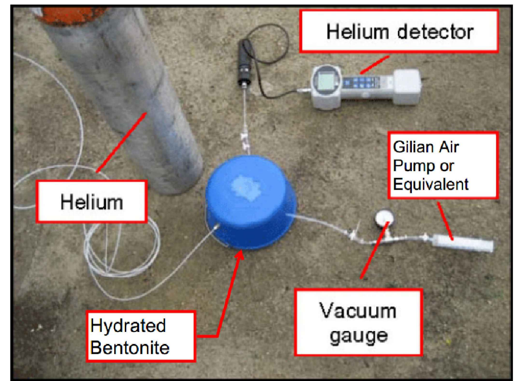
DETAIL 3: TYPICAL LEAK DETECTION SETUP
