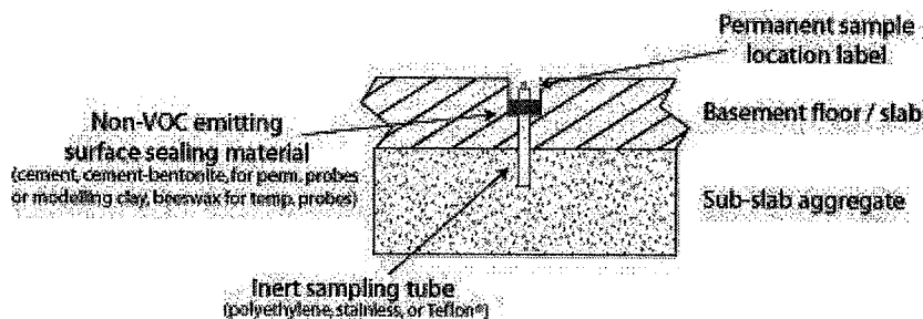
Figure 2.3 Schematic of a sub-slab vapor probe
