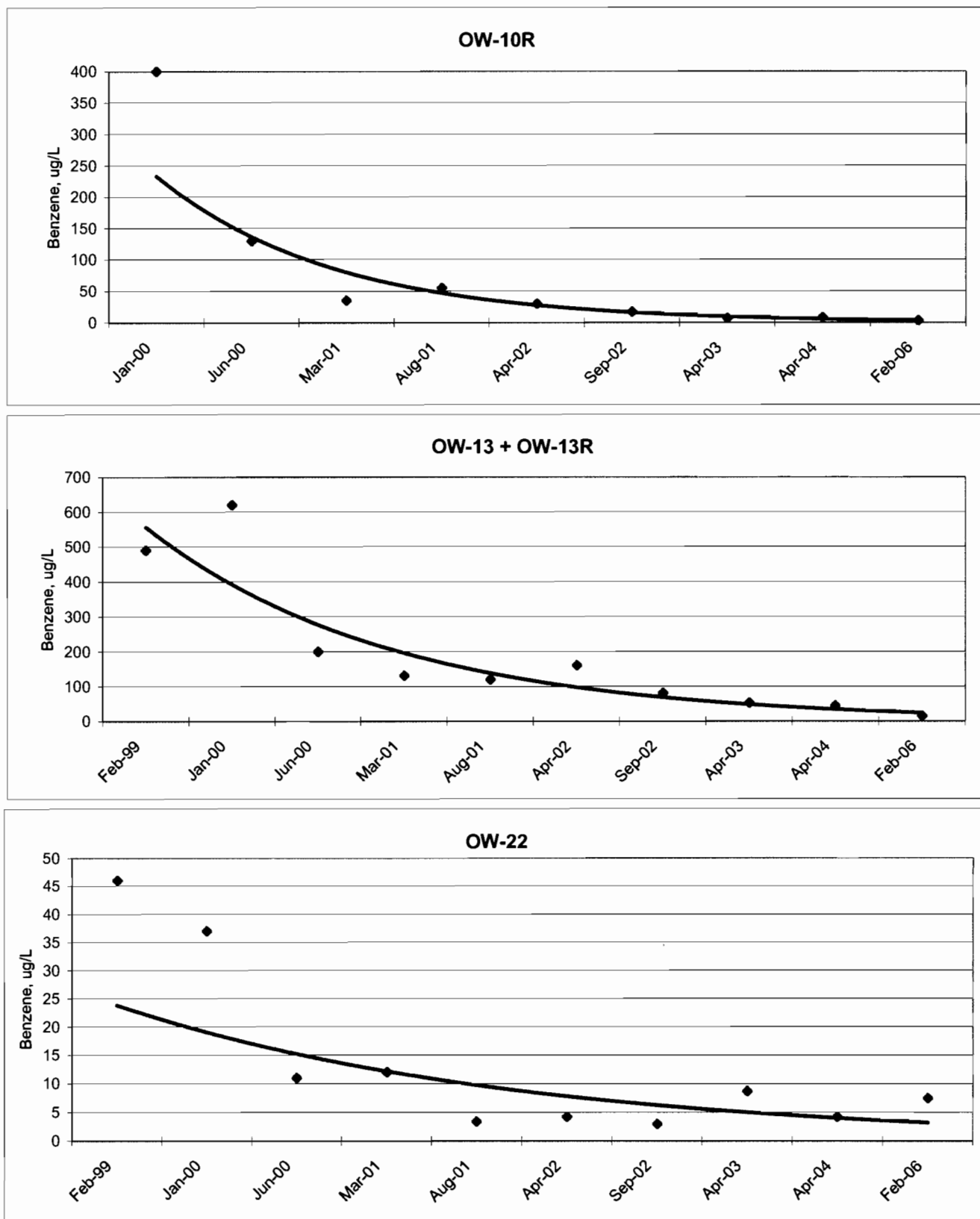
Figure 6 Benzene Concentration Trends Pre-Excavation to April 2004
