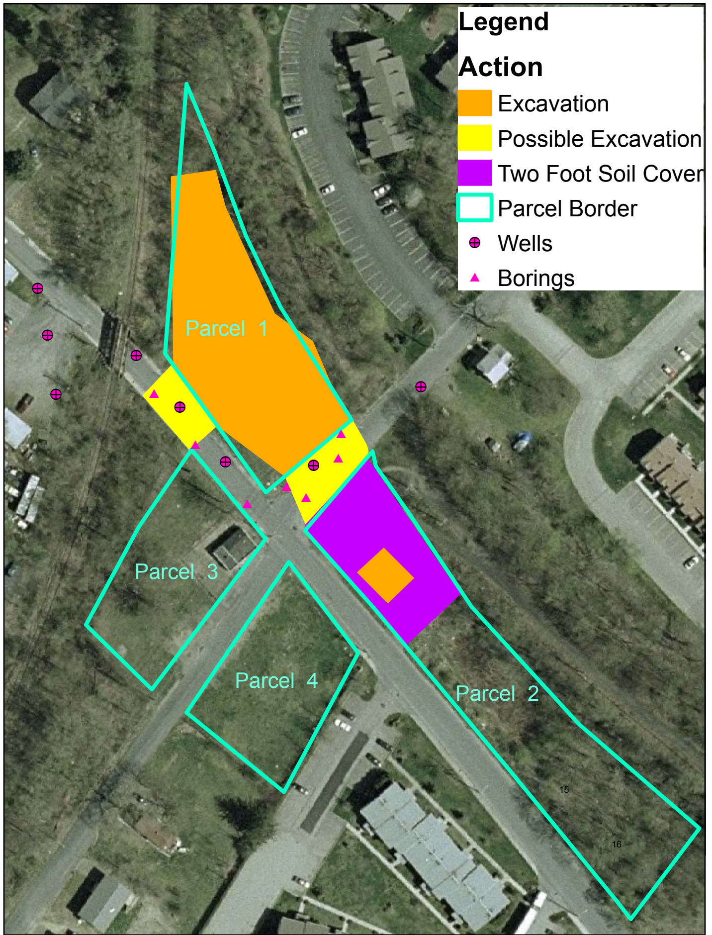
Figure 6 - Selected Remedy Middletown Genung Street MGP Site ROD
