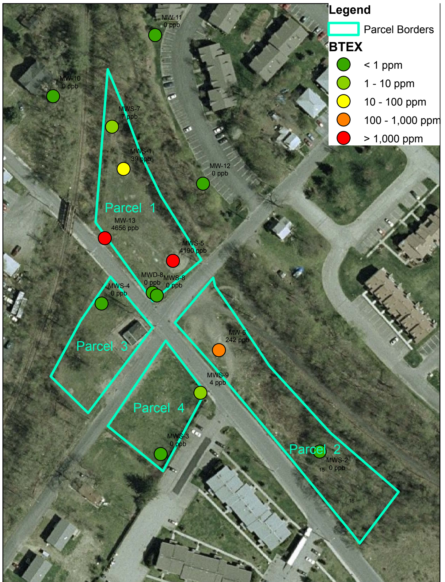
Figure 5 - Extent of Groundwater Contamination Middletown Genung Street MGP Site ROD
