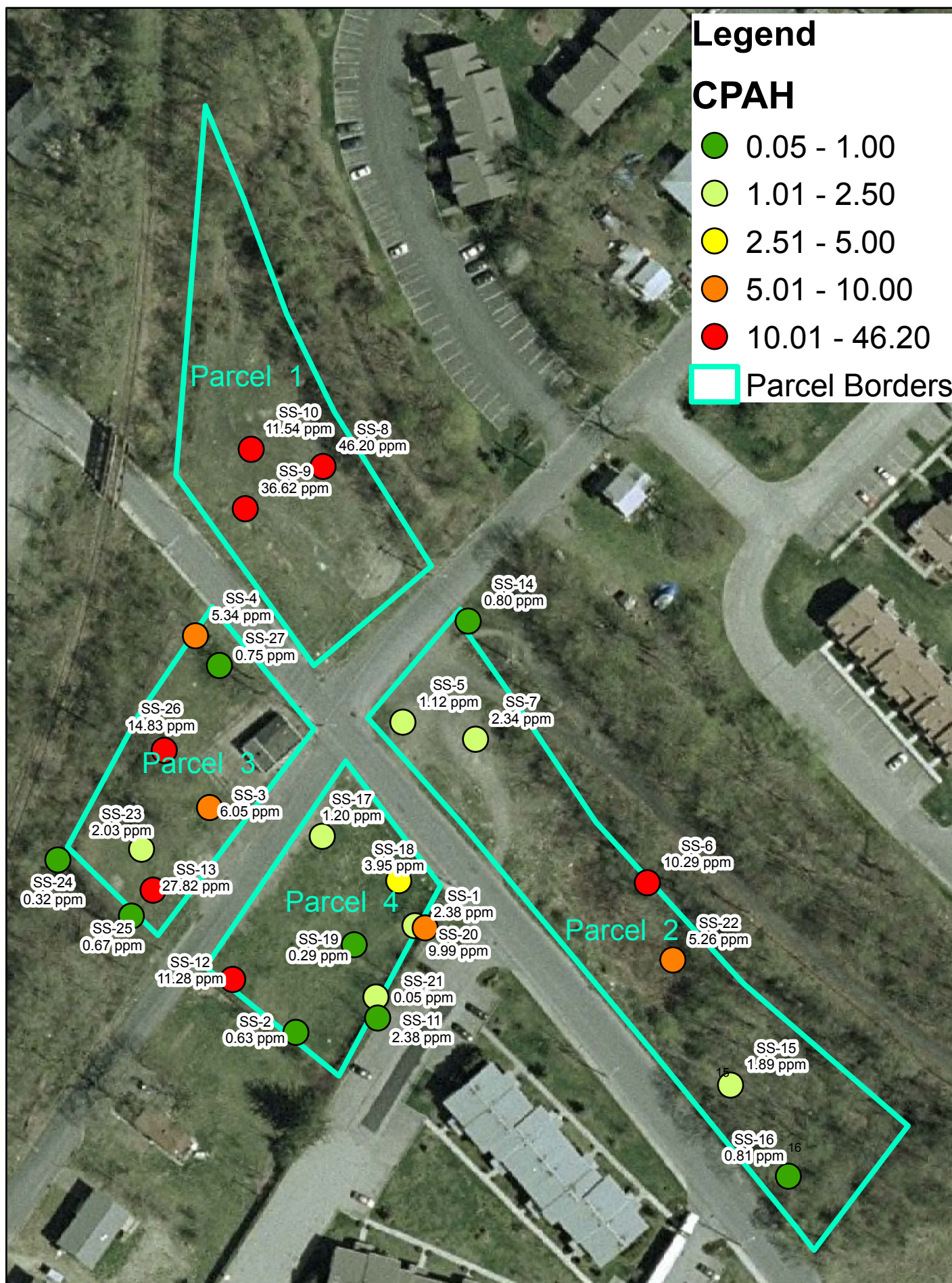
Figure 4 - Surface Soil cPAH Levels Middletown Genung Street MGP Site ROD
