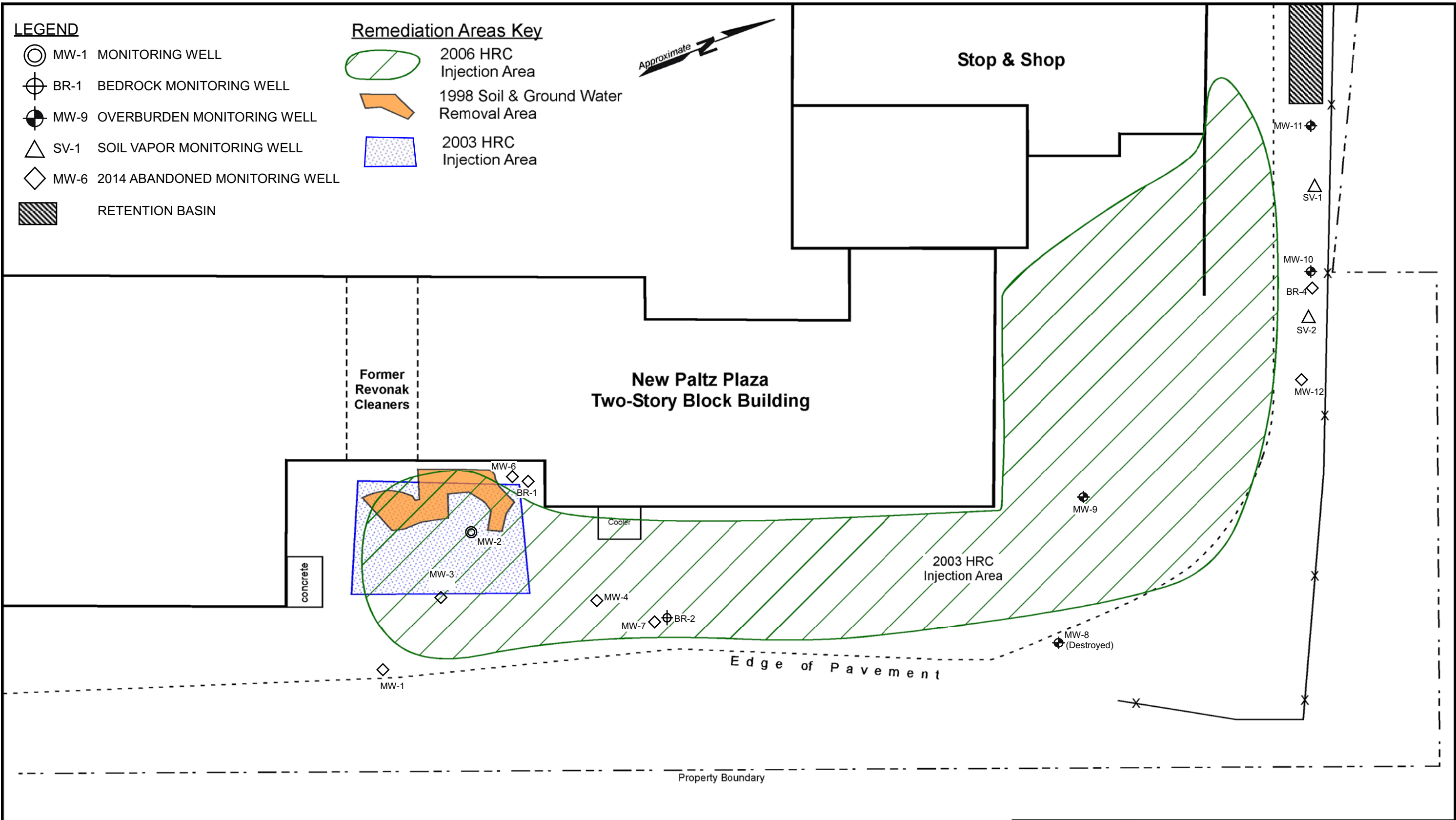
FIGURE 3 Monitoring Well Locations and Remediation Areas
